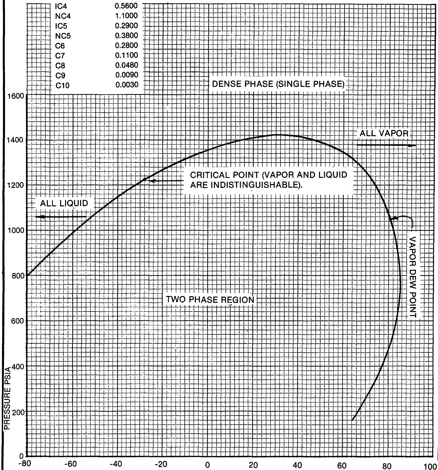
TRANS ALASKA GAS SYSTEM PHASE ENVELOPE PRUDHOE BAY RAW GAS
