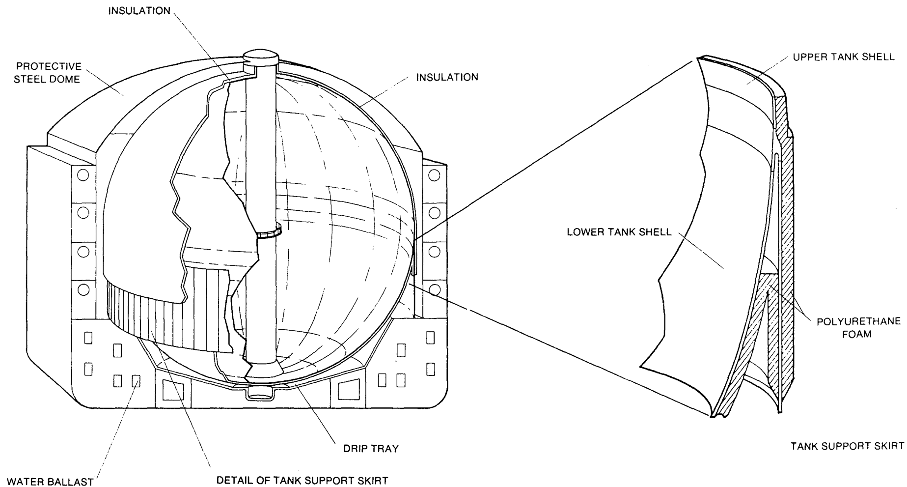
KVAERNER - MOSS SPHERICAL TANK DESIGN FIGURE 5
