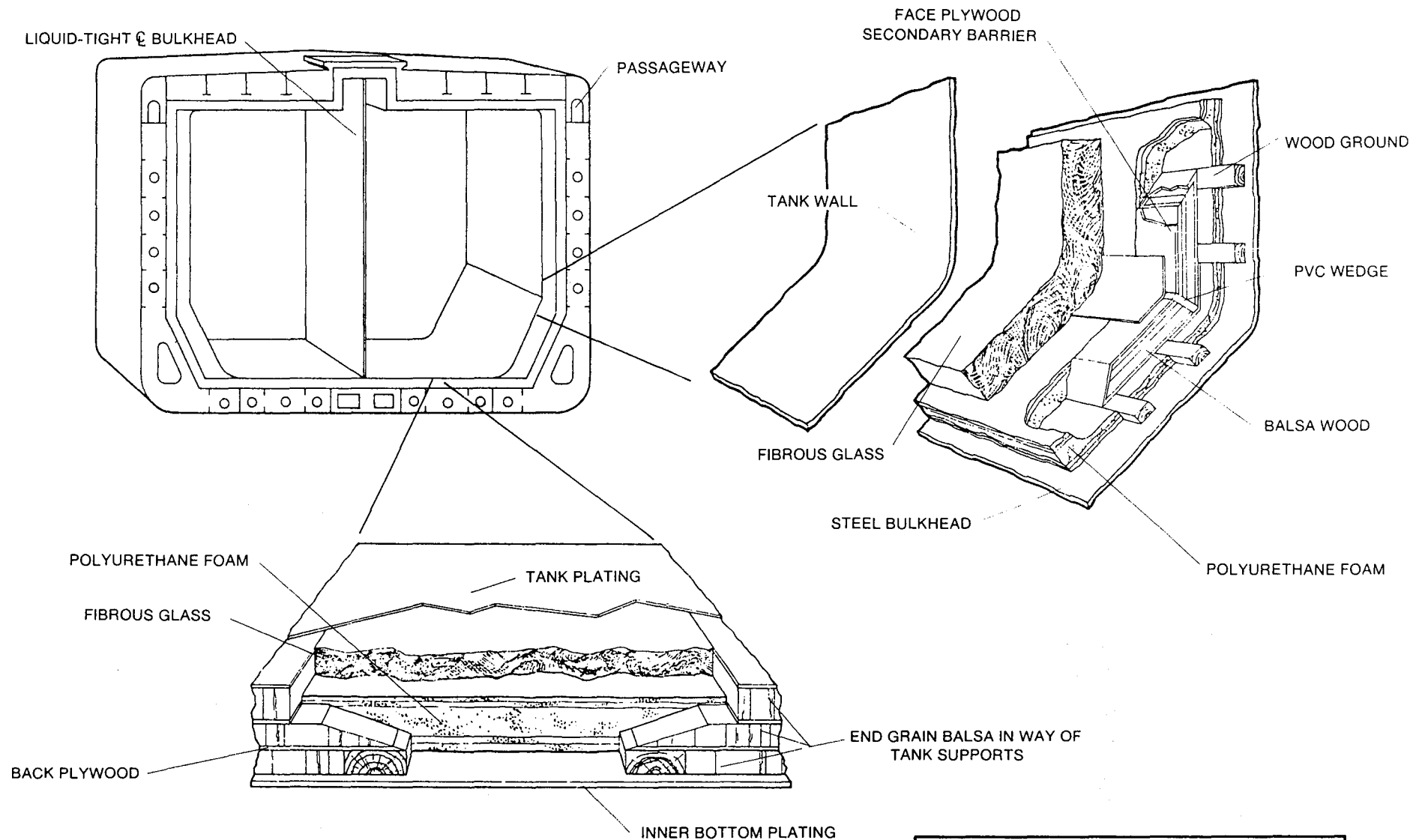
CONCH FREESTANDING TANK DESIGN FIGURE 4
