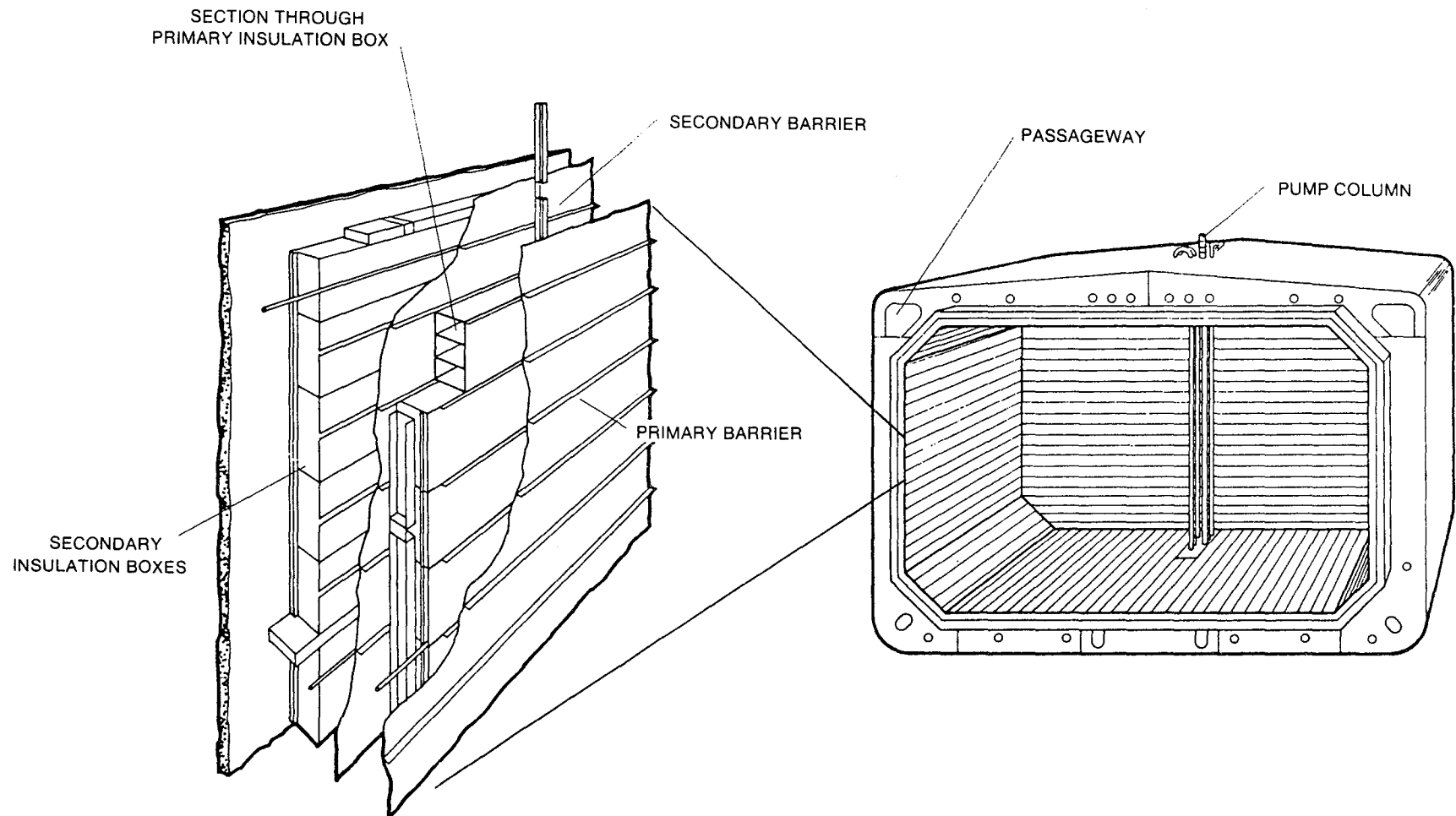
GAZ TRANSPORT MEMBRANE TANK DESIGN FIGURE 6
