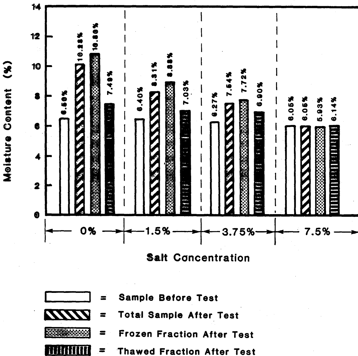
Figure A-3: MOISTURE CONTENT OF TEST SAMPLES
