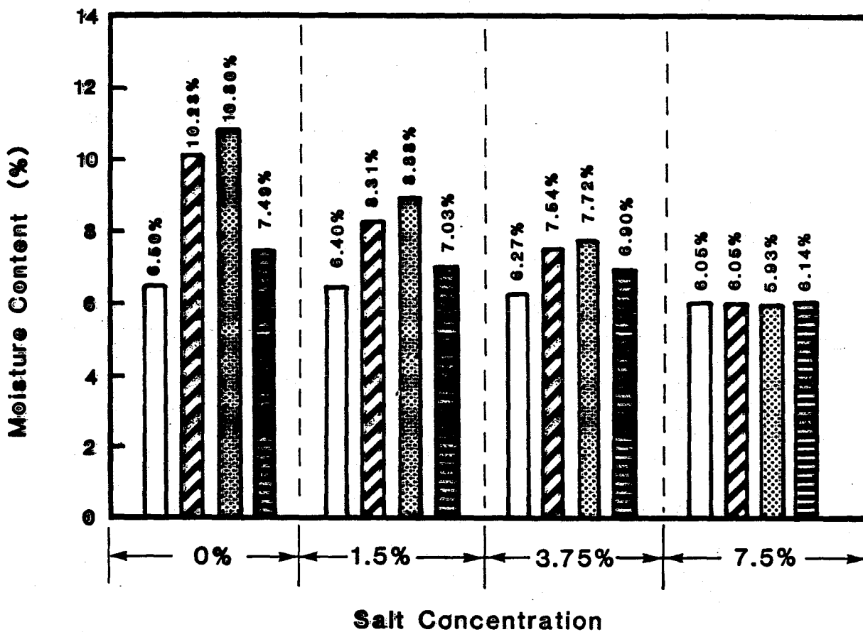
Figure A-3: MOISTURE CONTENT OF TEST SAMPLES
