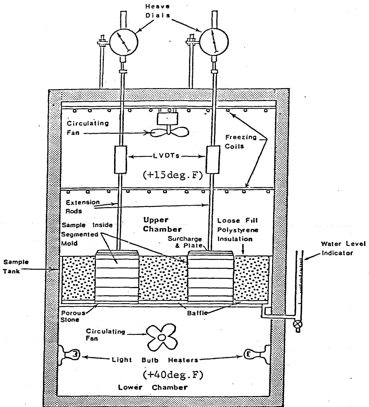
INTERIOR DIAGRAM OF HEAVE TEST CABINET
