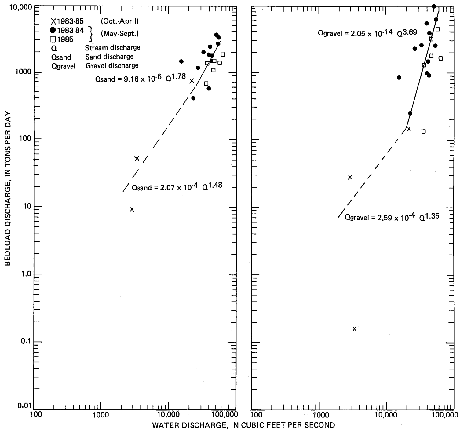
Figure 18.--Bedload-transport curves of sand and gravel for Susitna River below Chulitna River near Talkeetna (sum of right and left channels), 1983-85.
