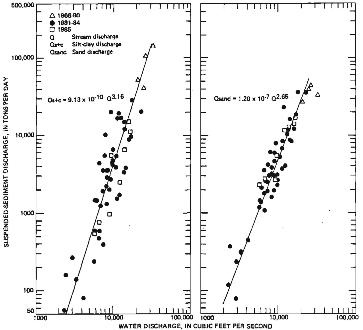
Figure 5.—Sediment-transport curves of suspended silt-clay and sand discharge for Talkeetna River near Talkeetna, May to September, 1981-85.
