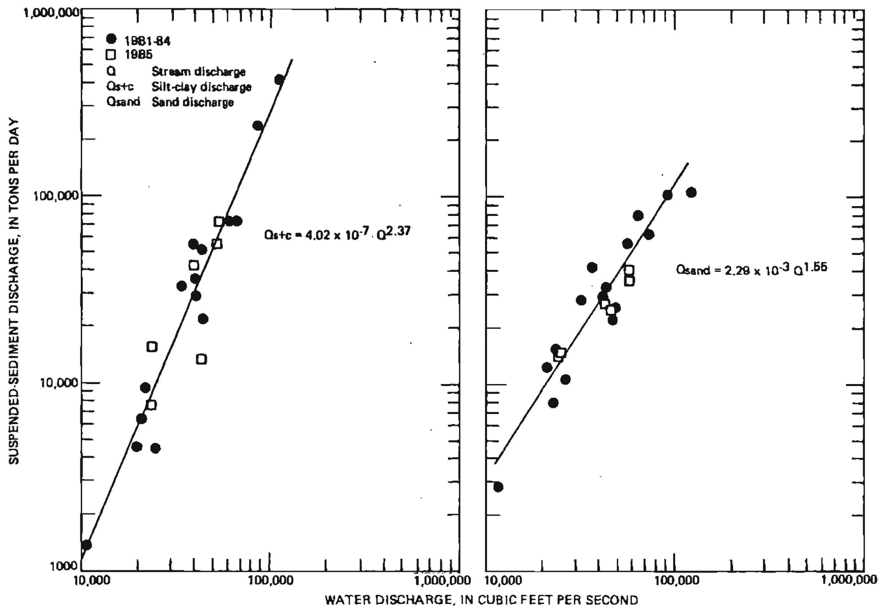
Figure 7.--Sediment-transport curves of suspended silt-clay and sand discharge for Yentna River near Sugitna Station, May to September, 1981-85.
