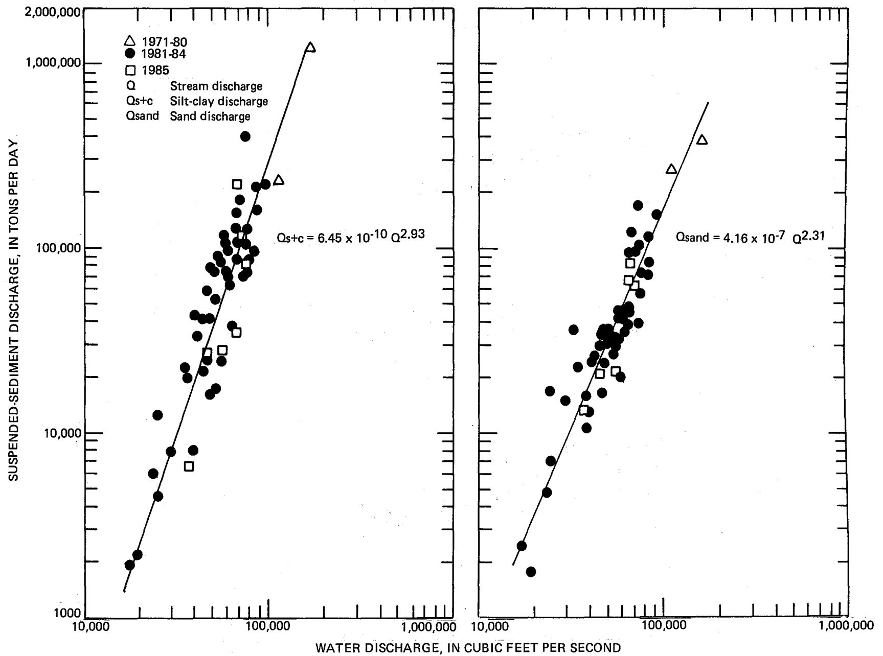
Figure 6.--Sediment-transport curves of suspended silt-clay and sand discharge for Susitna River at Sunshine, May to September, 1981-85.
