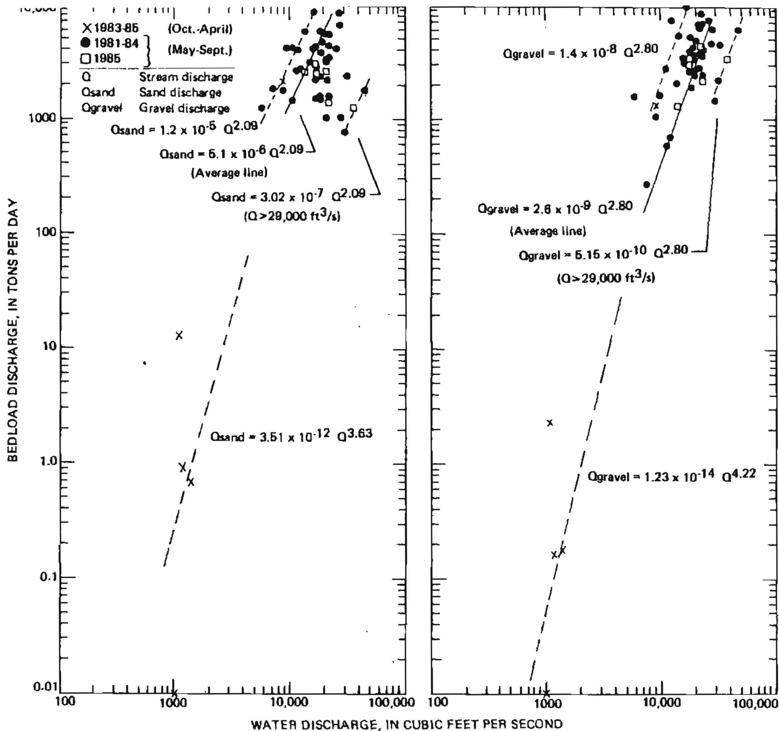
Figure 17.—Bedload-transport curves of sand and gravel for Chulitna River below canyon near Talkeetna, May to September, 1981-85 and October to April, 1983-85.
