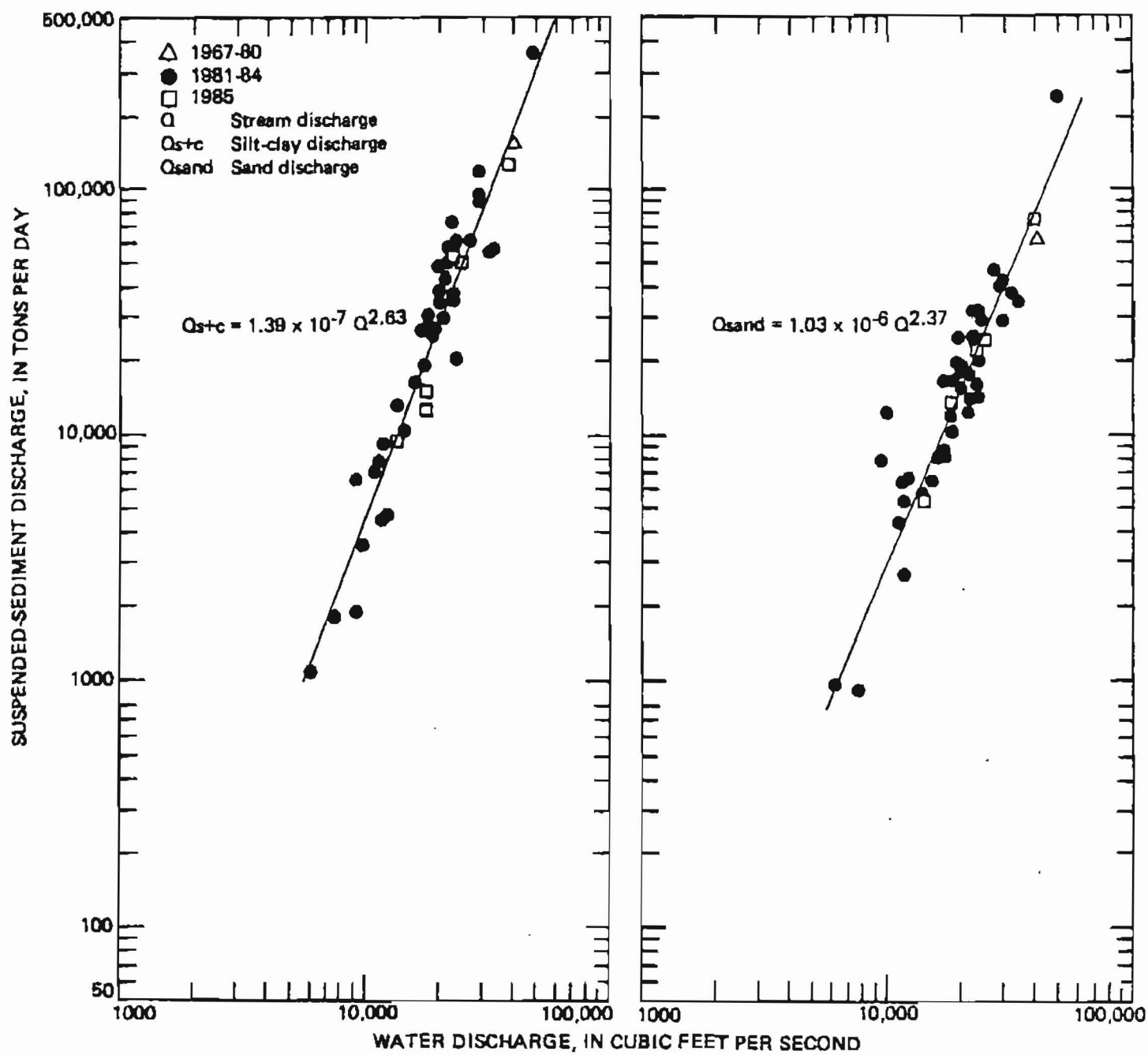
Figure 3.—Sediment-transport curves of suspended silt-clay and sand discharge for Chulitna River below canyon near Talkeetna, May to September, 1981-85.
