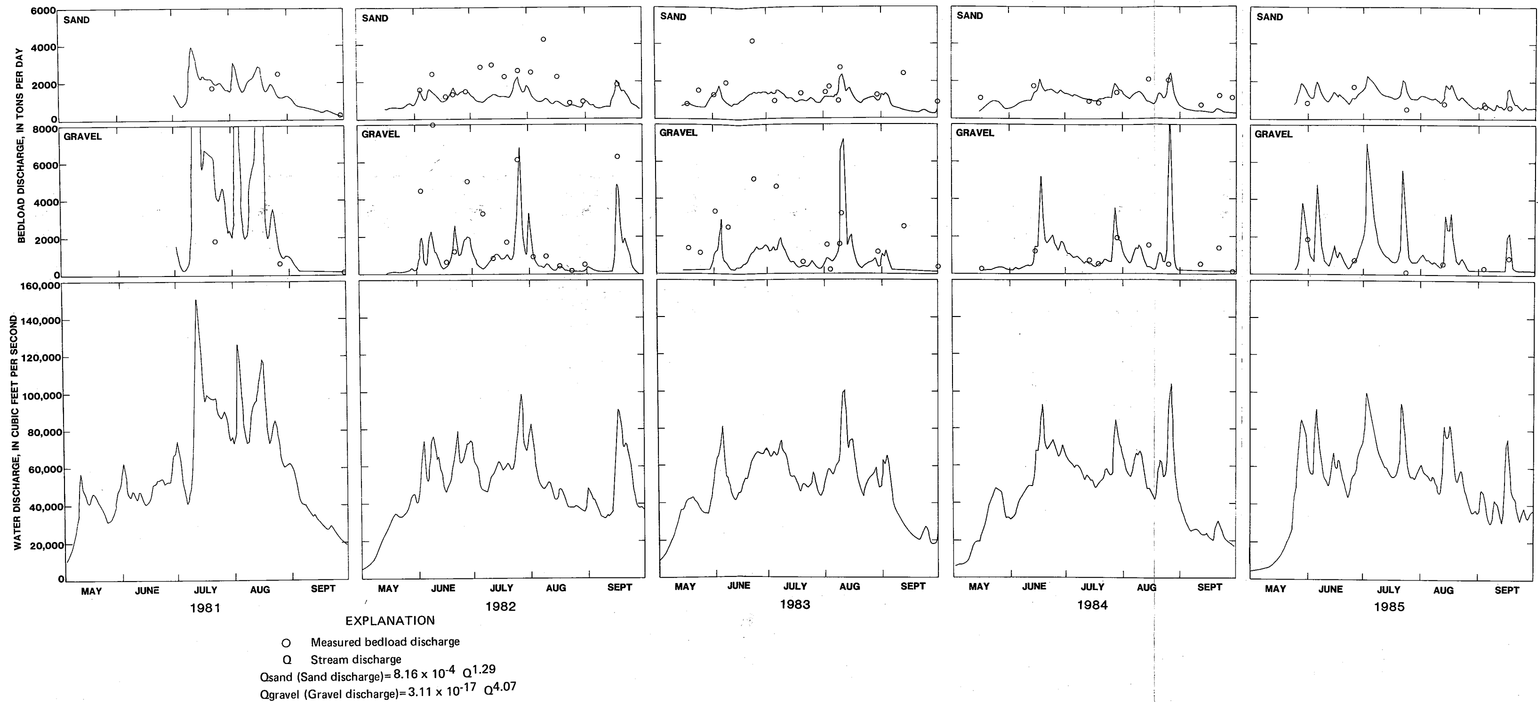
Figure 26.--Variability of water and bedload discharge for Susitna River at Sunshine, May to September, 1981-85.
