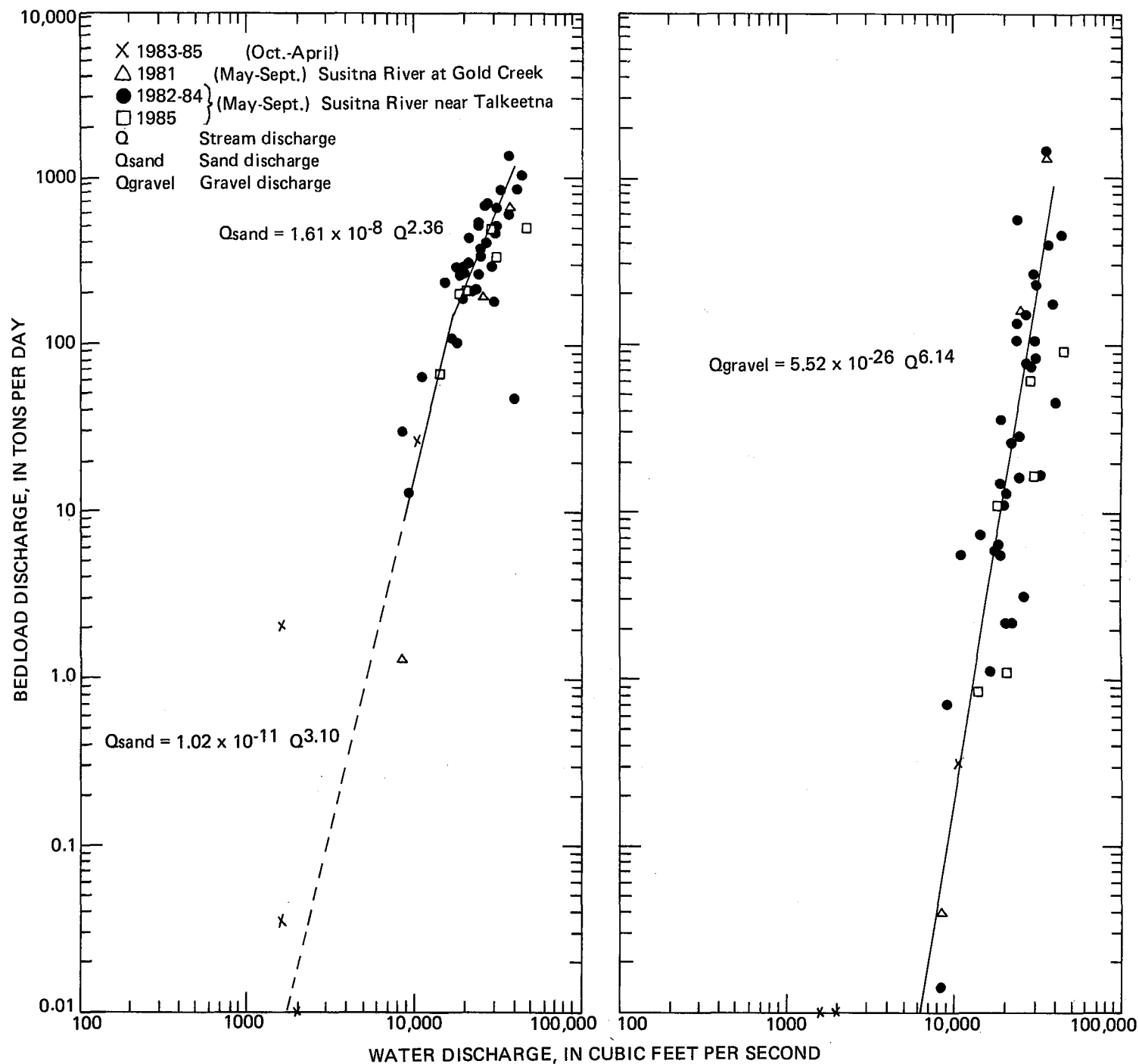
Figure 16.--Bedload-transport curves of sand and gravel for Susitna River near Talkeetna, May to September, 1982-85 and October to April, 1983-85.
