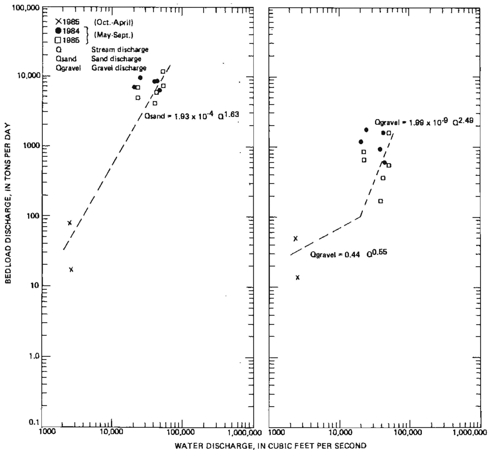
Figure 21.--Bedload-transport curves of sand and gravel for Yentna River near Susitna Station, May to September, 1984-85 and October to April, 1985.
