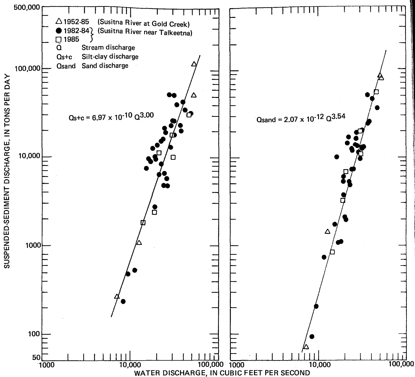
Figure 2.--Sediment-transport curves of suspended silt-clay and sand discharge for Susitna River near Talkeetna, May to September, 1981-85.
