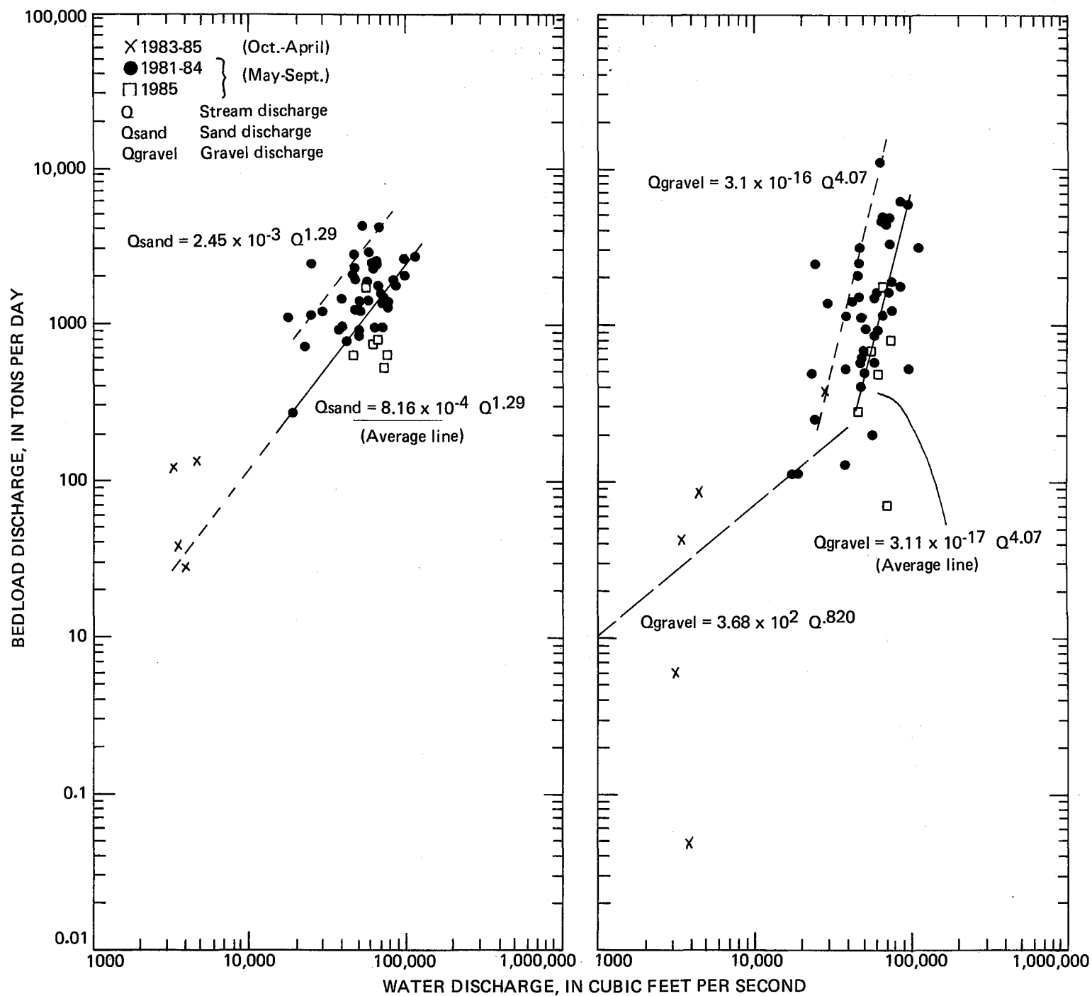
Figure 20.--Bedload-transport curves of sand and gravel for Susitna River at Sunshine, May to September, 1981-85 and October to April, 1983-85.
