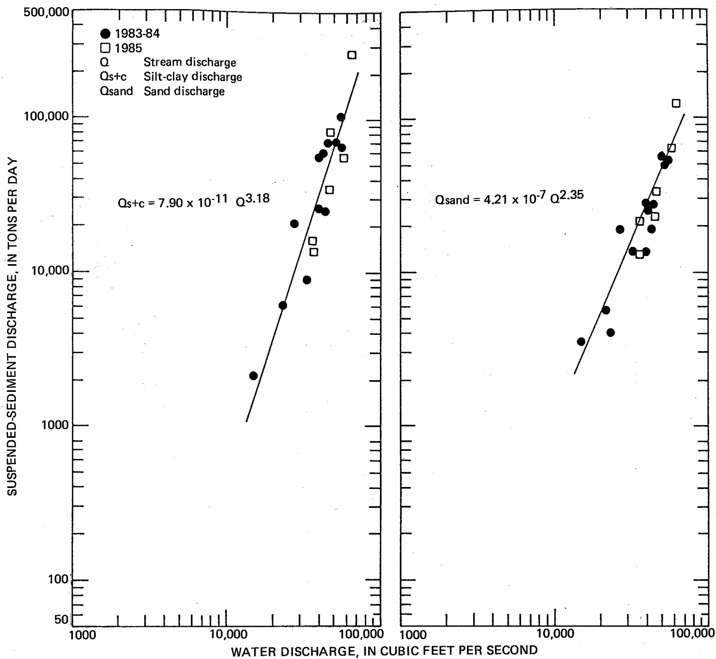
Figure 4.--Sediment-transport curves of suspended silt-clay and sand discharge for Susitna River below Chulitna River near Talkeetna (sum of right and left channels), May to September, 1983-85.
