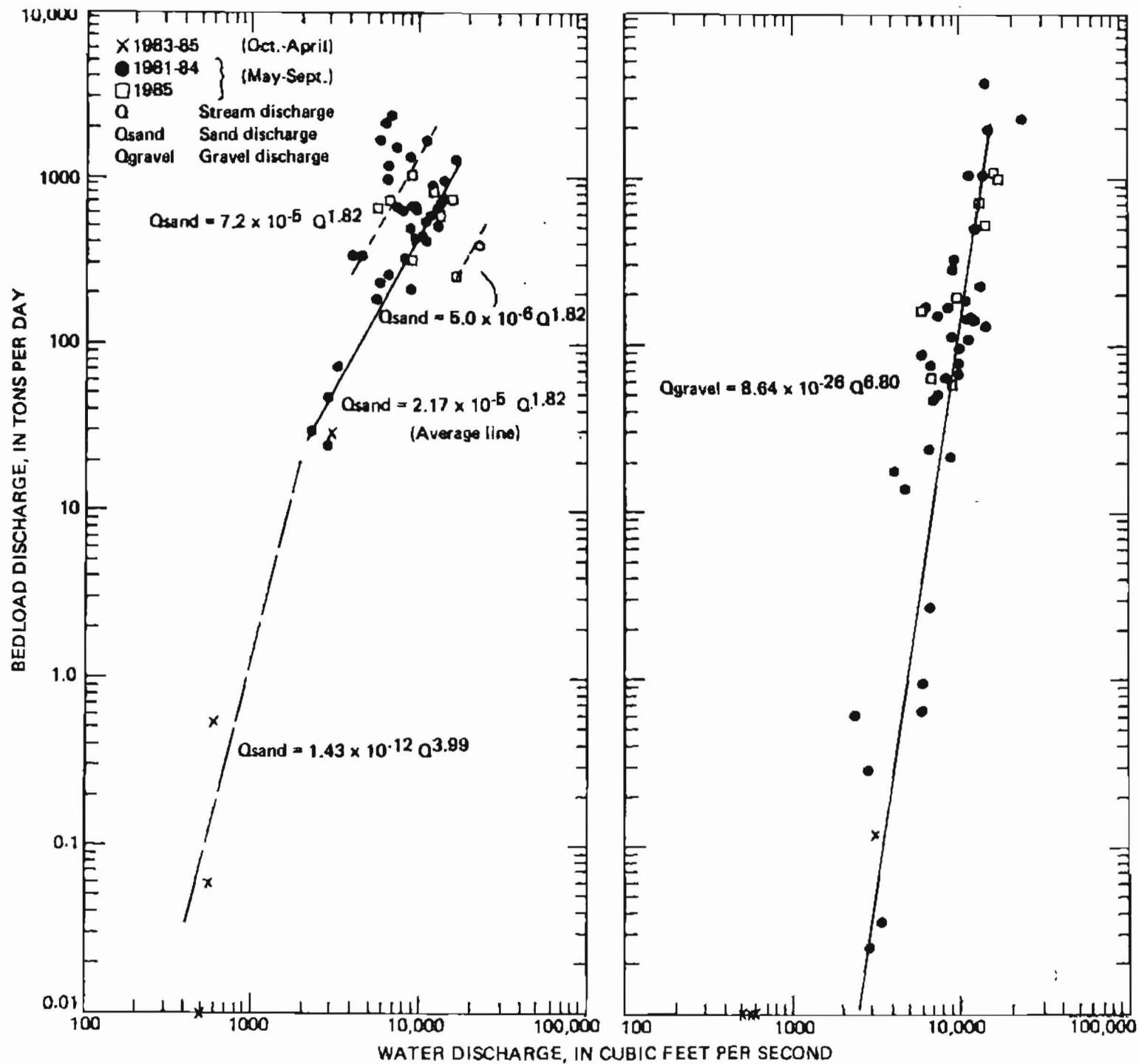
Figure 19.--Bedload-transport curves of sand and gravel for Talkeetna River near Talkeetna, May to September, 1981-85 and October to April, 1983-85.
