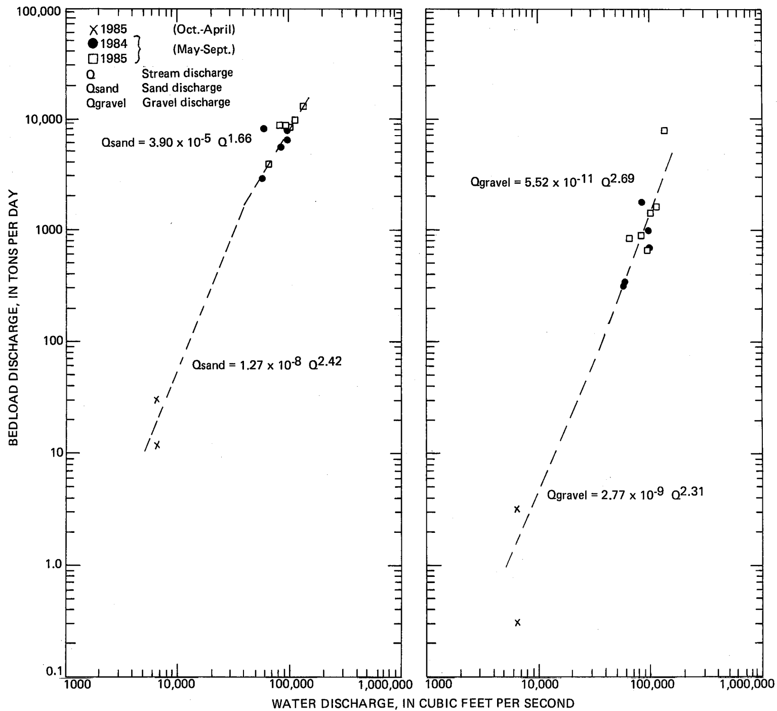
Figure 22.--Bedload-transport curves of sand and gravel for Susitna River at Susitna Station, 1984-85 and October to April, 1985.
