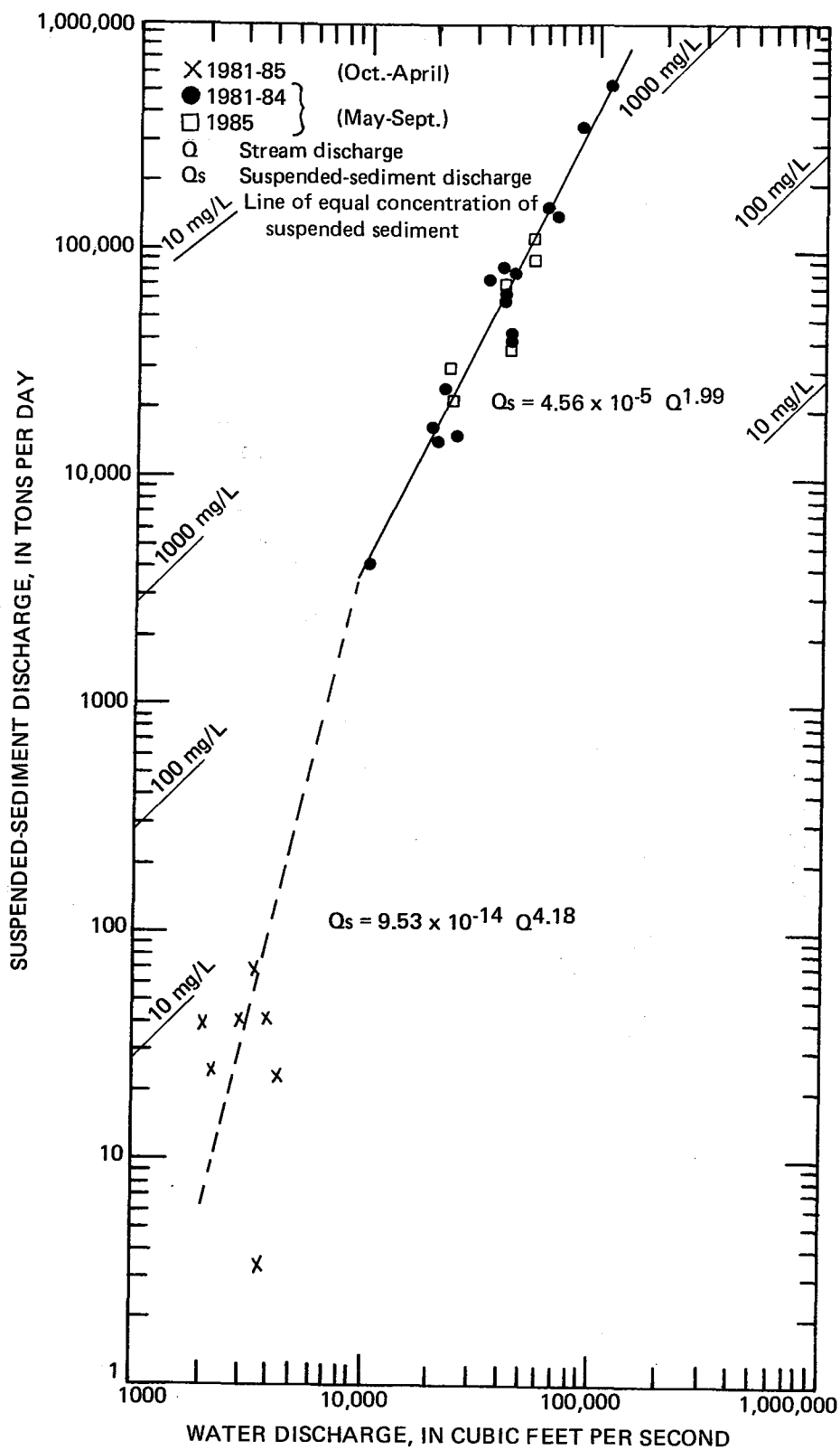
Figure 14.--Relation of mean suspended-sediment concentration and discharge to water discharge for Yentna River near Susitna Station, 1981-85.
