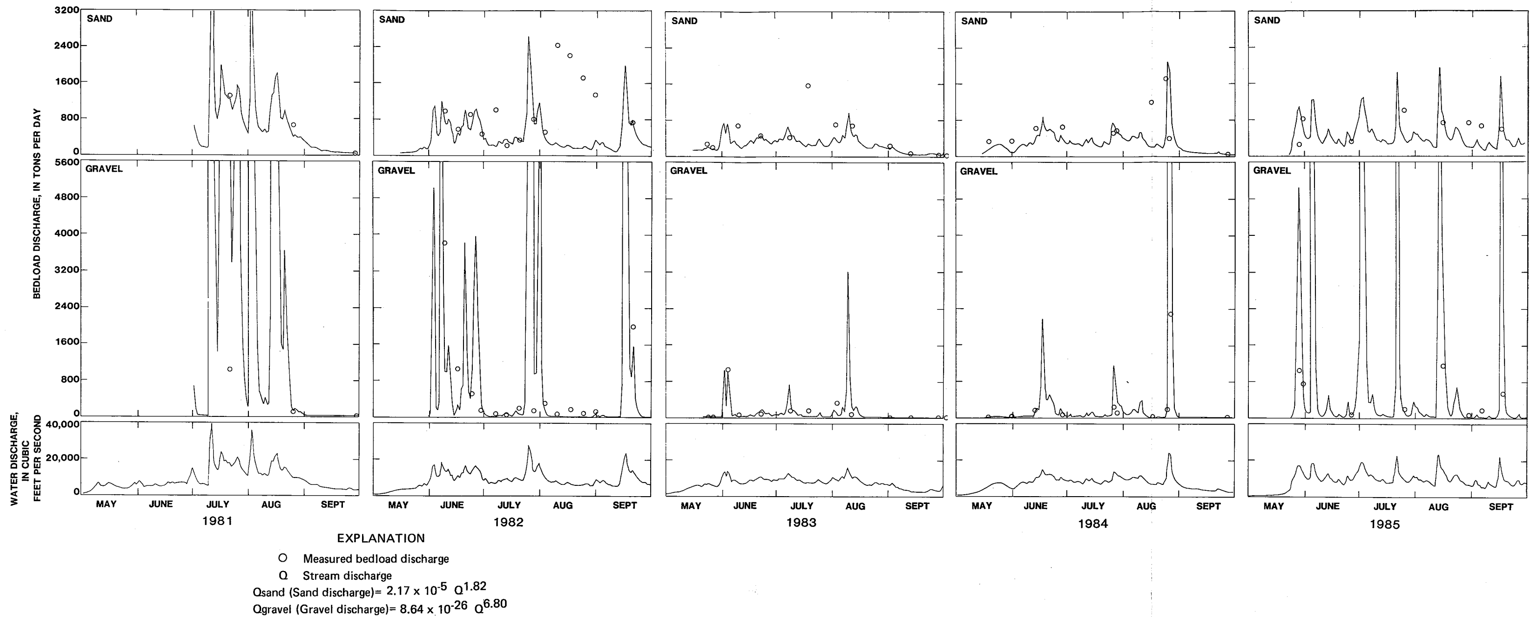
Figure 25.--Variability of water and bedload discharge for Talkeetna River near Talkeetna, May to September, 1981-85.
