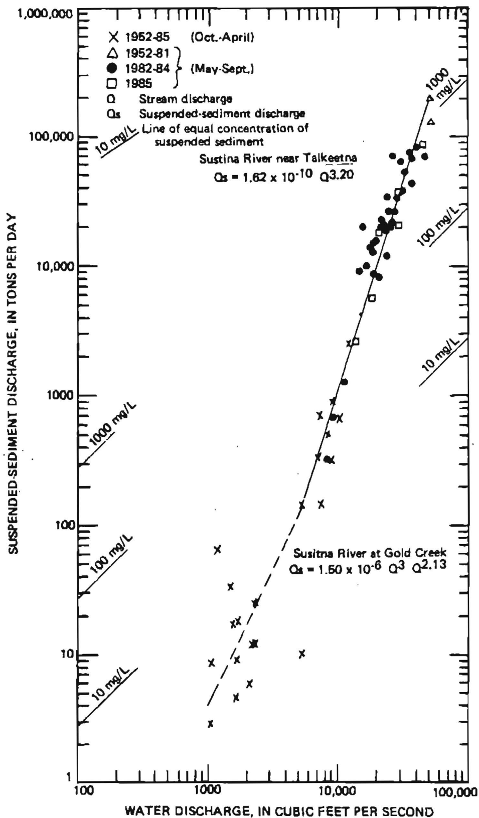
Figure 9.—Relation of mean suspended-sediment concentration and discharge to water discharge for Susitna River near Talkeetna, May to September, 1981-85 and Susitna River at Gold Creek, October to April, 1952-85.
