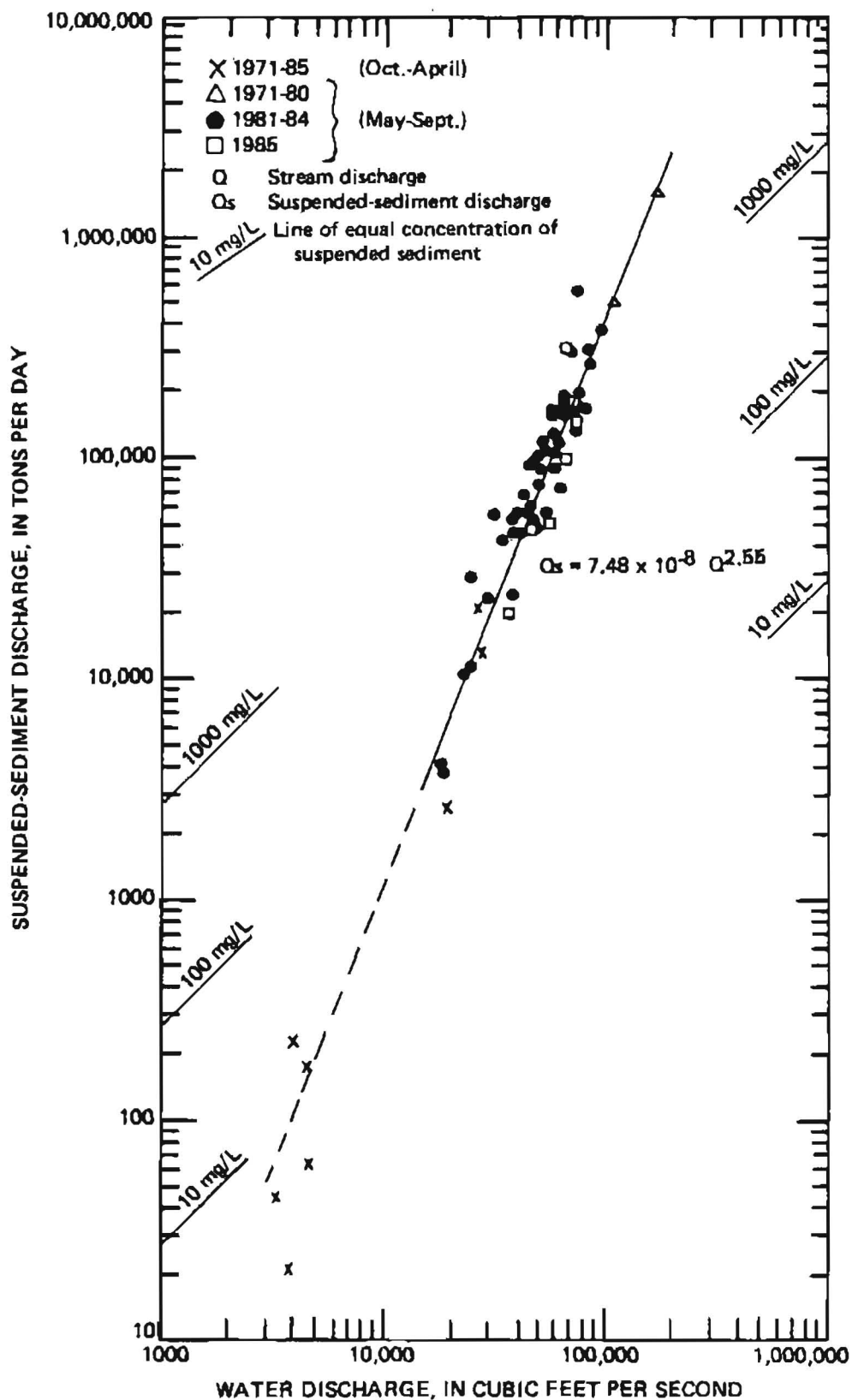
Figure 13.—Relation of mean suspended-sediment concentration and discharge to water discharge for Susitna River at Sunshine, 1981-85.
