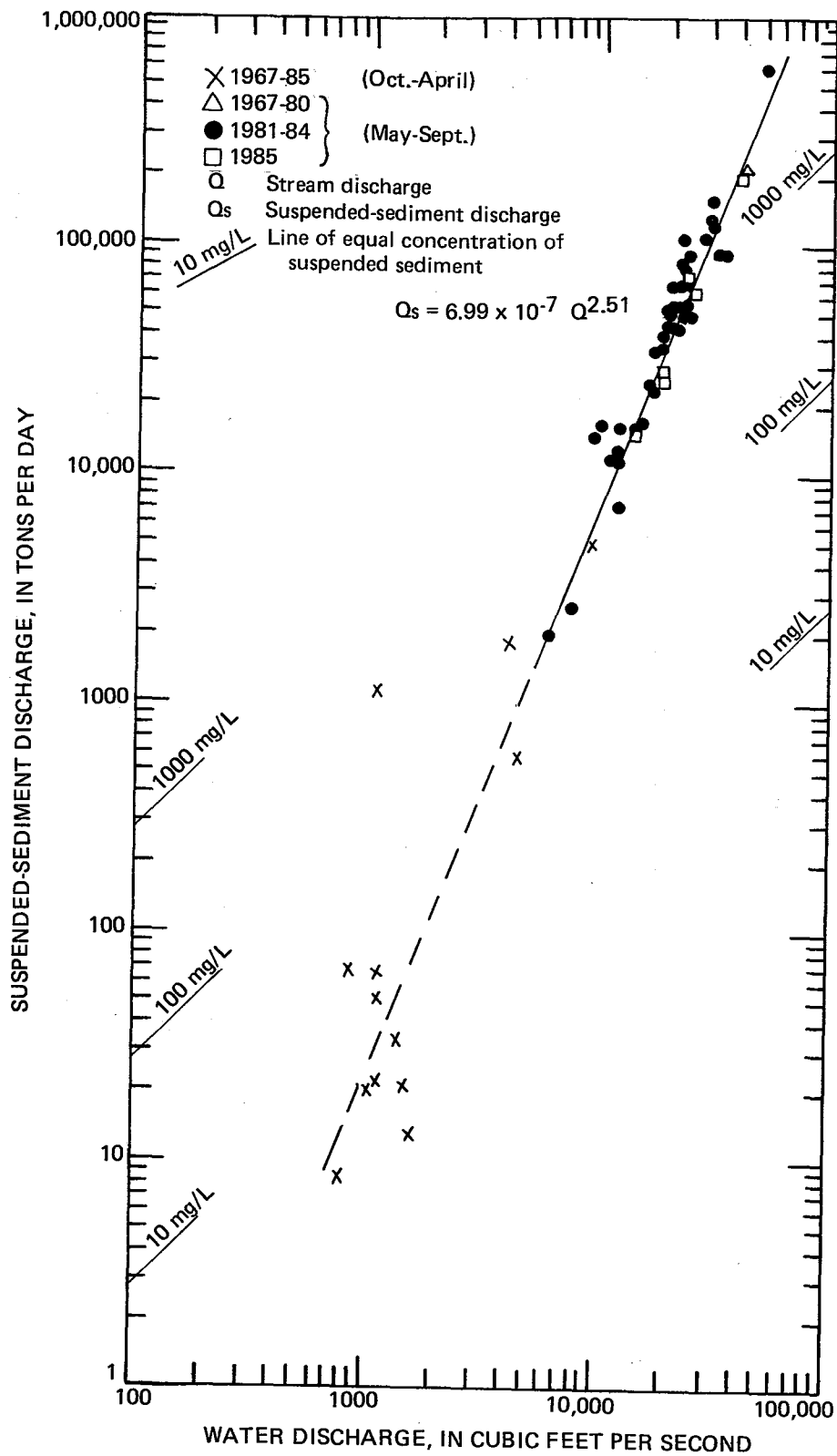
Figure 10.—Relation of mean suspended-sediment concentration and discharge to water discharge for Chulitna River below canyon near Talkeetna, 1981-85.
