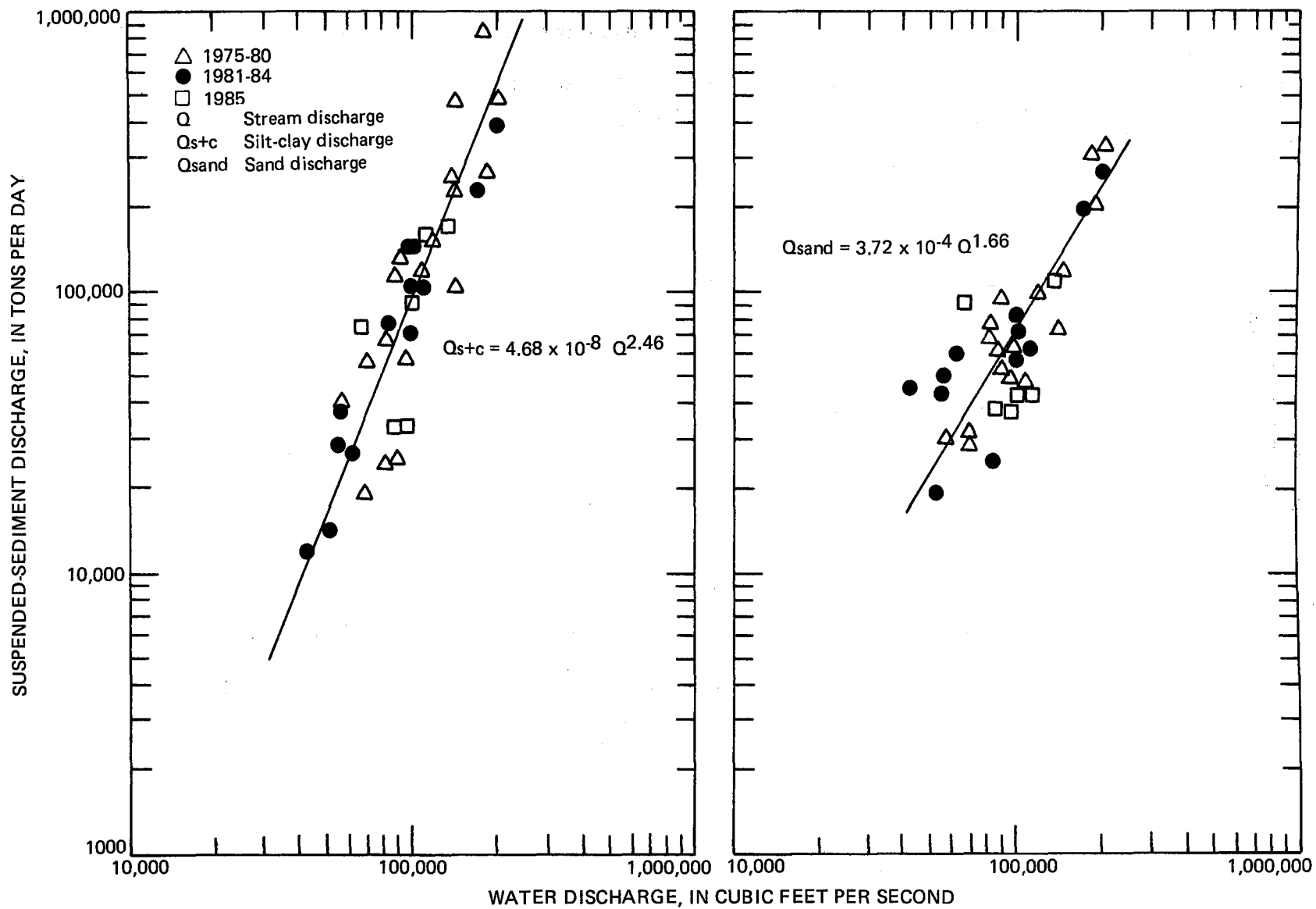
Figure 8.--Sediment-transport curves of suspended silt-clay and sand discharge for Susitna River at Susitna Station, May to September, 1981-85.
