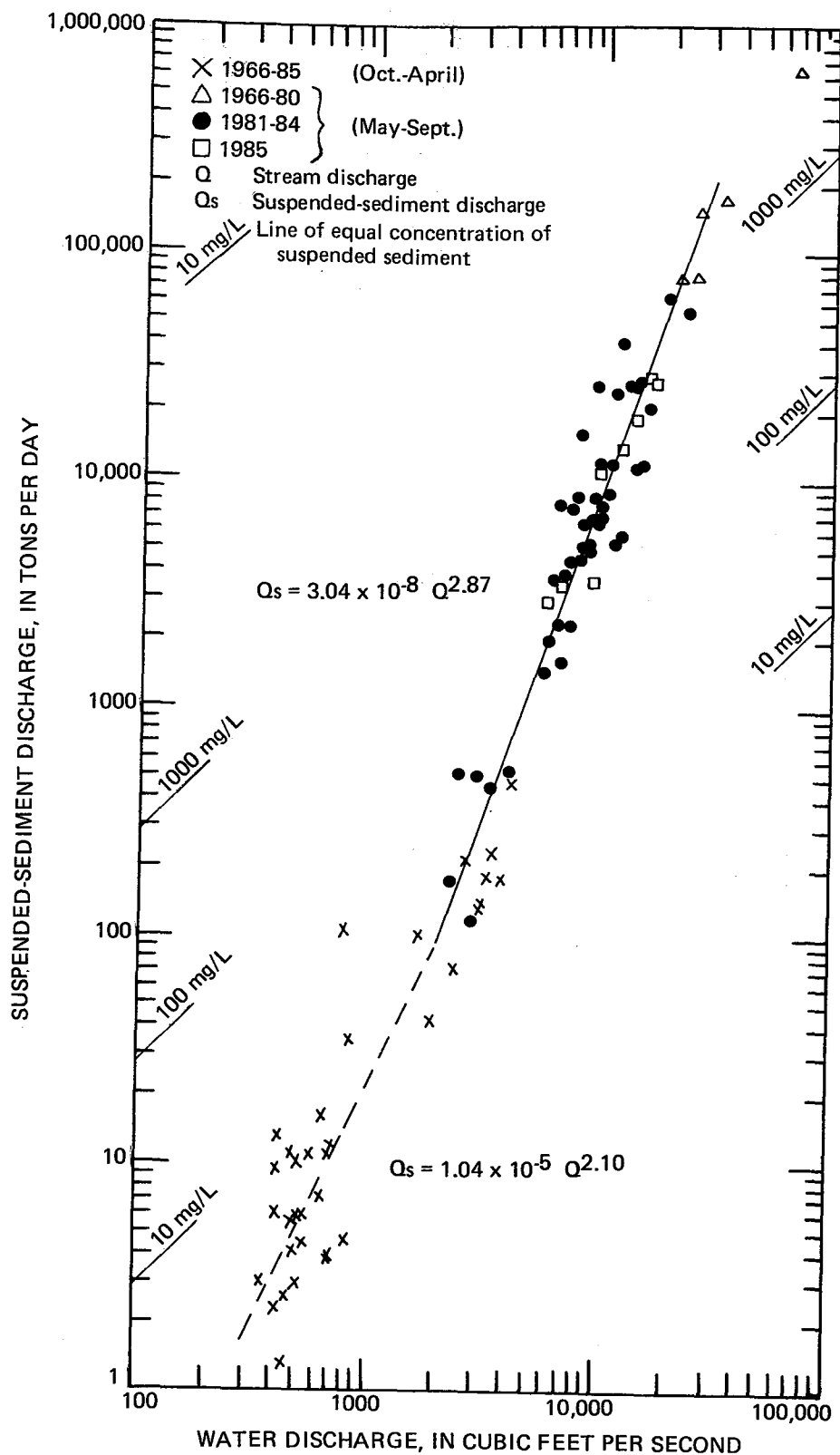
Figure 12.--Relation of mean suspended-sediment concentration and discharge to water discharge for Talkeetna River near Talkeetna, May to September, 1981-85 and October to April, 1966-85.
