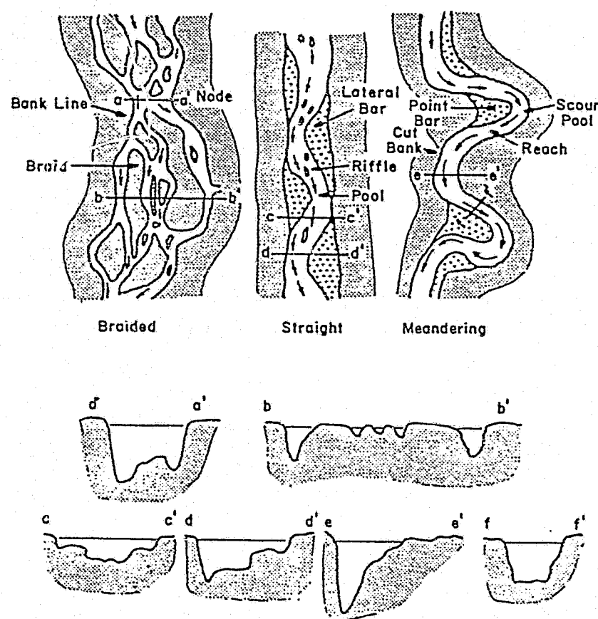
Figure 5. River Channel Patterns (from Richardson et al, 1975).
