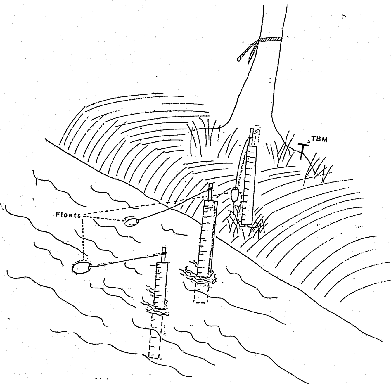
Figure 9. Staff Gage Installation.
