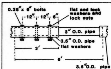
a) LEG JOINT (side view)
