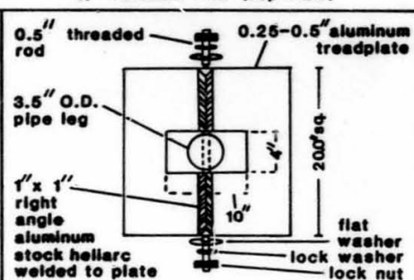
b) TUNDRA PAD (top view)
