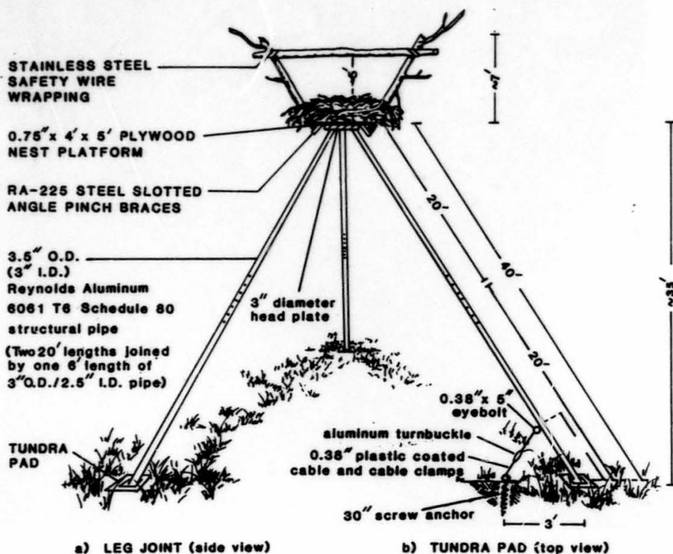
a) LEG JOINT (side view)
