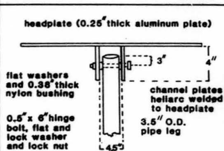
d) HEADPLATE/LEG HINGE (side view)
