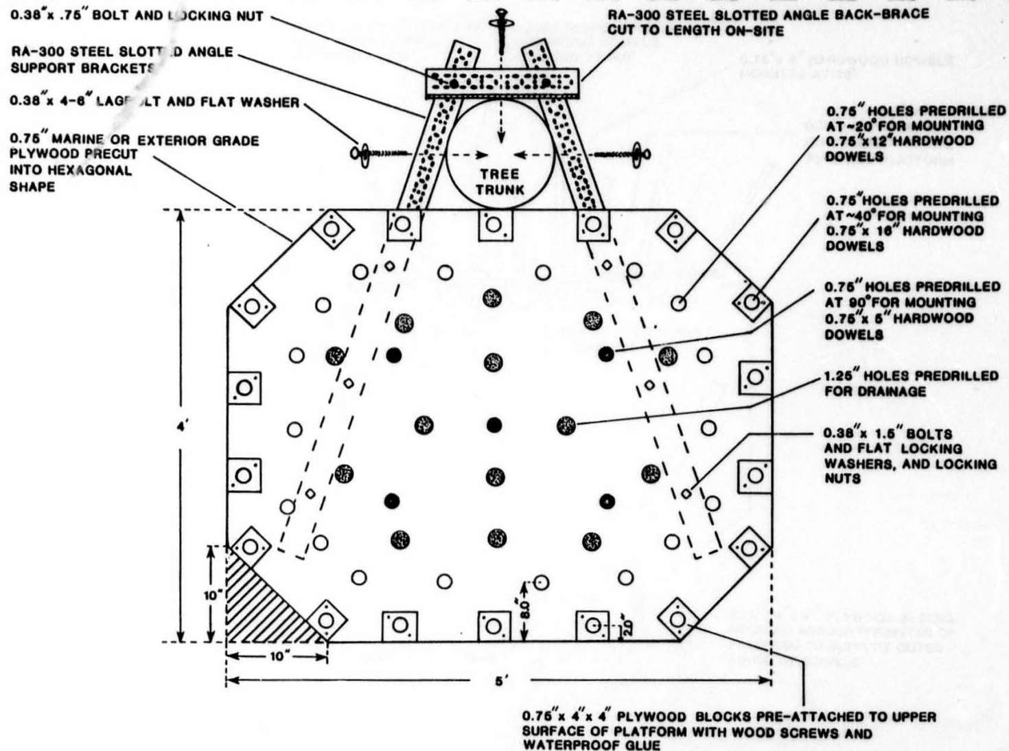
Figure 2. Overhead view of hexagonal nesting platform.
