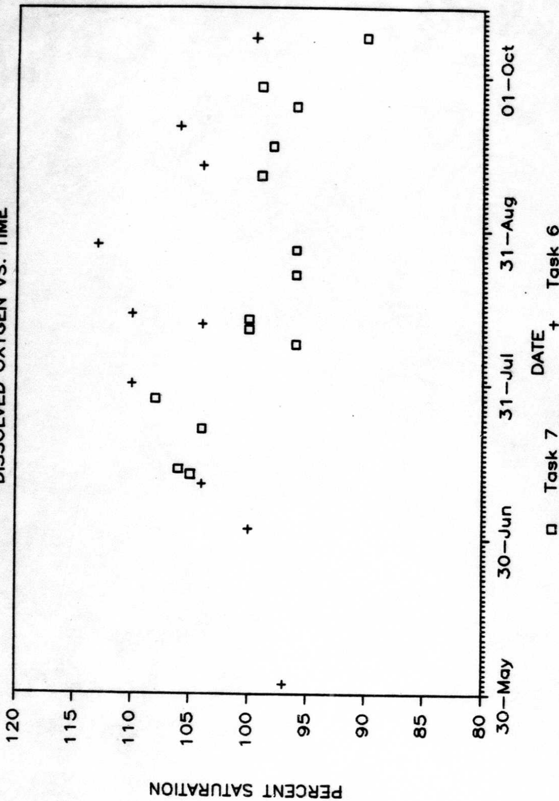
Appendix Figure 39. Dissolved oxygen percent saturation levels from upstream of Portage Creek (RM 149.4).
