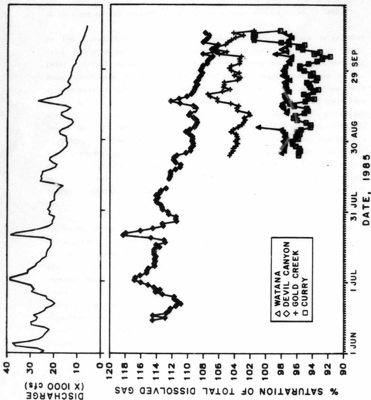
Figure 10. A comparison of percent saturation of total dissolved gas for the four continuous dissolved gas monitoring stations
