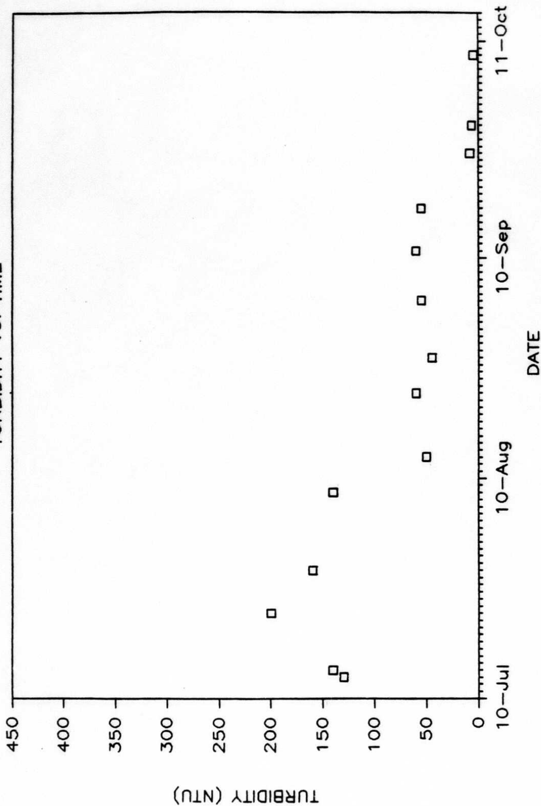
Appendix Figure 20. Weekly measurements of turbidity from upstream of Portage Creek (RM 149.4).
