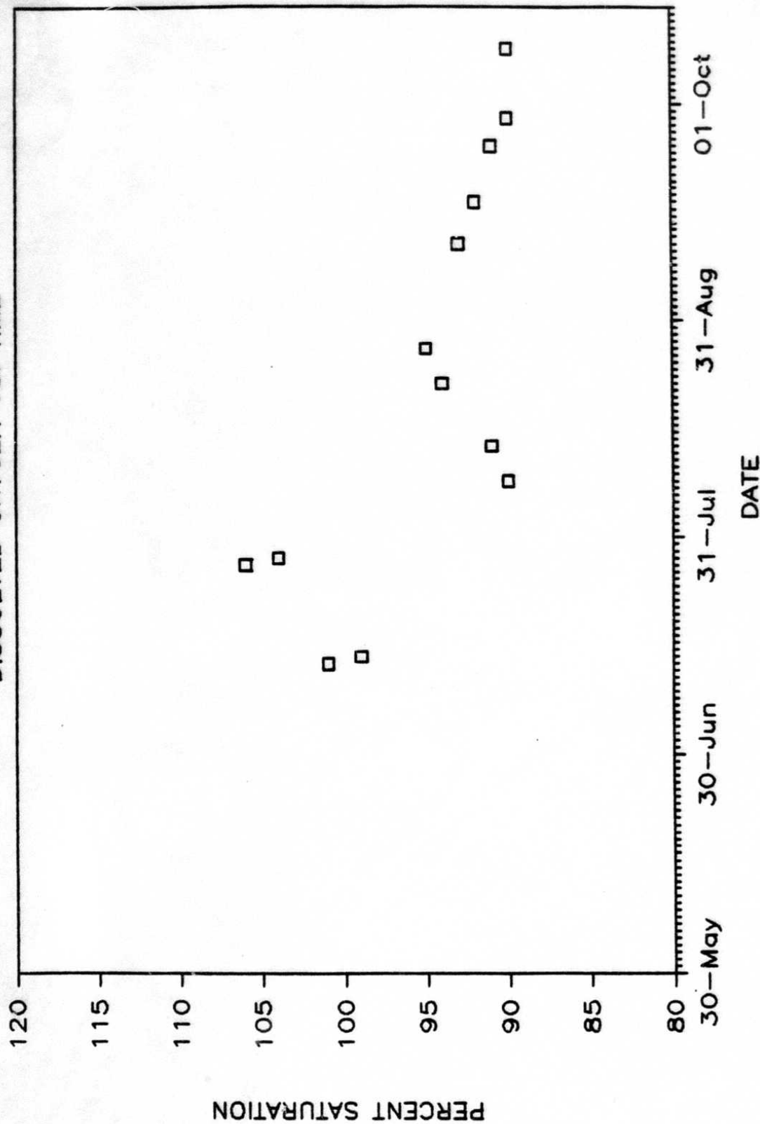
Appendix Figure 35. Dissolved oxygen percent saturation levels from upstream of the Parks Highway Bridge (RM 86.2).
