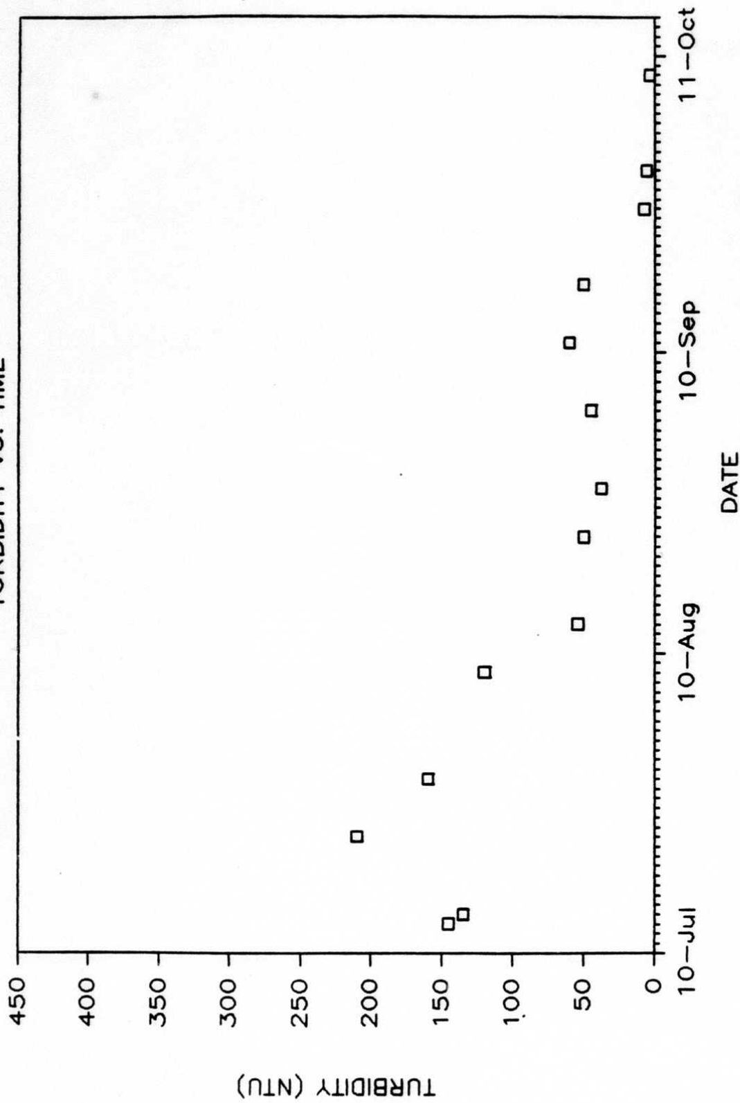
Appendix Figure 18. Weekly measurements of turbidity from the Curry Station (RM 120.7).
