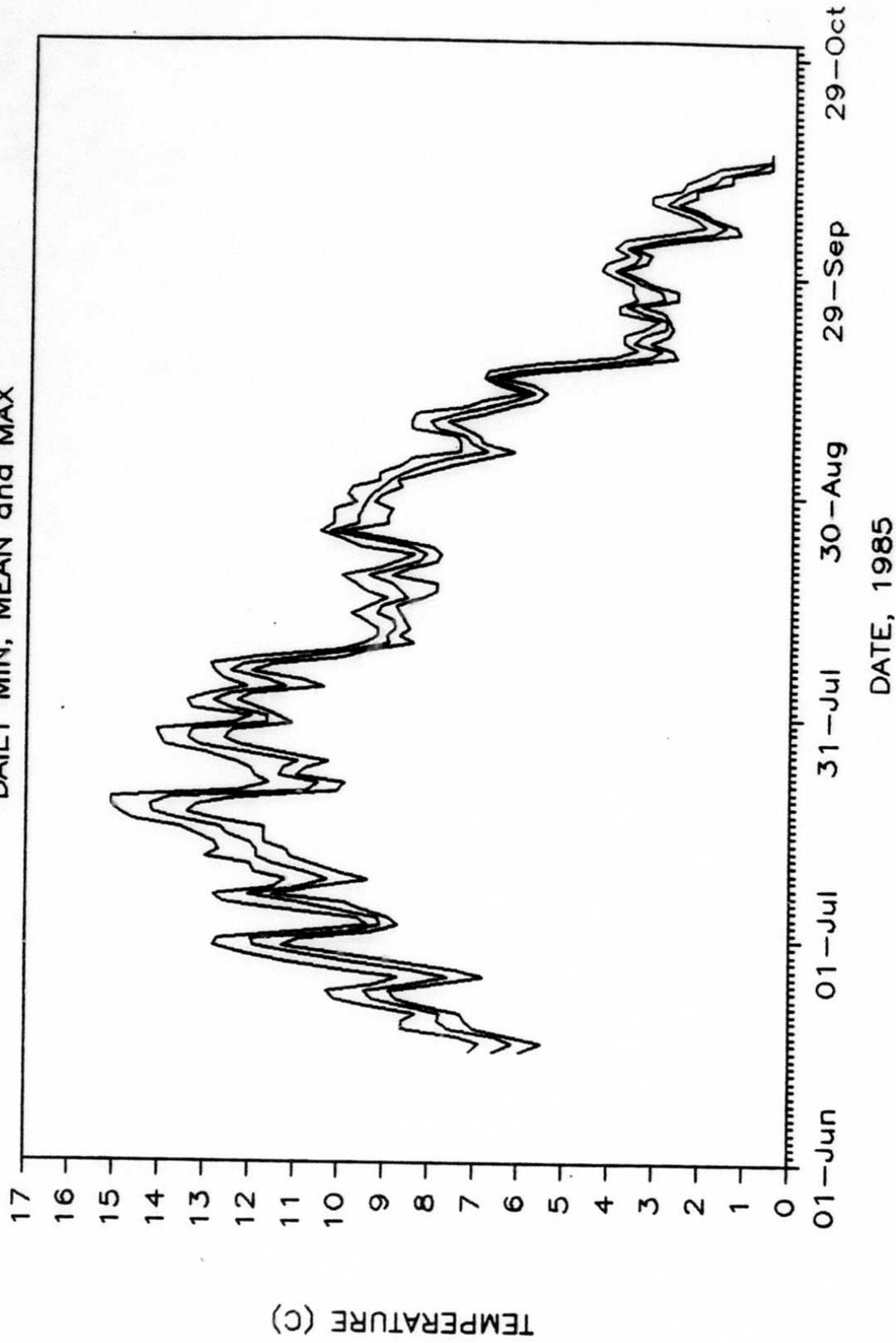
Appendix Figure 14. Daily minimum, mean, and maximum water temperatures monitored at the Devil Canyon Station (RM 150.0).
