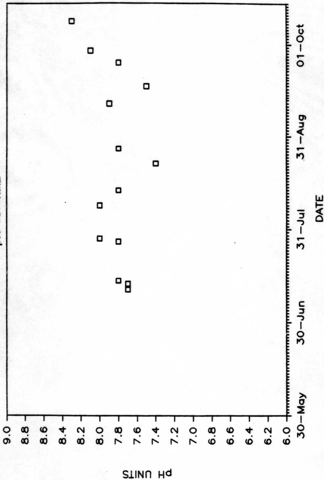
Appendix Figure 42. Weekly measurements of pH from the Talkeetna Station (RM 103.0).
