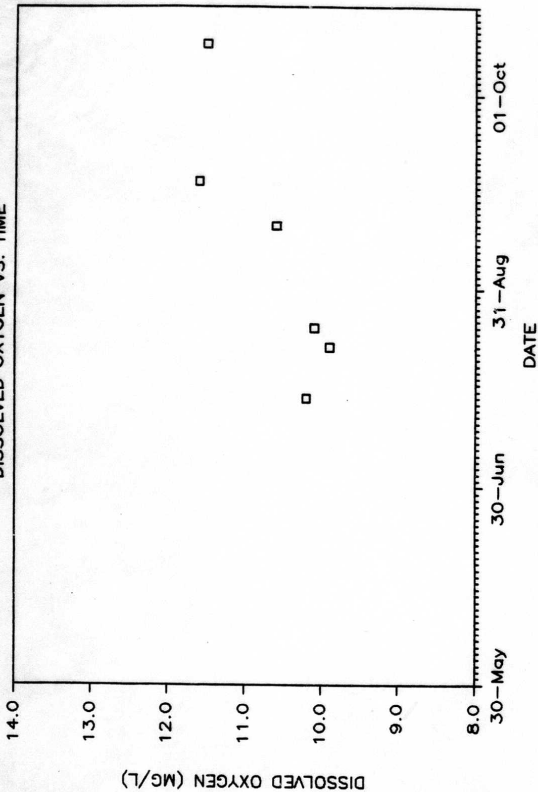
Appendix Figure 34. Weekly dissolved oxygen measurements from the proposed Watana Dam Site (RM 89.2).
