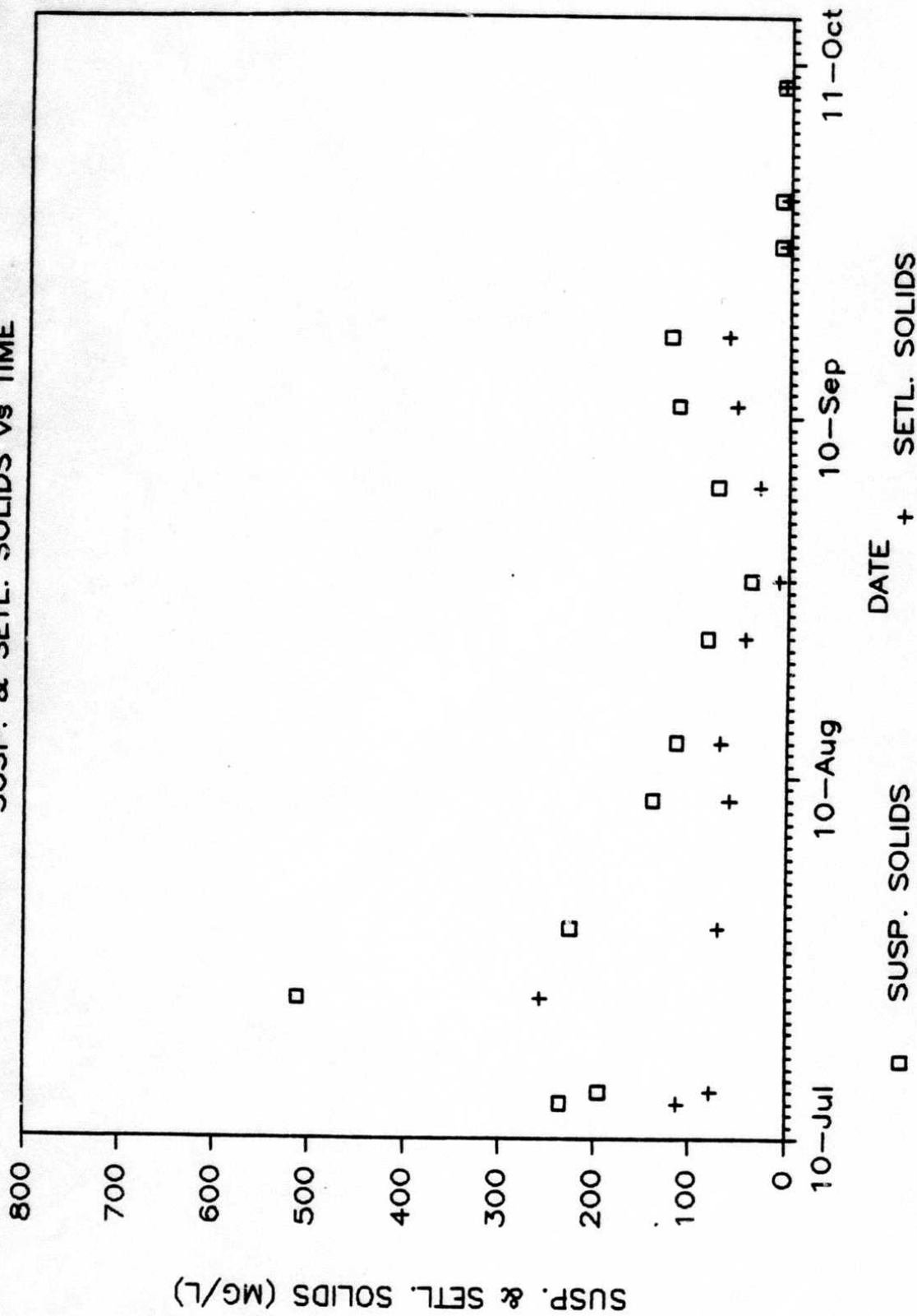
Appendix Figure 23. Weekly suspended and settleable solids measurements from upstream of Curry (RM 120.7).
