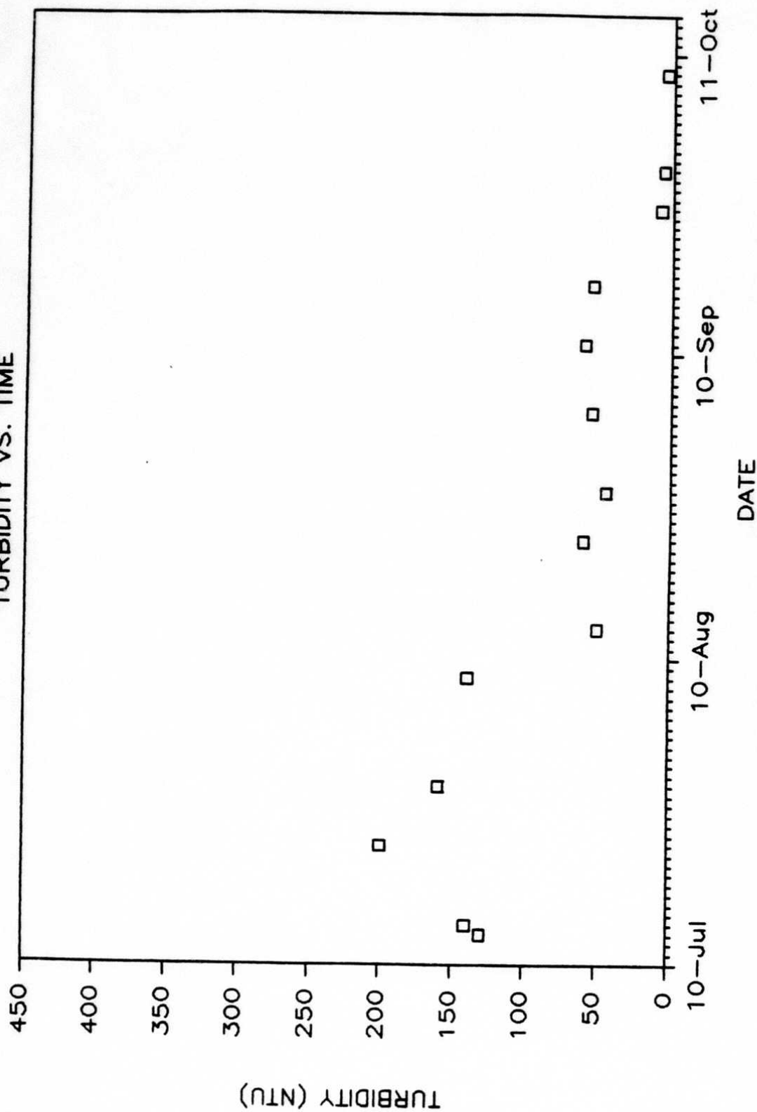
Appendix Figure 19. Weekly measurements of turbidity from downstream of the Gold Creek Bridge (RM 135.8).
