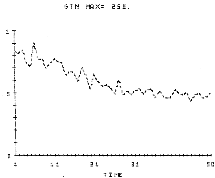
Figure 3.61: Brown bear populations. The maximum on the y-axis is 250 animals.
