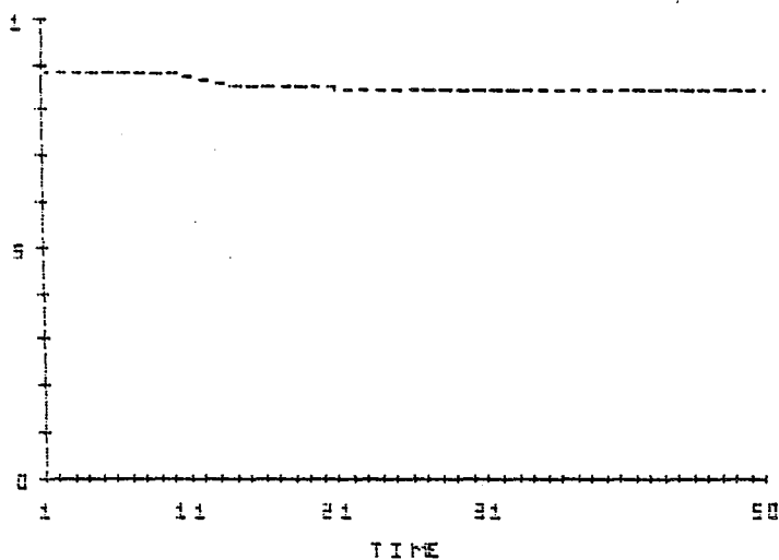
Figure 3.53: The number of bird territories associated with northern water thrush in the total modelled area. The maximum on the y-axis is 50,000.
