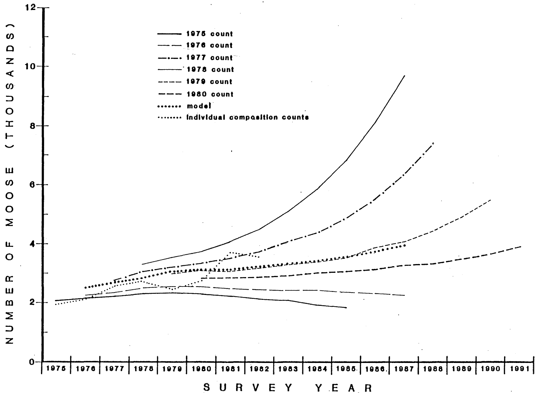
Figure 8. Fall moose population trends derived from modeling using annual composition count data for initial population size for the Sualtna River Study Area, 1975-1991.
