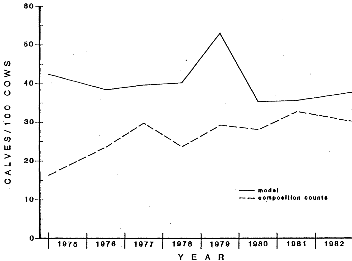
Figure 9. Estimated moose calf:cow ratios derived from modeling versus calf:cow ratios obtained from annual composition counts in the Susitna River Study Area, 1975-1982.
