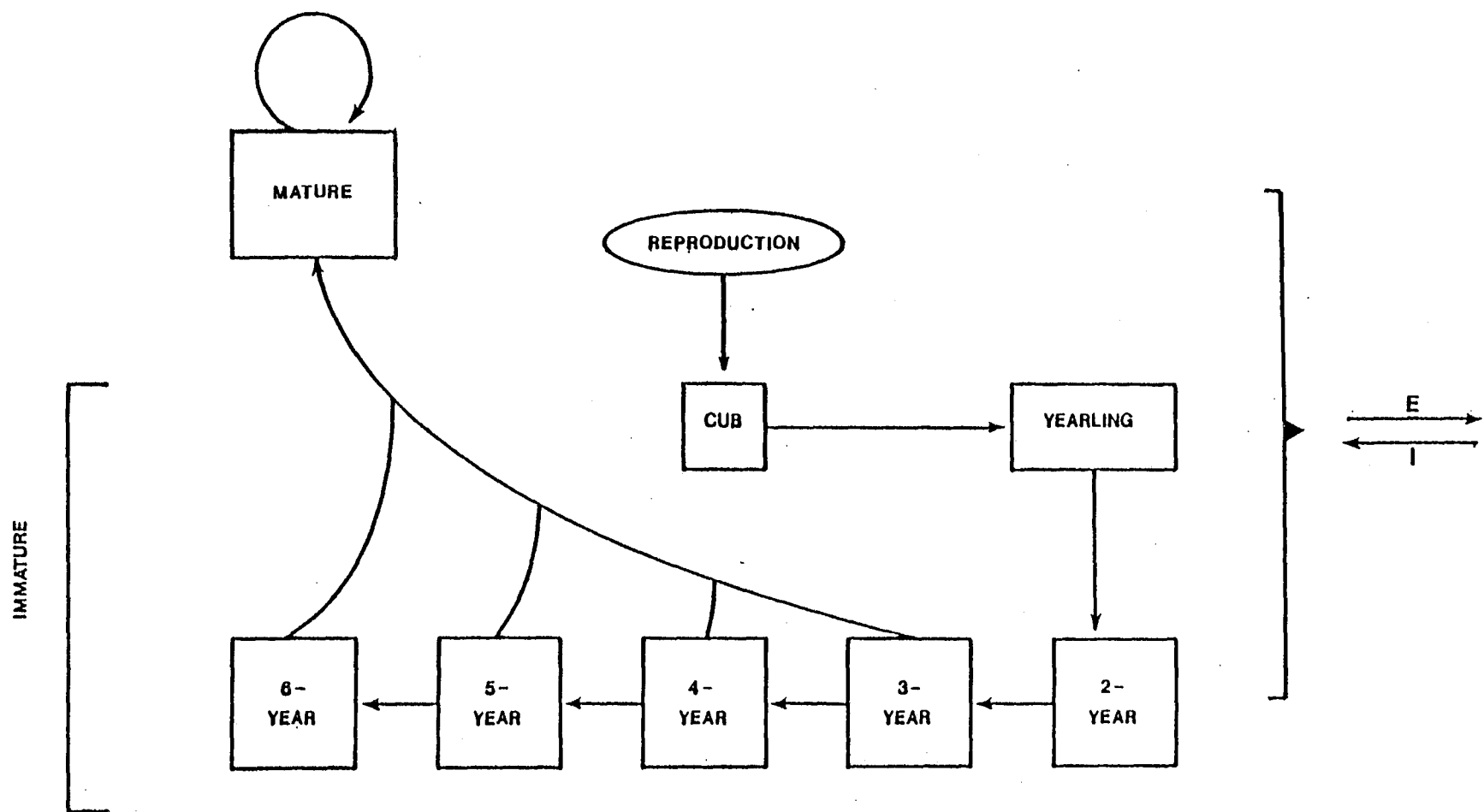
Figure 3.28: Life structure of male brown bear. Each arrow represents a time step of one year.
