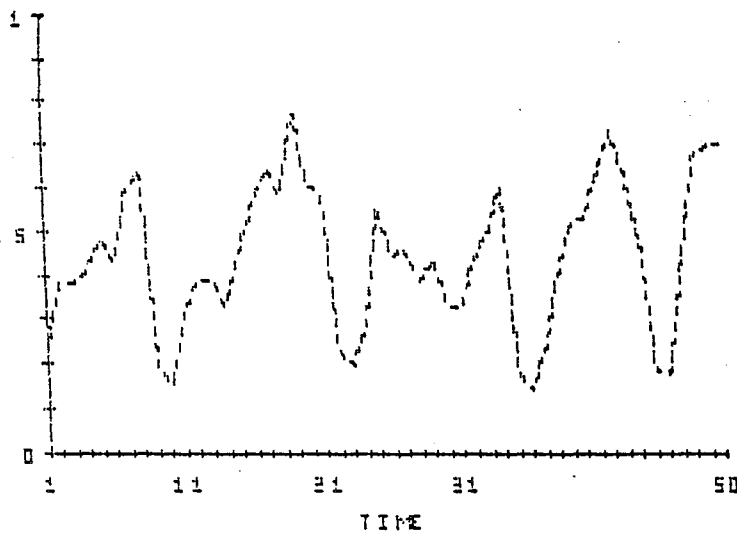
Figure 3.59: Moose harvest. The maximum on the y-axis is 250 animals.
