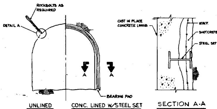
TYPICAL TUNNEL SECTIONS (NOT TO SCALE)
