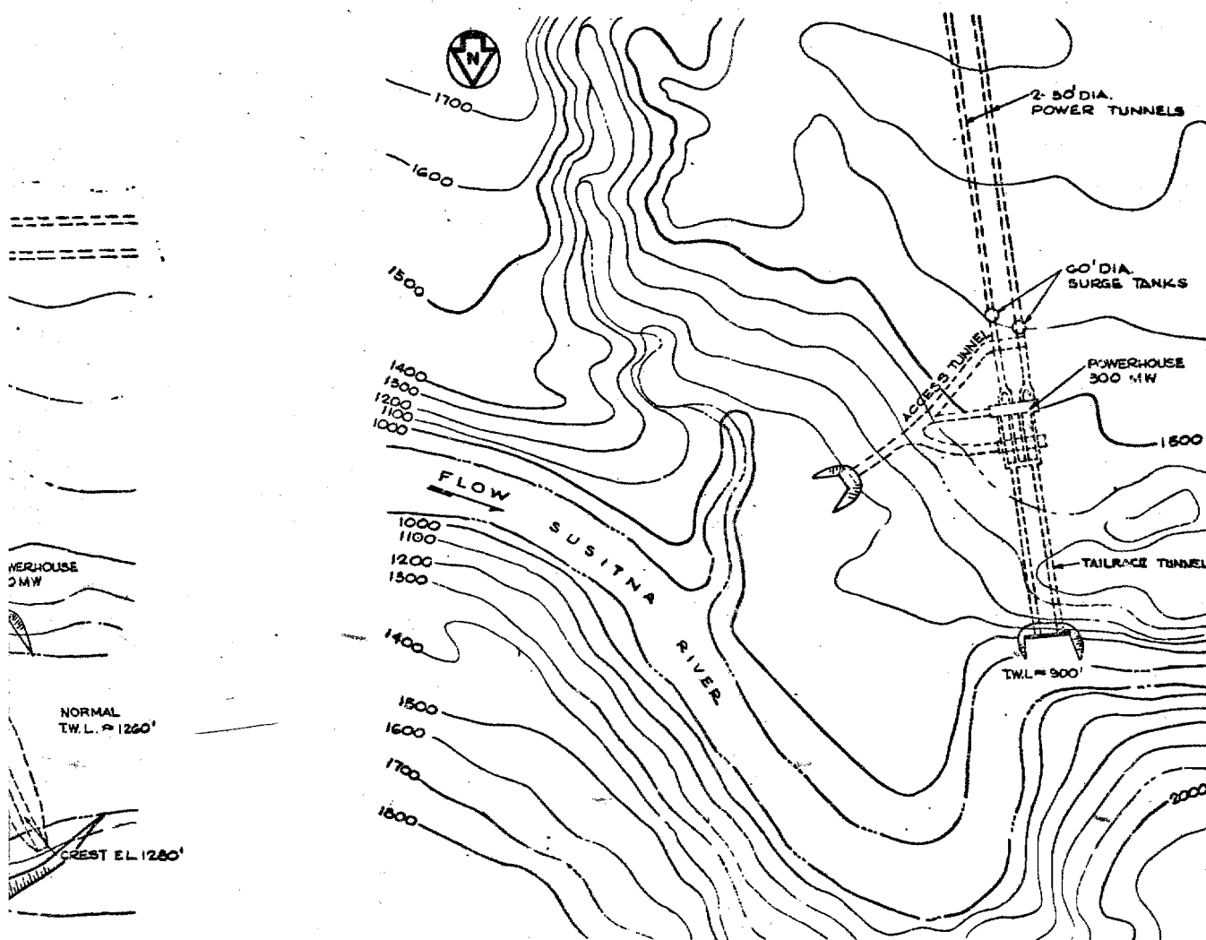
GENERAL ARRANGEMENT DEVIL CANYON POWERHOUSE
