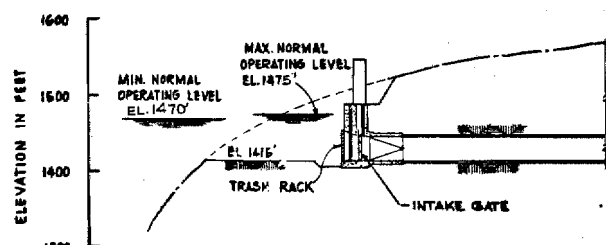
POWER TUNNEL INTAKE SECTION
