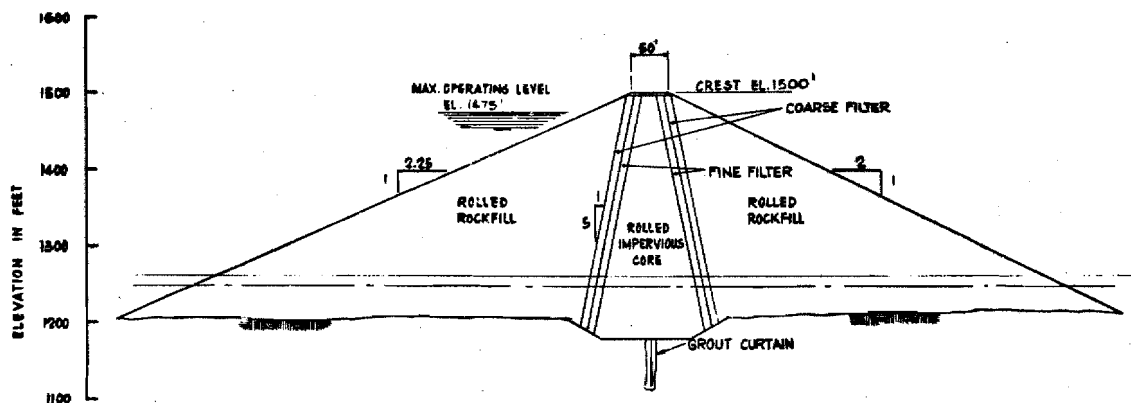
RE-REGULATION DAM TYPICAL SECTION
