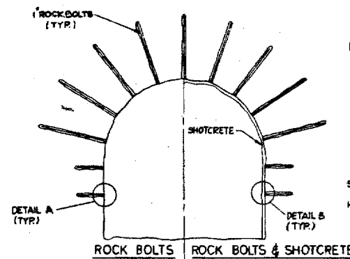
TYPICAL TUNNEL SECTIONS (NOT TO SCALE)
