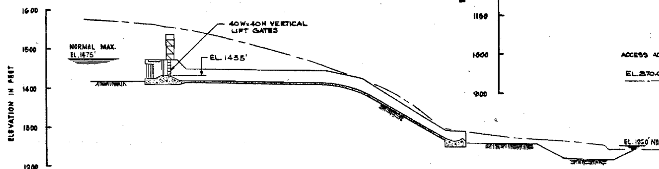
SPILLWAY PROFILE
