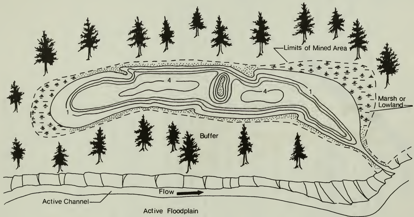
Figure D-1. Desired general configuration of a gravel pit connected to the active channel.
