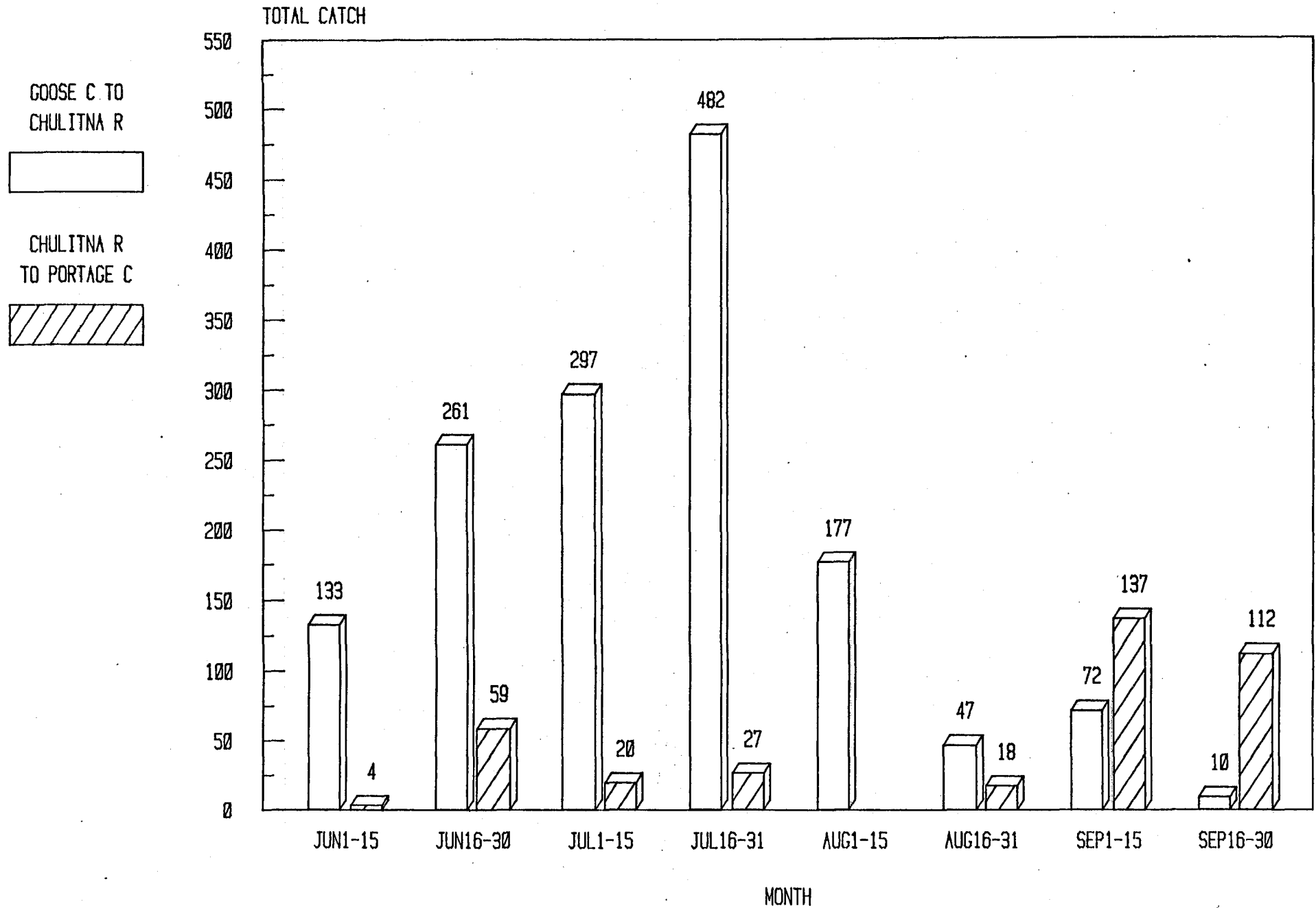
Figure 18. Relative utilization by two week period of Lower and Upper Susitna DFH sites by coho salmon. (ADF&C 1983c)
