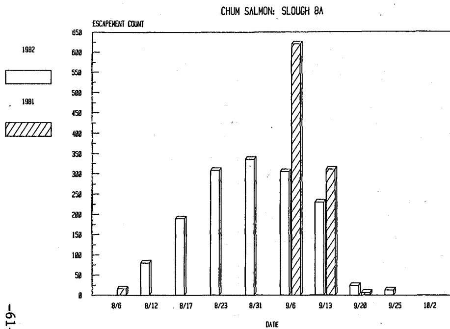
Figure 16. Weekly chum salmon escapement to four Upper Susitna sloughs. (From ADF&G 1983b)
