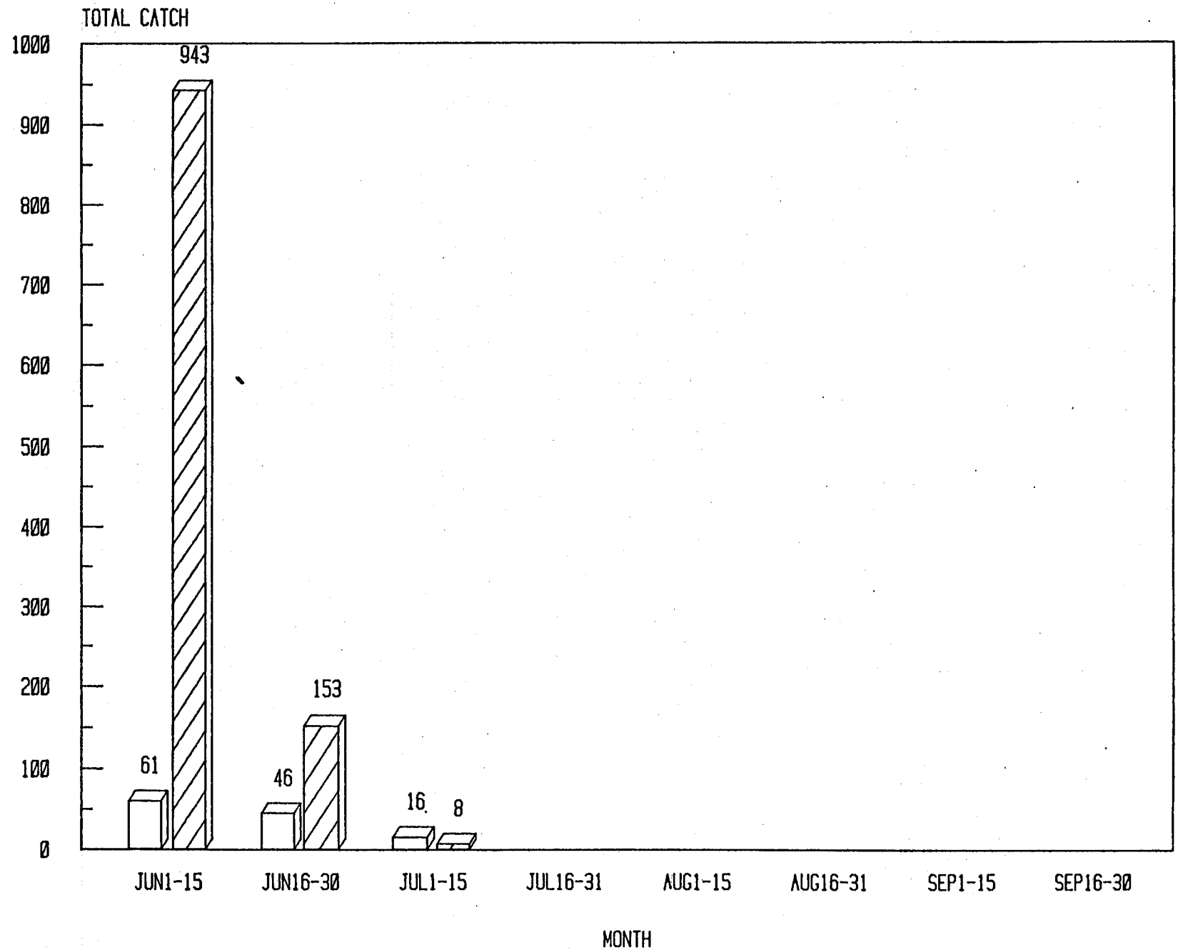
Figure 20. Relative utilization by two week period of Lower and Upper Susitna DFH sites by chum salmon (ADF&G 1983c)
