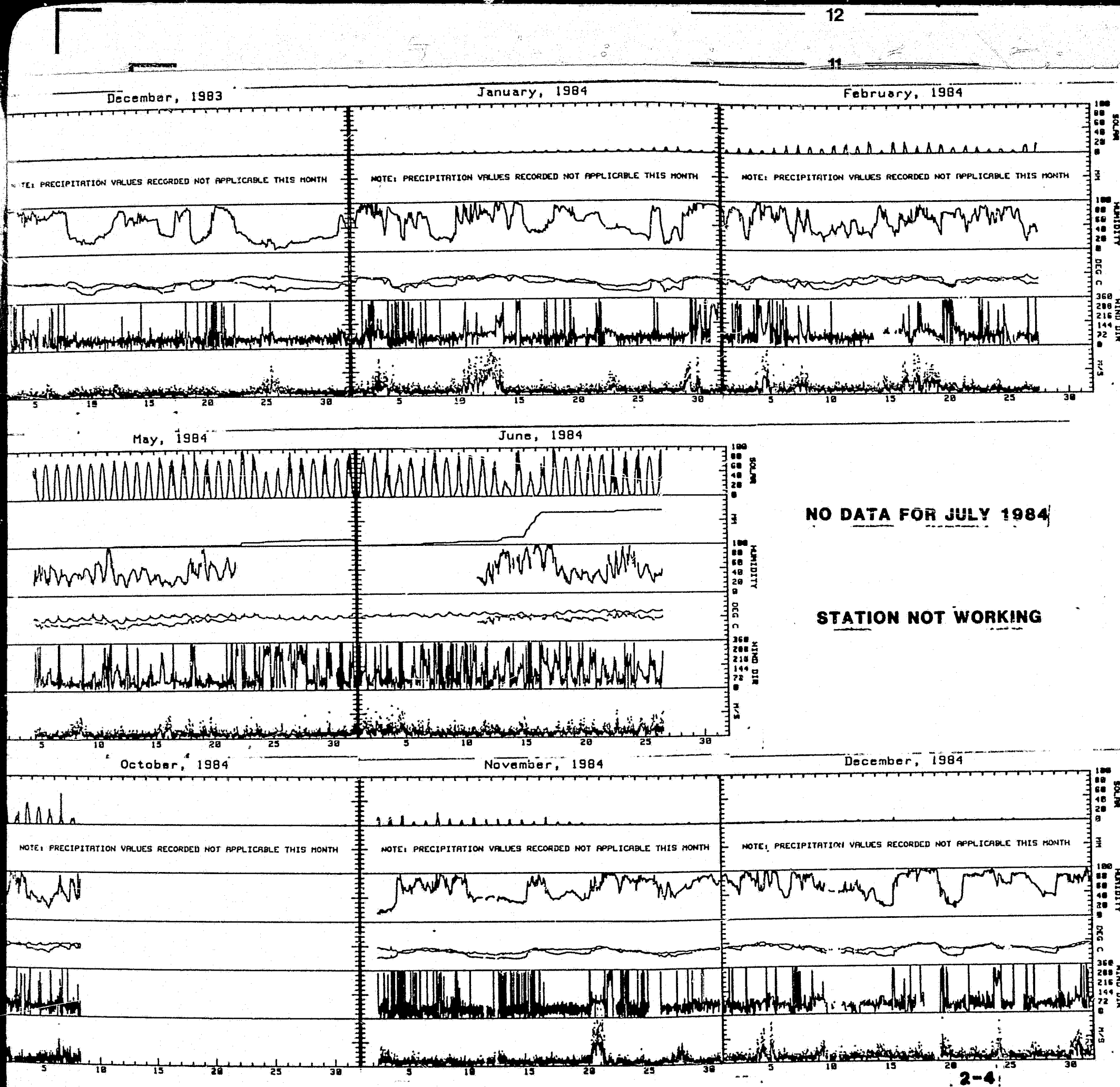
FIGURE 2.1: SEQUENTIAL PLOT OF CLIMATIC DATA, SUSITNA GLACIER STATION, OCTOBER 1983- DECEMBER 1984
