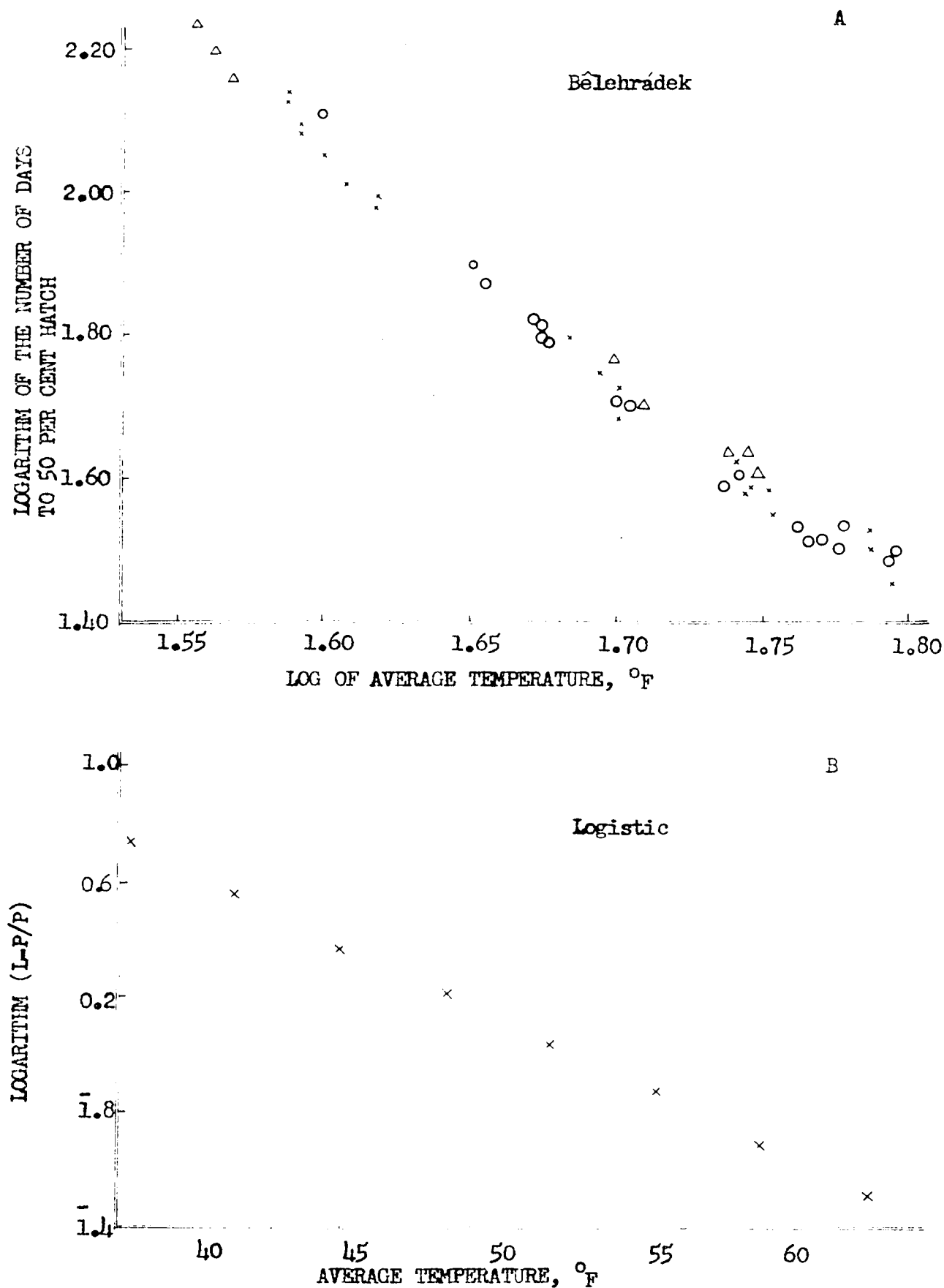
Figure 16. Relationship of the Bělehrádek Equation and the Logistic Equation to the Rate of Development Data from all Lots. A, Relationship of the Logarithm of Temperature to the Logarithm of the Number of Days to Hatching. B, Relationship of Temperature to the Logarithm of L-P/P.
