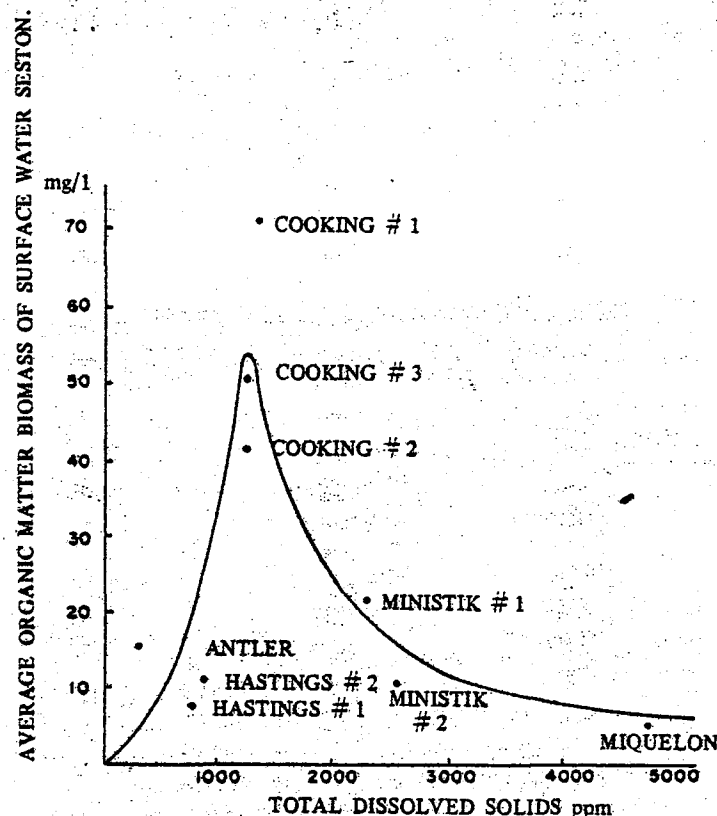
Figure 1. Relationship of organic matter biomass of surface water seston (productivity) to the total dissolved solids in nine bodies of water in central Alberta. (Kerekes and Nurshall (1966), reprinted by permission of the International Association of Theoretical and Applied Limnology.)
