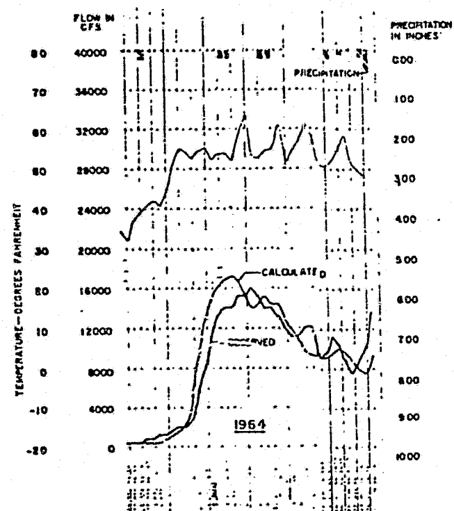
HYDROGRAPH SUSITNA RIVER NEAR DENALI, 1964, 1971
