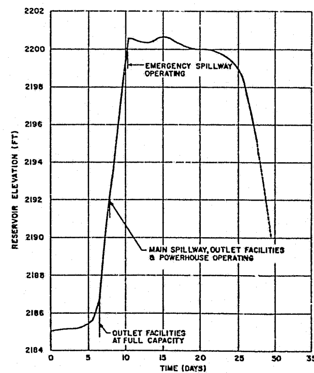
PROBABLE MAXIMUM FLOOD
