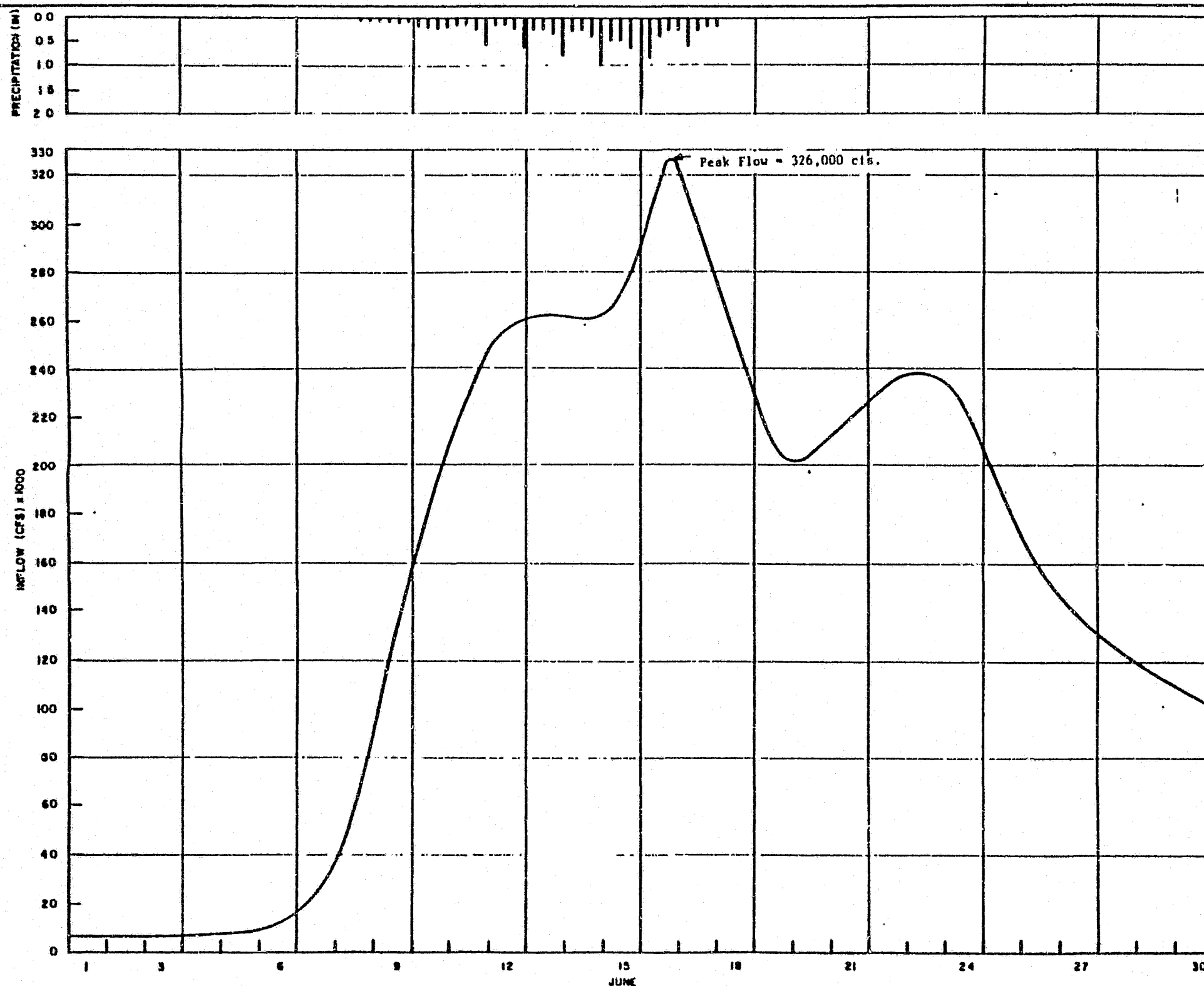
WATANA PMF INFLOW HYDROGRAPH
