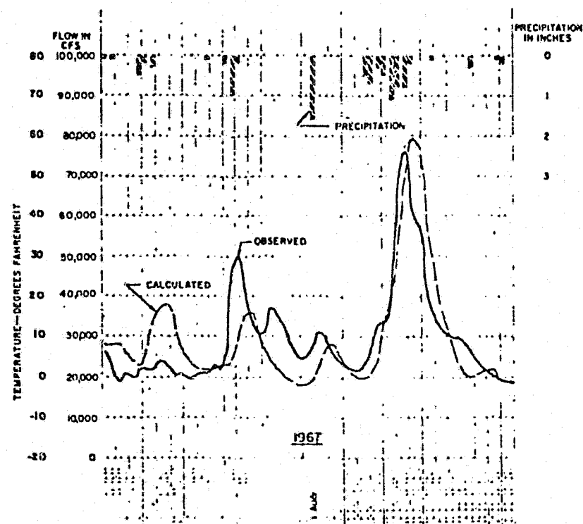
HYDROGRAPH: SUSITNA RIVER AT GOLD CREEK, 1967, 1972
