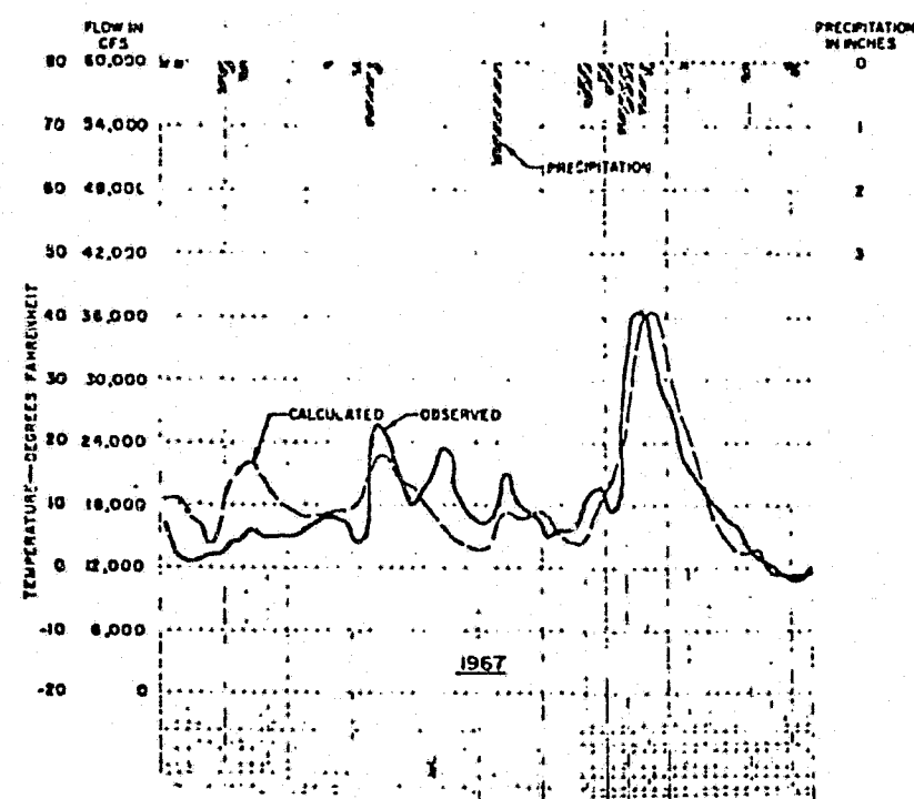
HYDROGRAPH : SUSITNA RIVER NEAR CANTWELL, 1967, 1972
