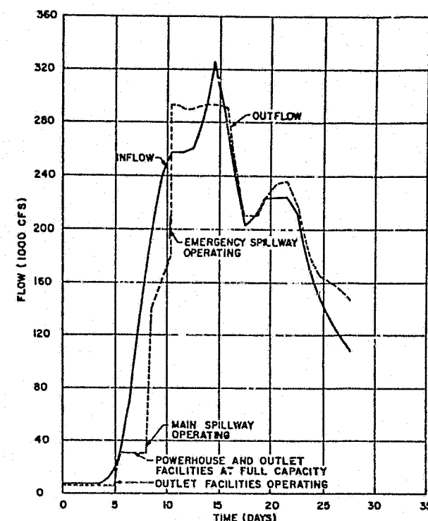
PROBABLE MAXIMUM FLOOD
