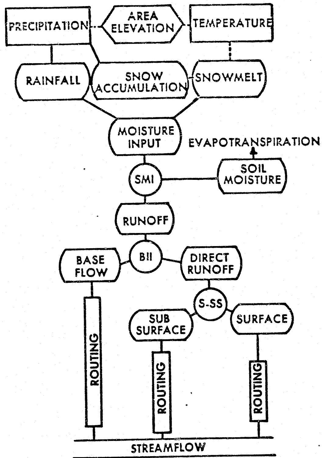
SSARR WATERSHED MODEL
