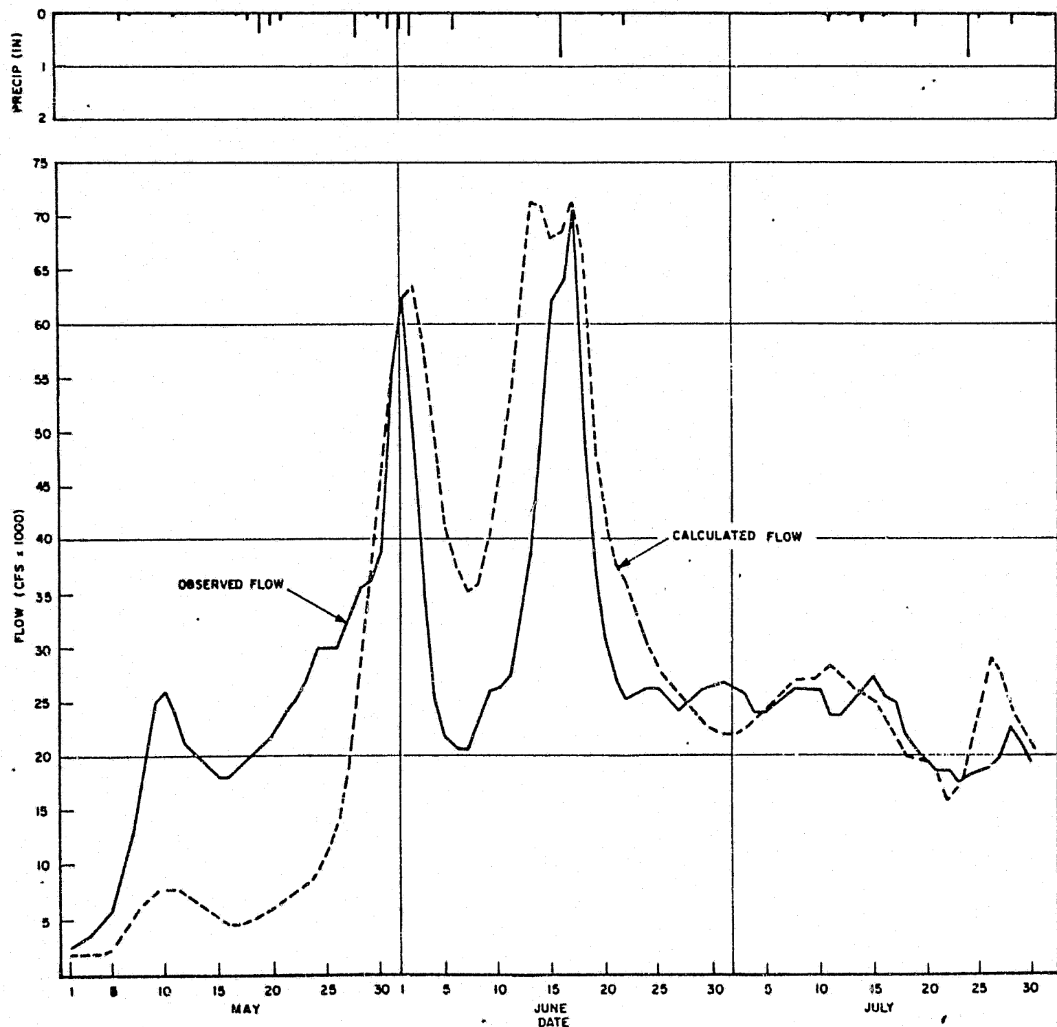
SSARR MODEL CALIBRATION SUSITNA RIVER AT GOLD CREEK 1972 FLOOD
