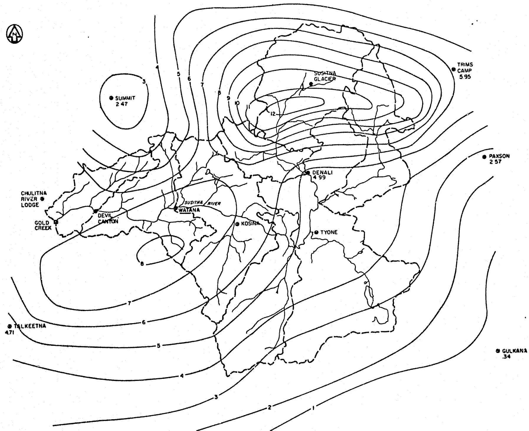
ISOHYETAL MAP STORM OF AUGUST 9-17, 1967
