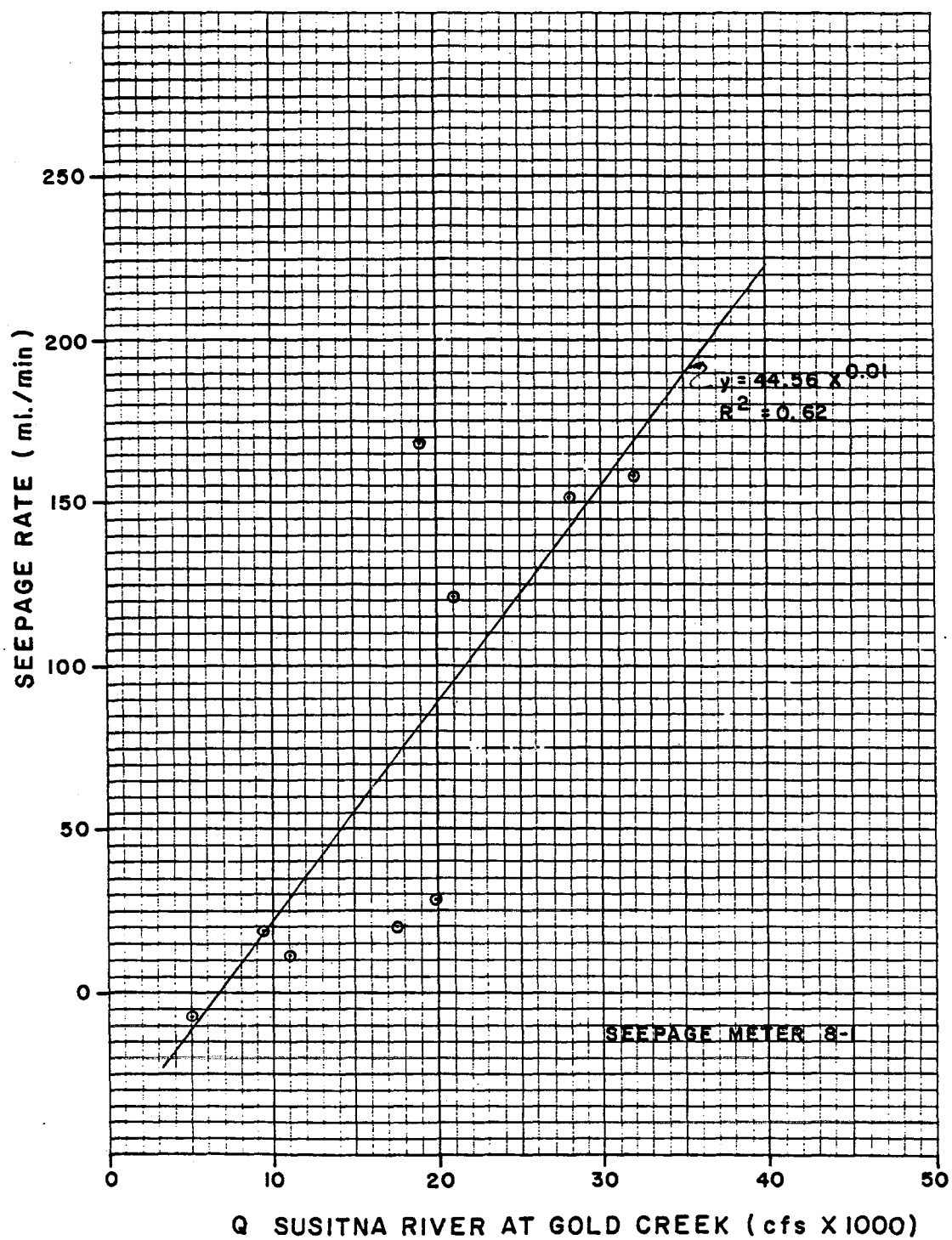
EXHIBIT 21. SEEPAGE RATE VS. MAINSTEM DISCHARGE, SEEPAGE METER 8-1.
