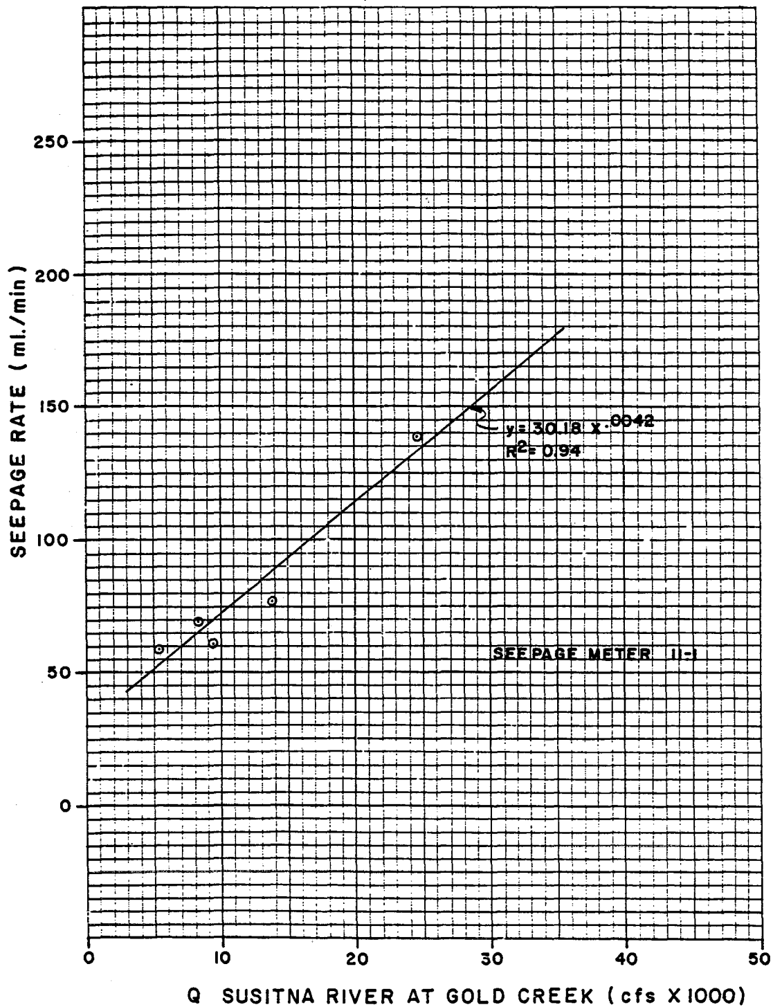
EXHIBIT 26. SEEPAGE RATE VS. MAINSTEM DISCHARGE, SEEPAGE METER 11-1.
