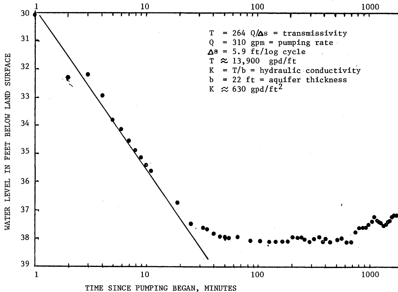
EXHIBIT 13. ANALYSIS OF TALKEETNA FIRE HALL WELL PUMPING TEST.
