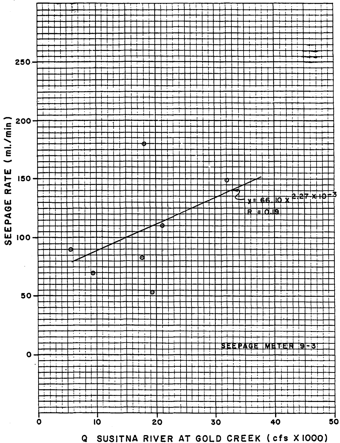
EXHIBIT 25. SEEPAGE RATE VS. MAINSTEM DISCHARGE, SEEPAGE METER 9-3.
