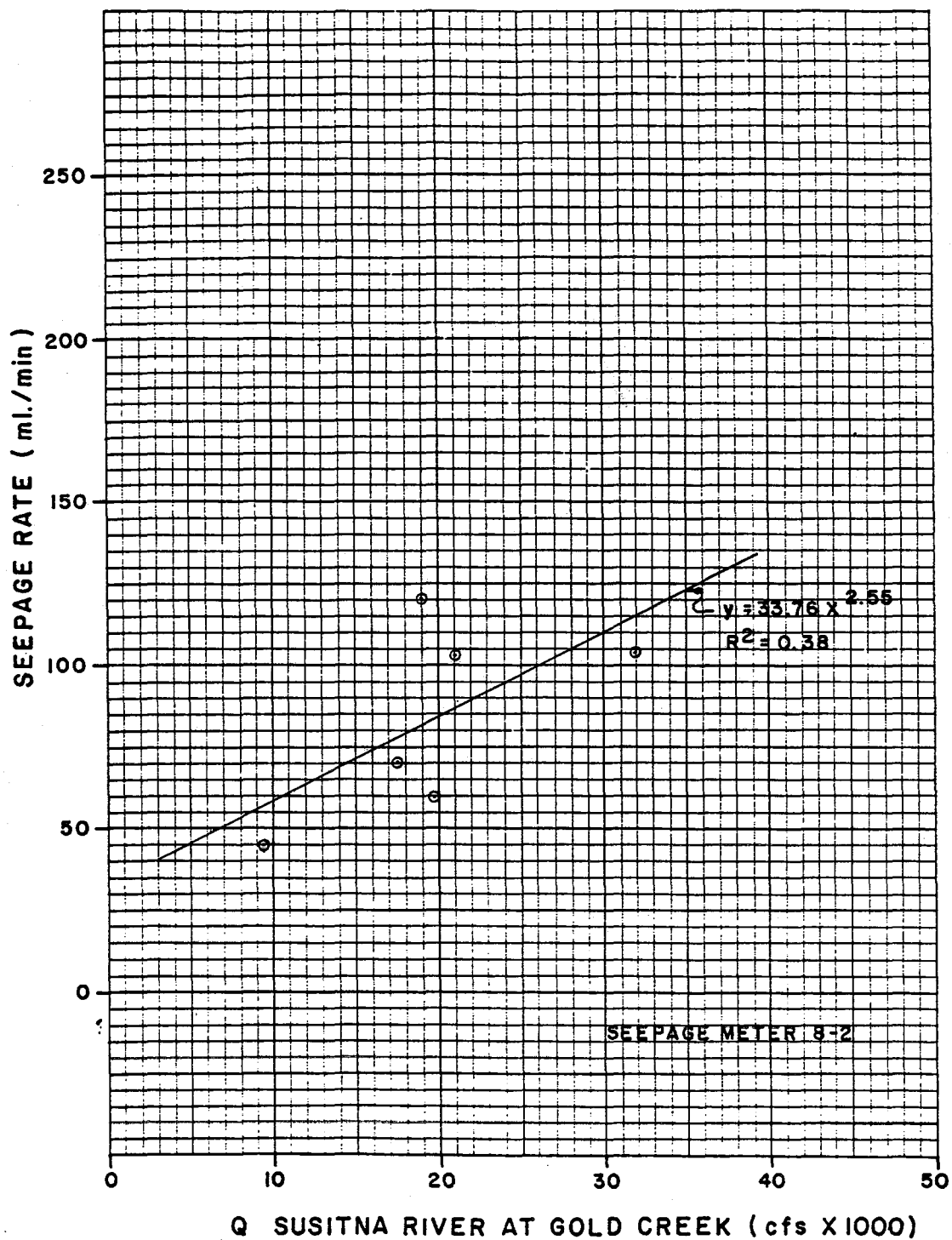
EXHIBIT 22. SEEPAGE RATE VS. MAINSTEM DISCHARGE, SEEPAGE METER 8-2.
