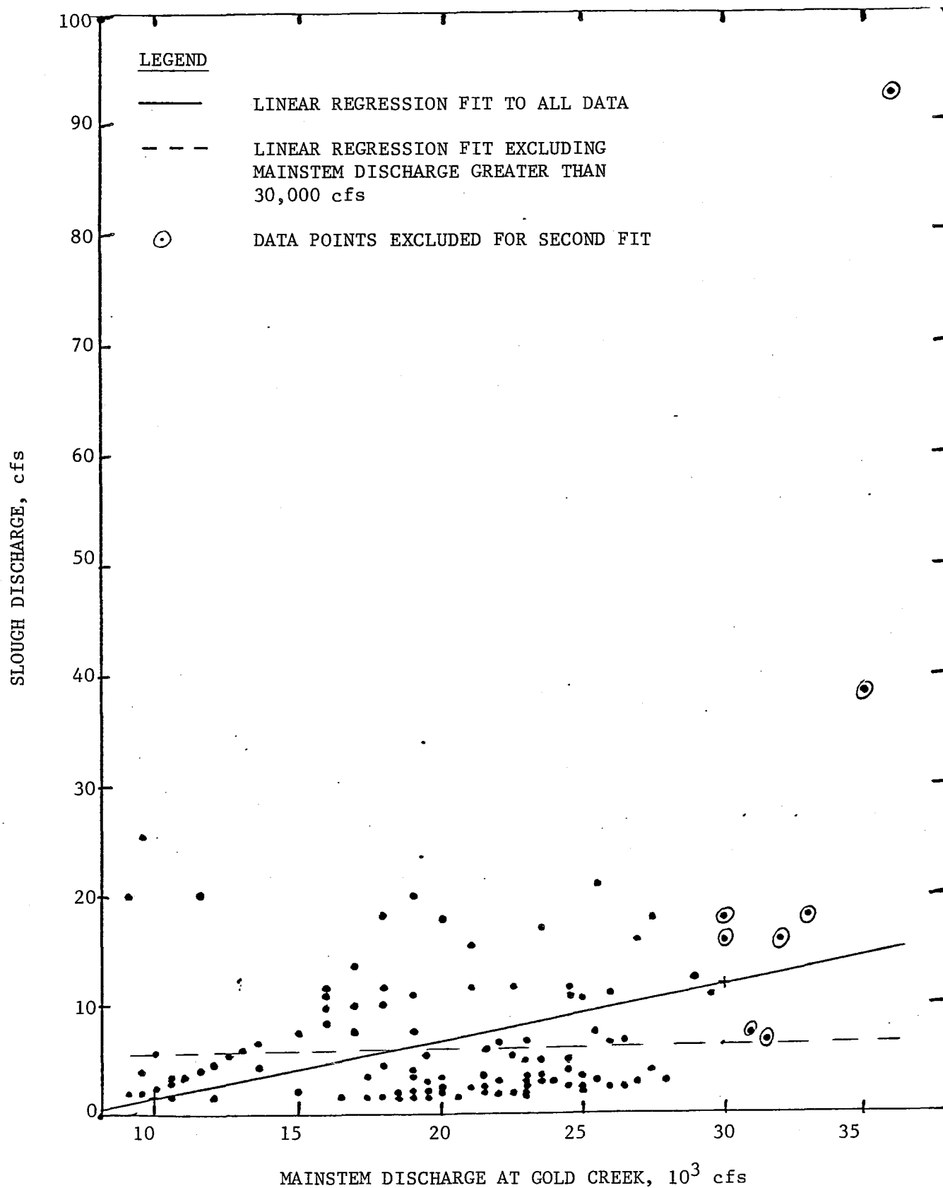
EXHIBIT 18a. SLOUGH 8A DISCHARGE VS. MAINSTEM DISCHARGE AT GOLD CREEK, SUMMER 1983
