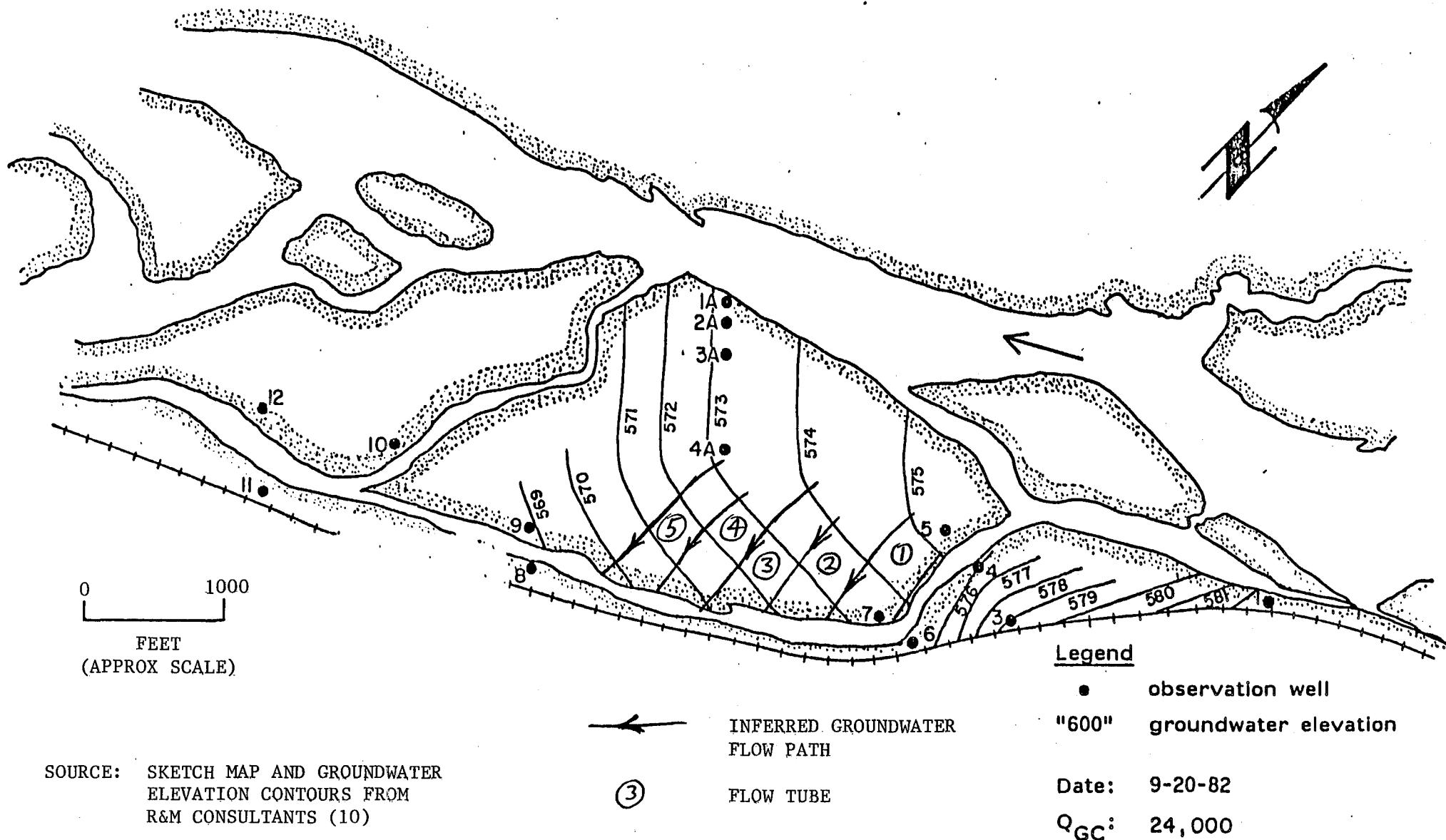
EXHIBIT 10. GROUNDWATER CONTOURS AND FLOW PATHS, SUSITNA RIVER AT SLOUGH 8A.
