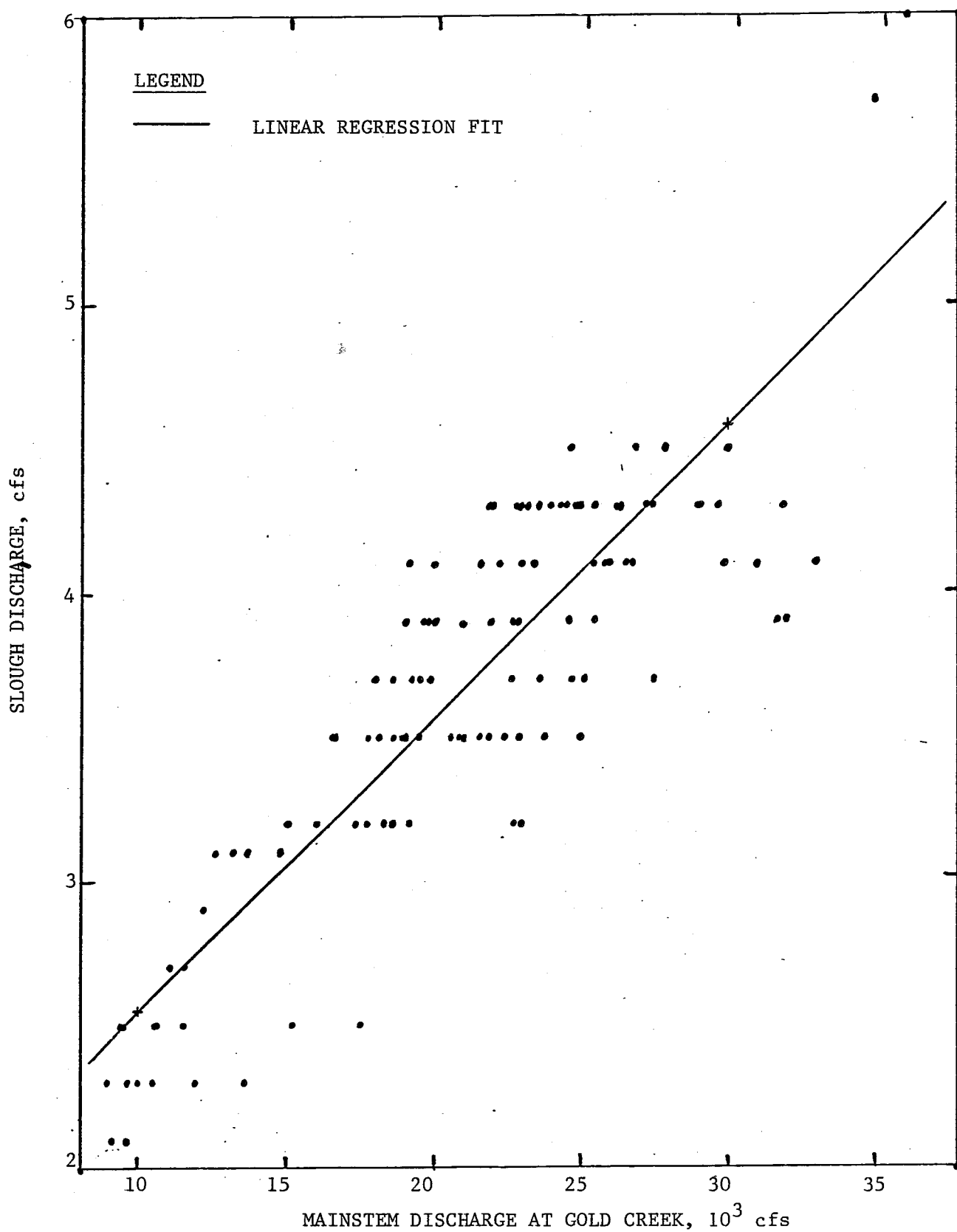
EXHIBIT 20. SLOUGH 11 DISCHARGE VS. MAINSTEM DISCHARGE AT GOLD CREEK, SUMMER 1983
