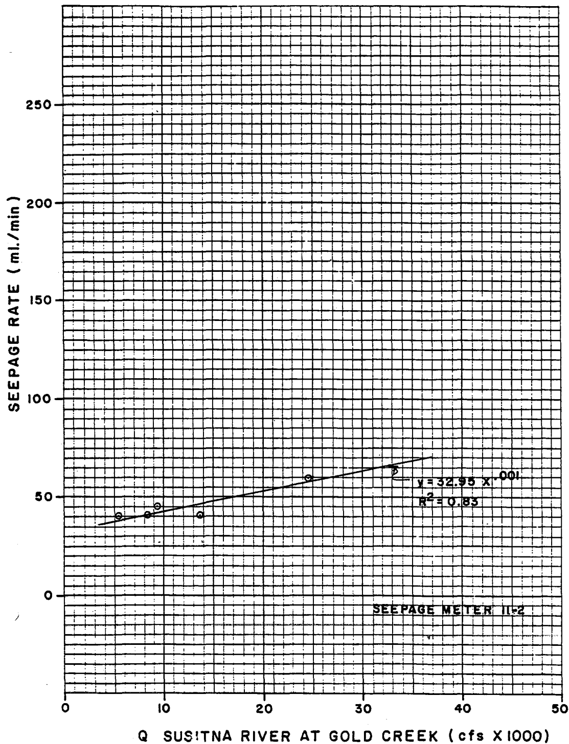
EXHIBIT 27. SEEPAGE RATE VS. MAINSTEM DISCHARGE, SEEPAGE METER 11-2.
