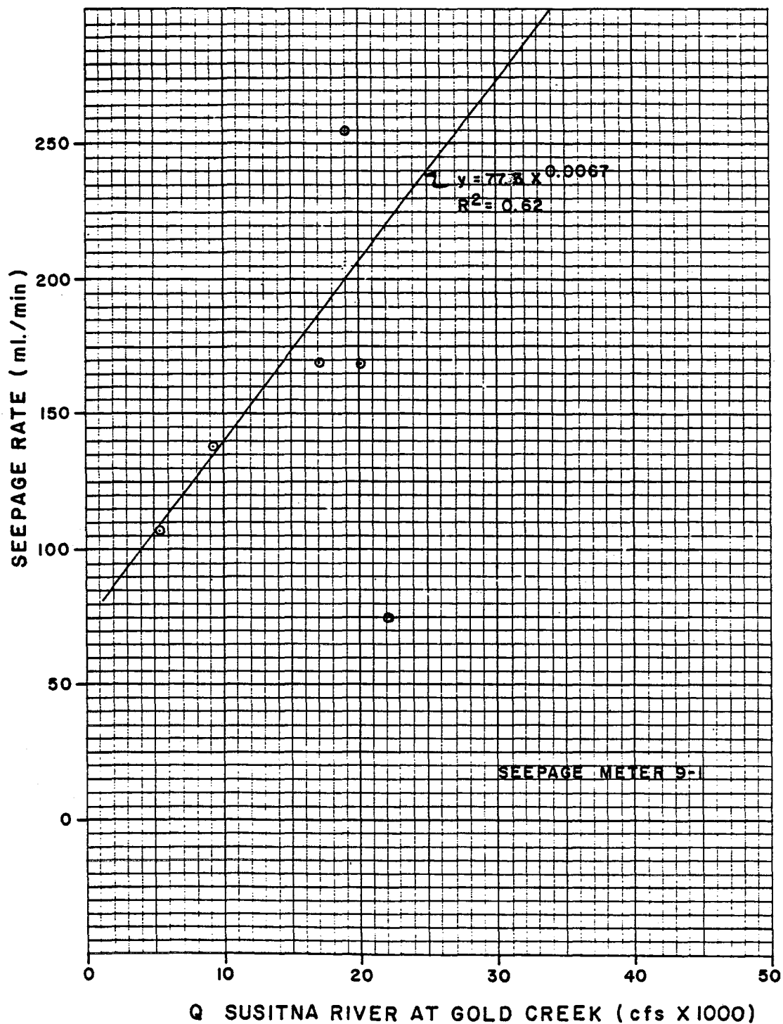
EXHIBIT 23. SEEPAGE RATE VS. MAINSTEM DISCHARGE, SEEPAGE METER 9-1.
