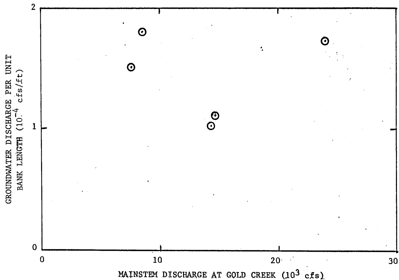
EXHIBIT 11. GROUNDWATER DISCHARGE VS. MAINSTEM DISCHARGE, SLOUGH 8A IN 1982.
