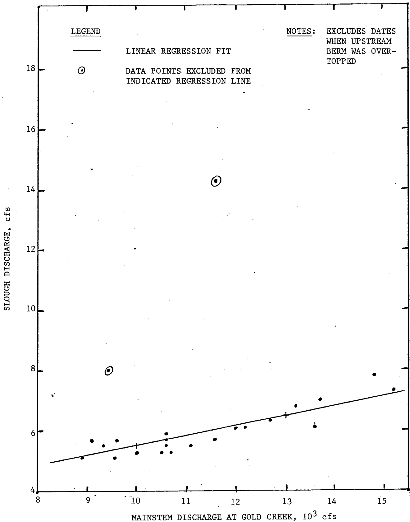
EXHIBIT 19b. SLOUGH 9 DISCHARGE VS. MAINSTEM DISCHARGE AT GOLD CREEK, SUMMER 1983
