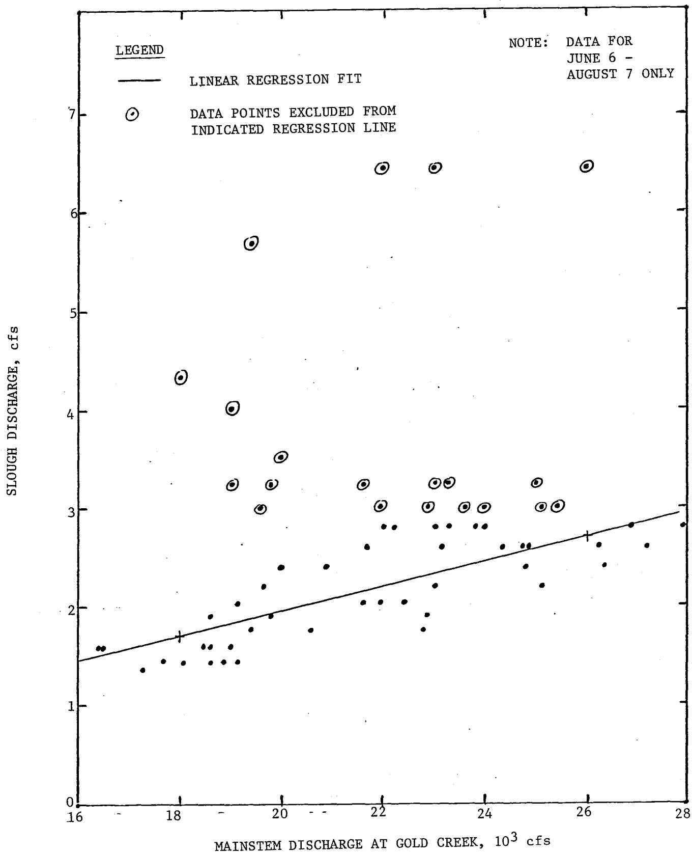
EXHIBIT 18b. SLOUGH 8A DISCHARGE VS. MAINSTEM DISCHARGE AT GOLD CREEK, SUMMER 1983
