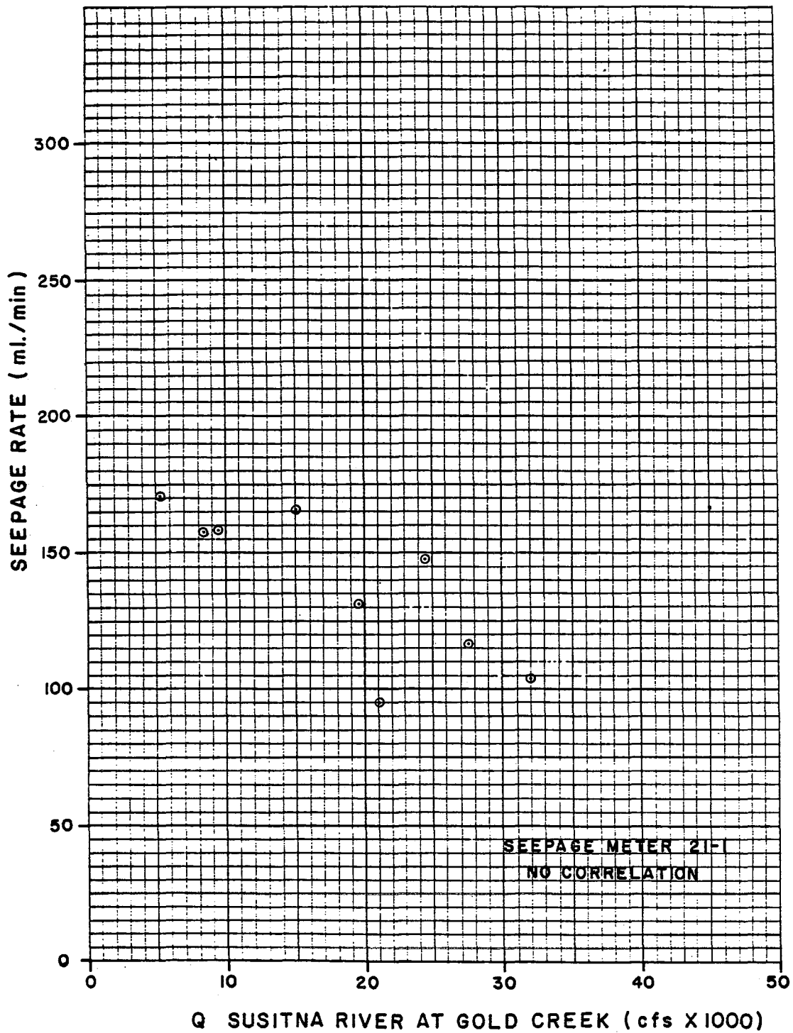
EXHIBIT 28. SEEPAGE RATE VS. MAINSTEM DISCHARGE, SEEPAGE METER 21-1.
