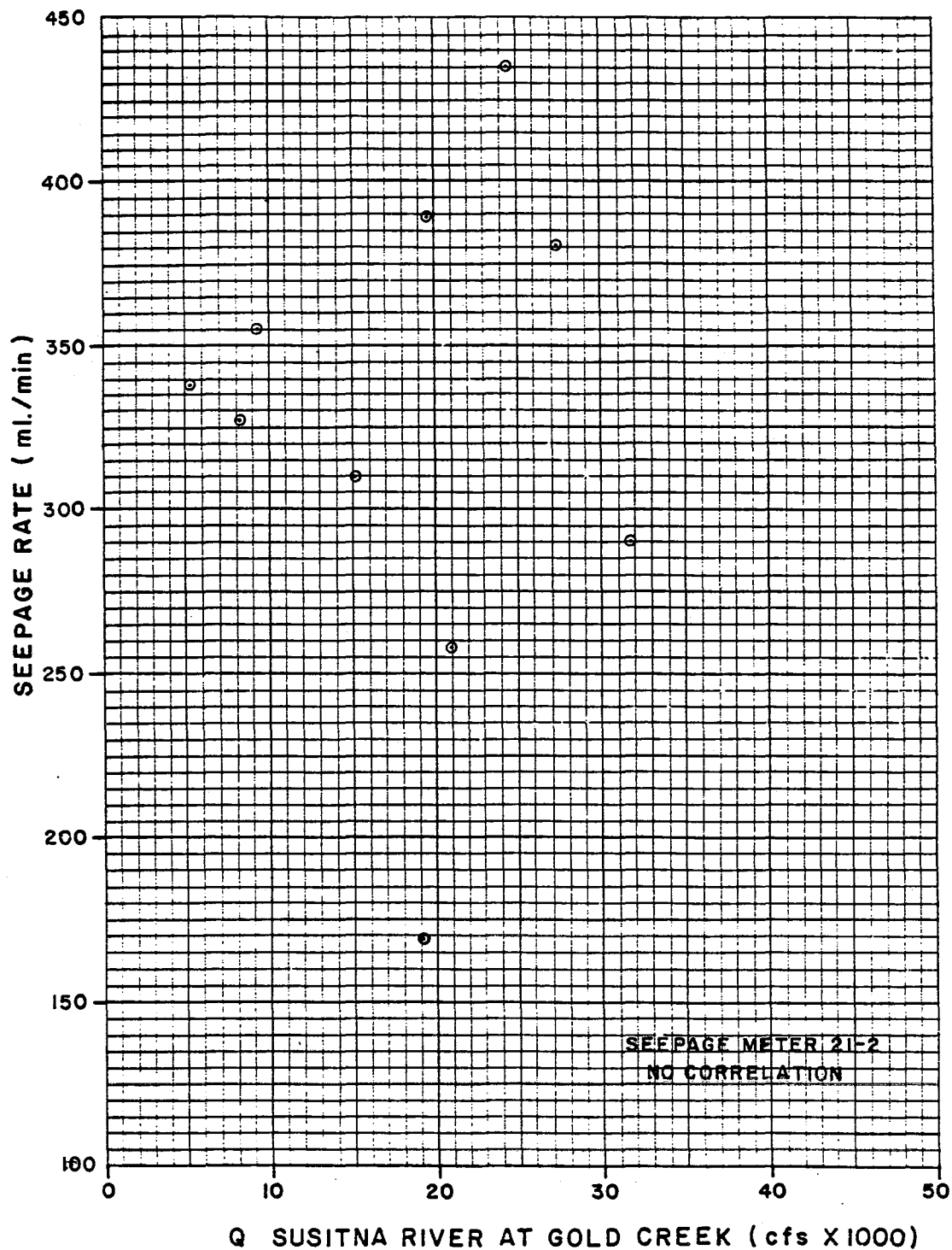
EXHIBIT 29. SEEPAGE RATE VS. MAINSTEM DISCHARGE, SEEPAGE METER 21-2.
