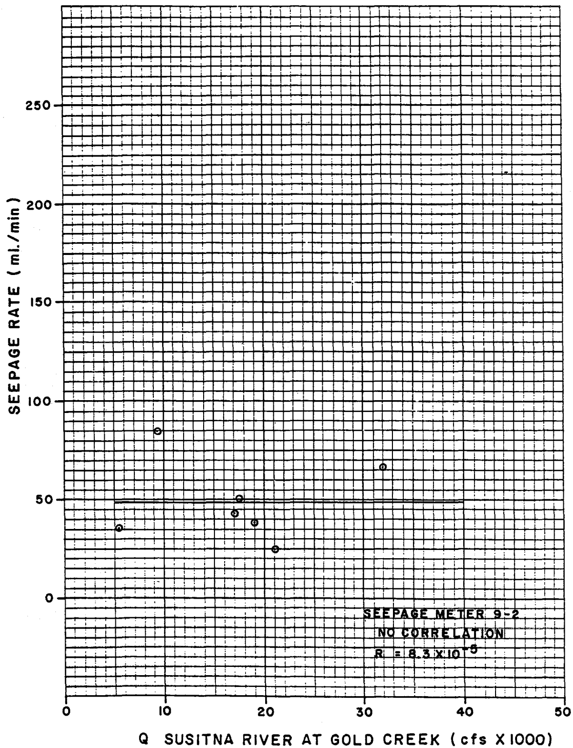
EXHIBIT 24. SEEPAGE RATE VS. MAINSTEM DISCHARGE, SEEPAGE METER 9-2.
