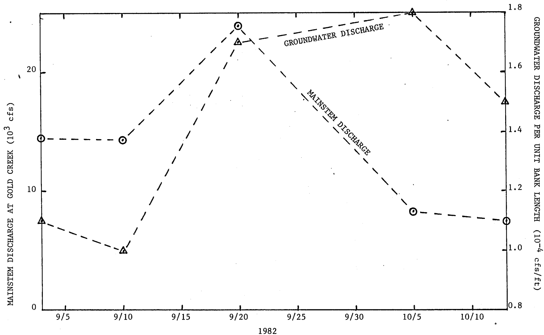
EXHIBIT 12. GROUNDWATER DISCHARGE AND MAINSTEM DISCHARGE VS. TIME, SLOUGH 8A, SEPT-OCT 1982.
