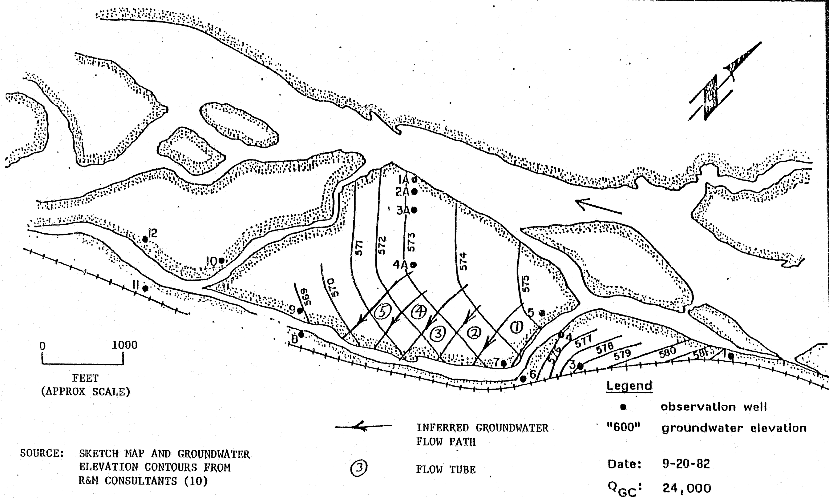
EXHIBIT 10. GROUNDWATER CONTOURS AND FLOW PATHS, SUSITNA RIVER AT SLOUGH 8A.
