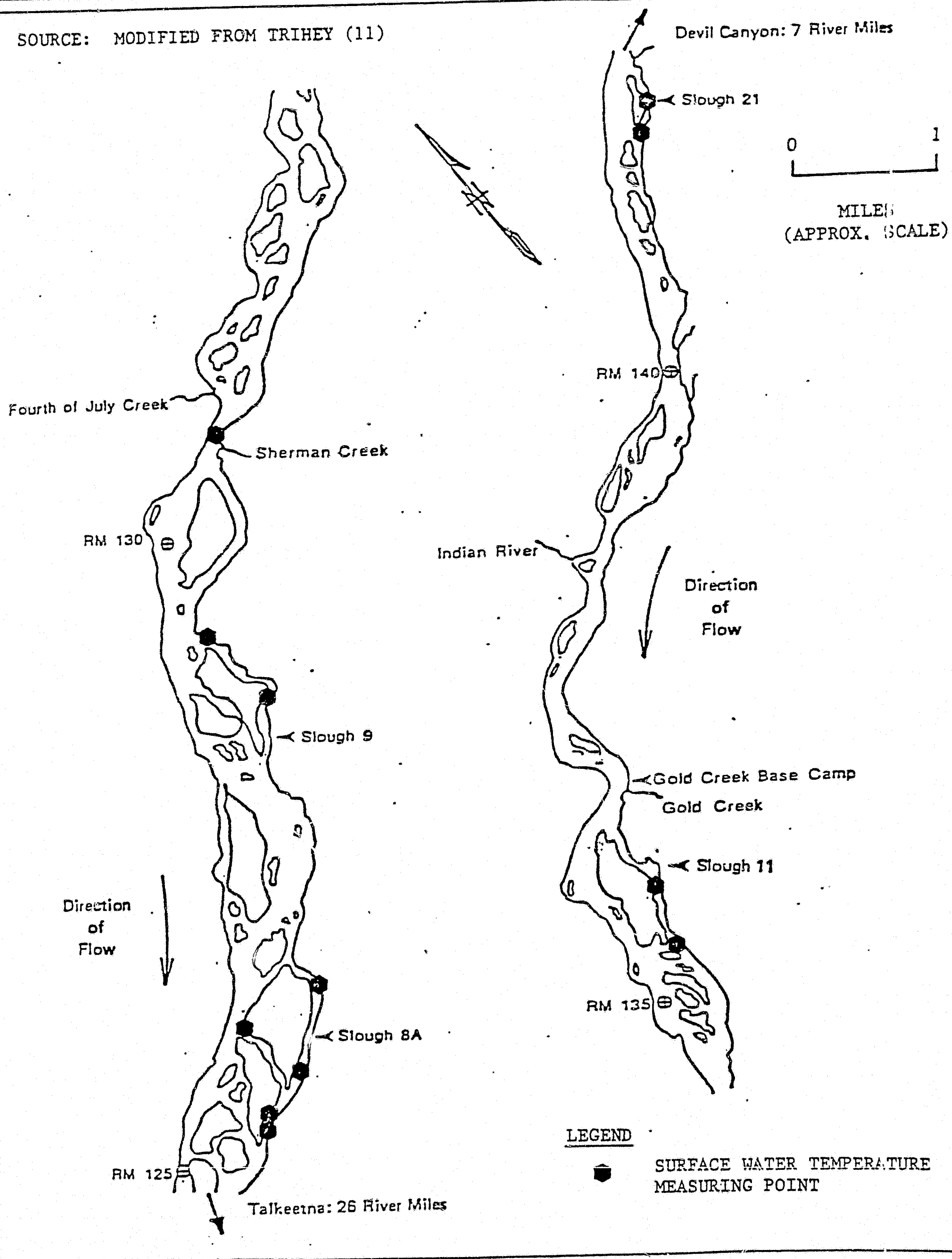
EXHIBIT 4. APPROXIMATE LOCATIONS OF DATA COLLECTION POINTS - SURFACE WATER TEMPERATURE, SUMMER 1982.
