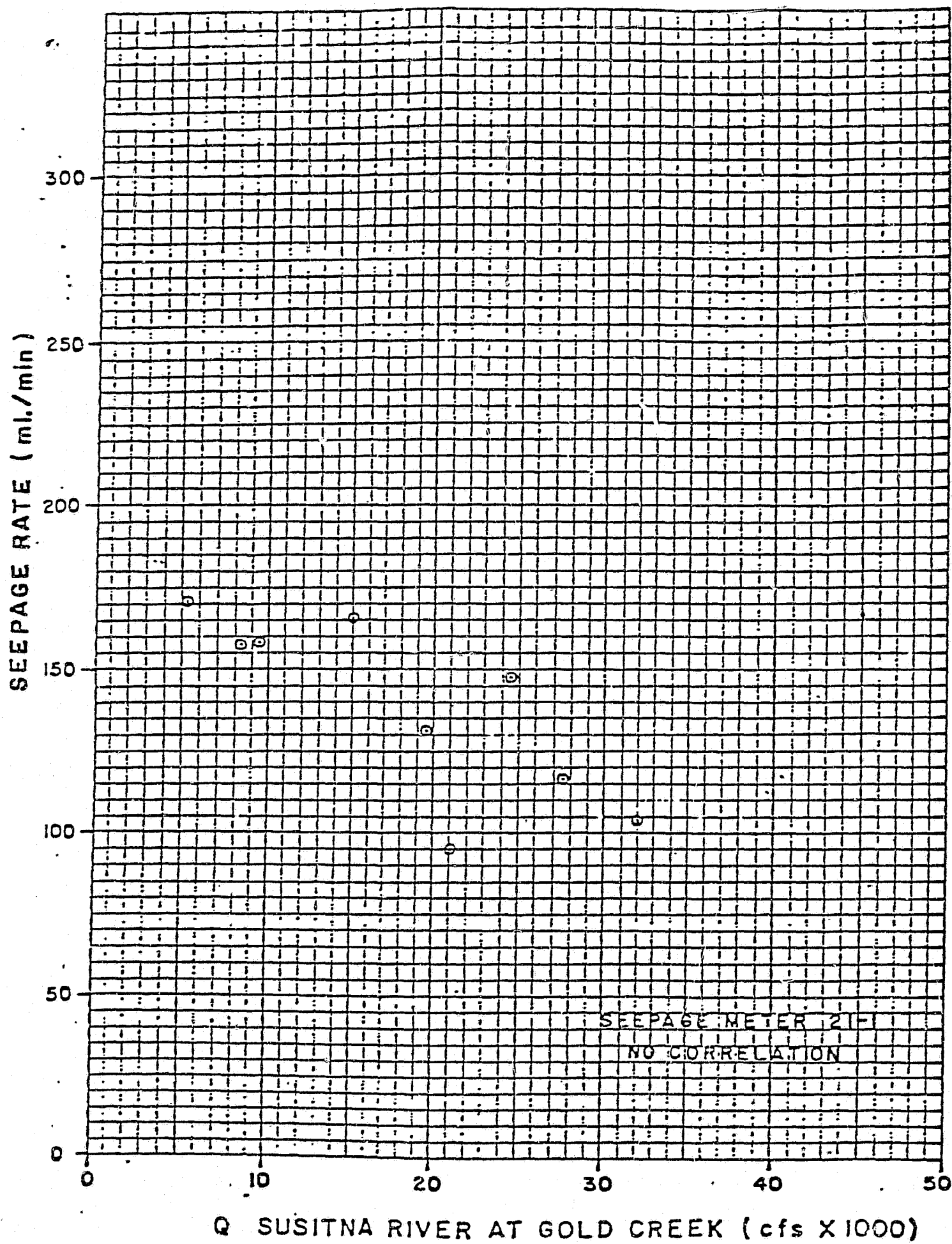
EXHIBIT 28. SEEPAGE RATE VS. MAINSTEM DISCHARGE, SEEPAGE METER 21-1.
