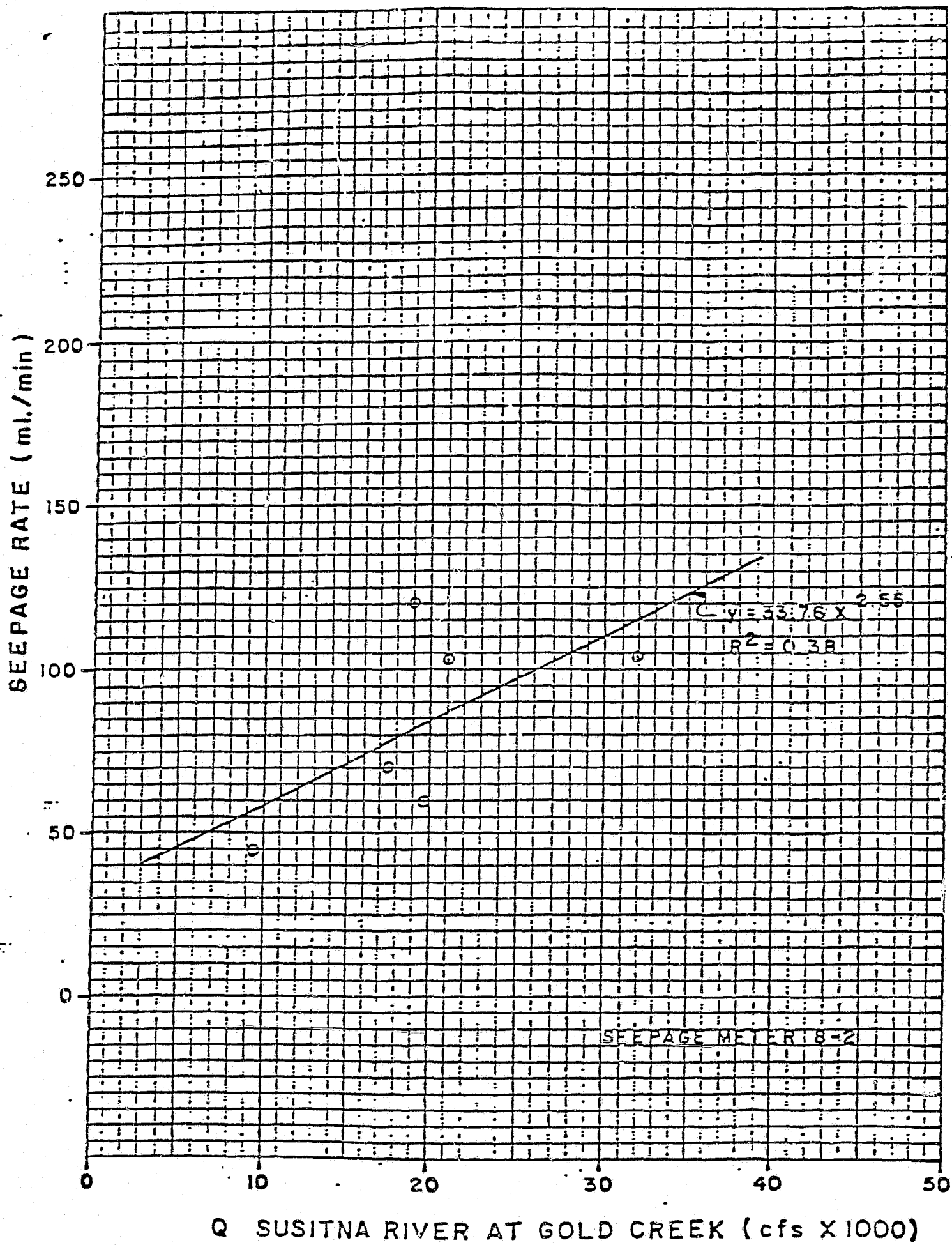
EXHIBIT 22. SEEPAGE RATE VS. MAINSTEM DISCHARGE, SEEPAGE METER 8-2.
