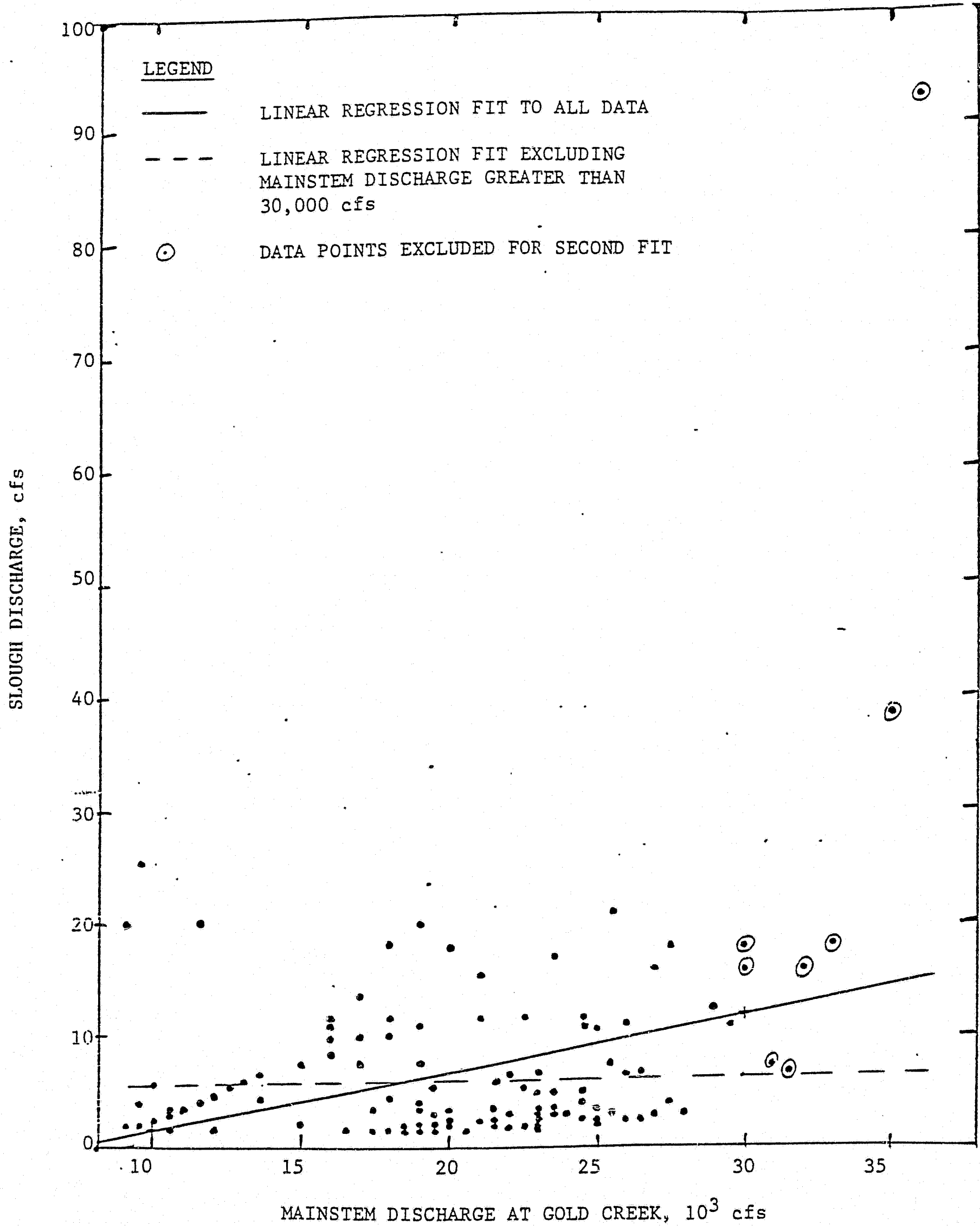
EXHIBIT 18a. SLOUGH 8A DISCHARGE VS. MAINSTEM DISCHARGE AT GOLD CREEK, SUMMER 1983
