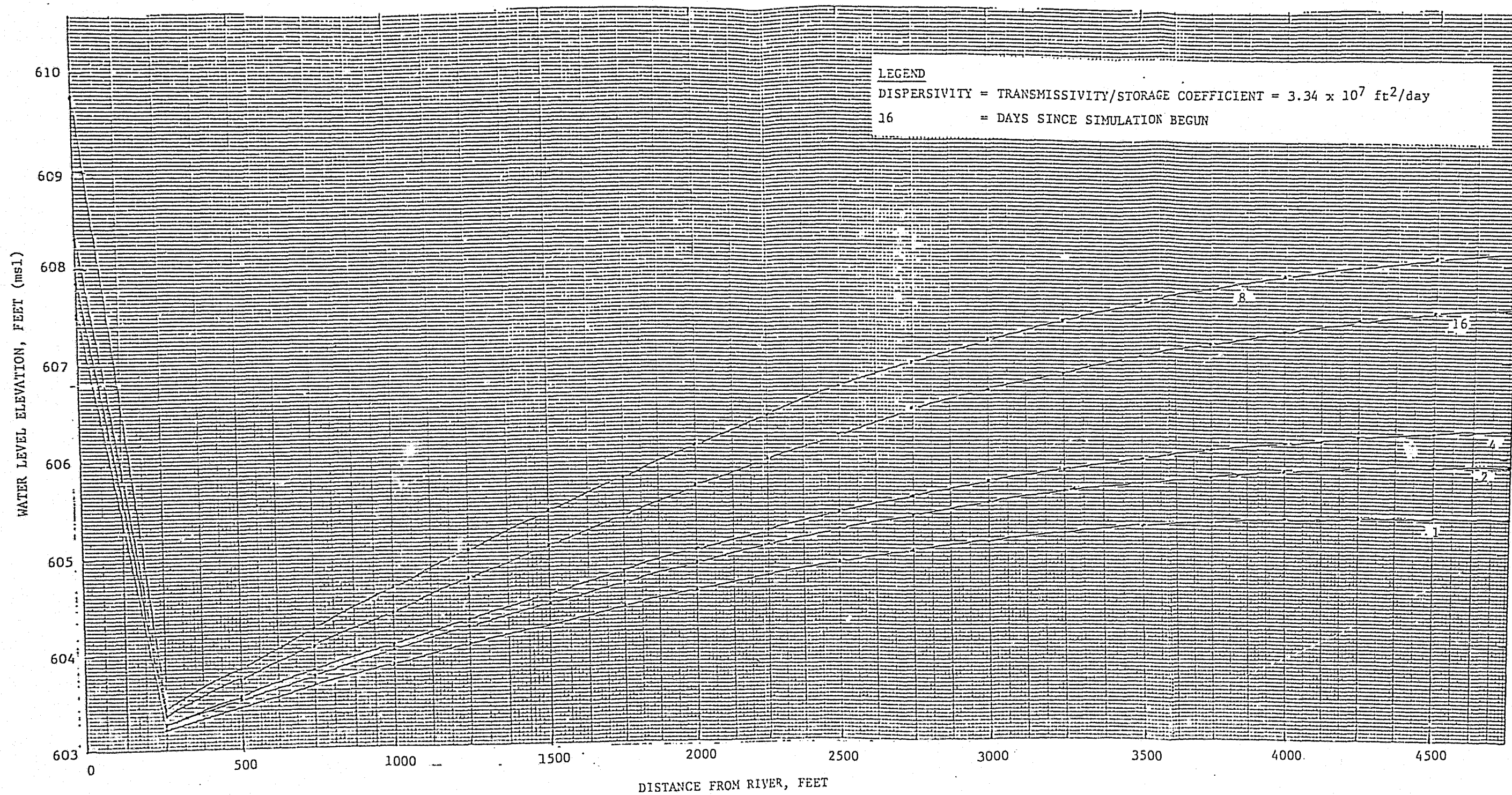
EXHIBIT 39. SIMULATED GROUNDWATER LEVELS VS. DISTANCE FROM RIVER, STORAGE COEFFICIENT = 0.0002
