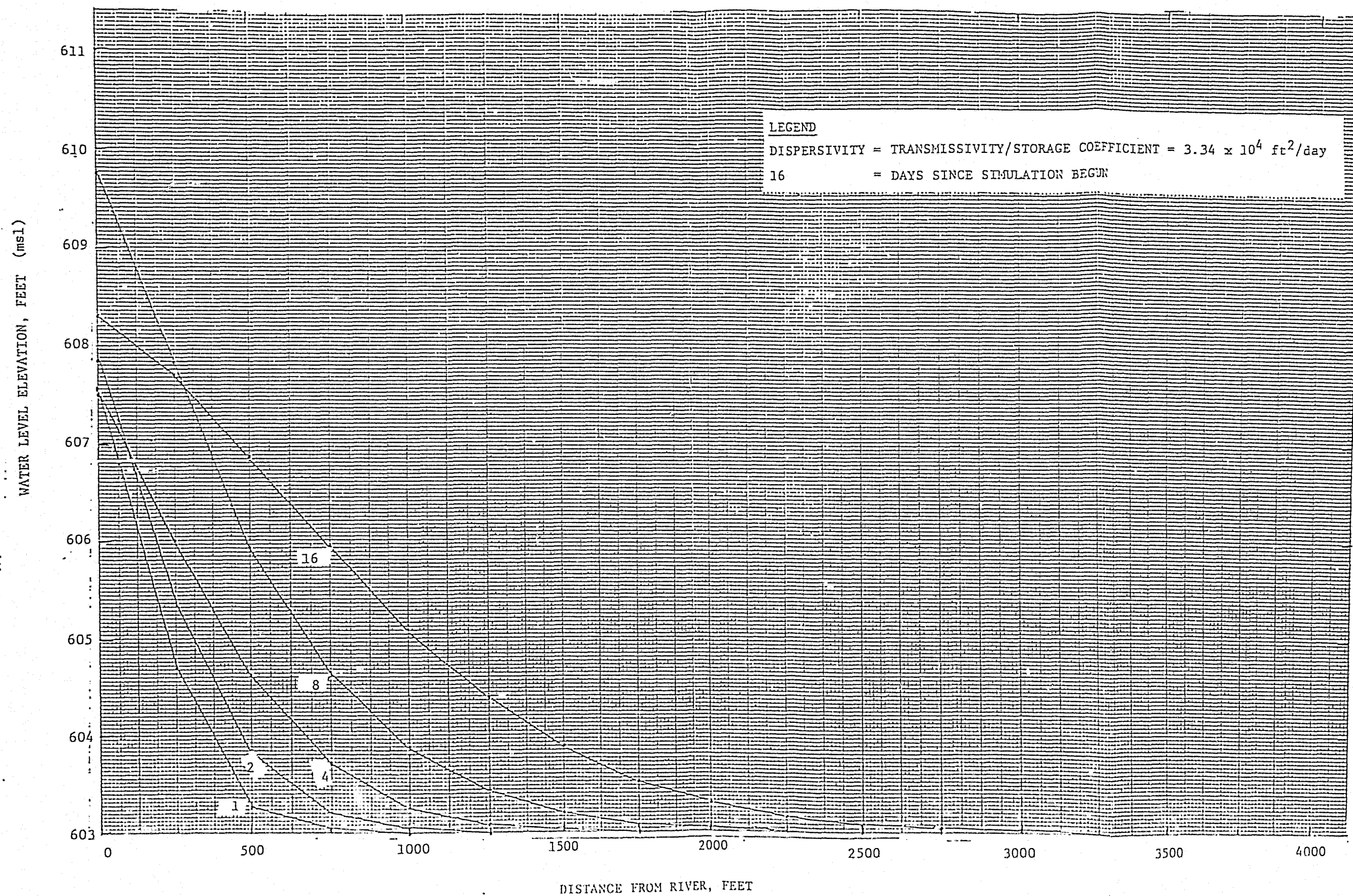
EXHIBIT 36. SIMULATED GROUNDWATER LEVELS VS. DISTANCE FROM RIVER, STORAGE COEFFICIENT= 0.2
