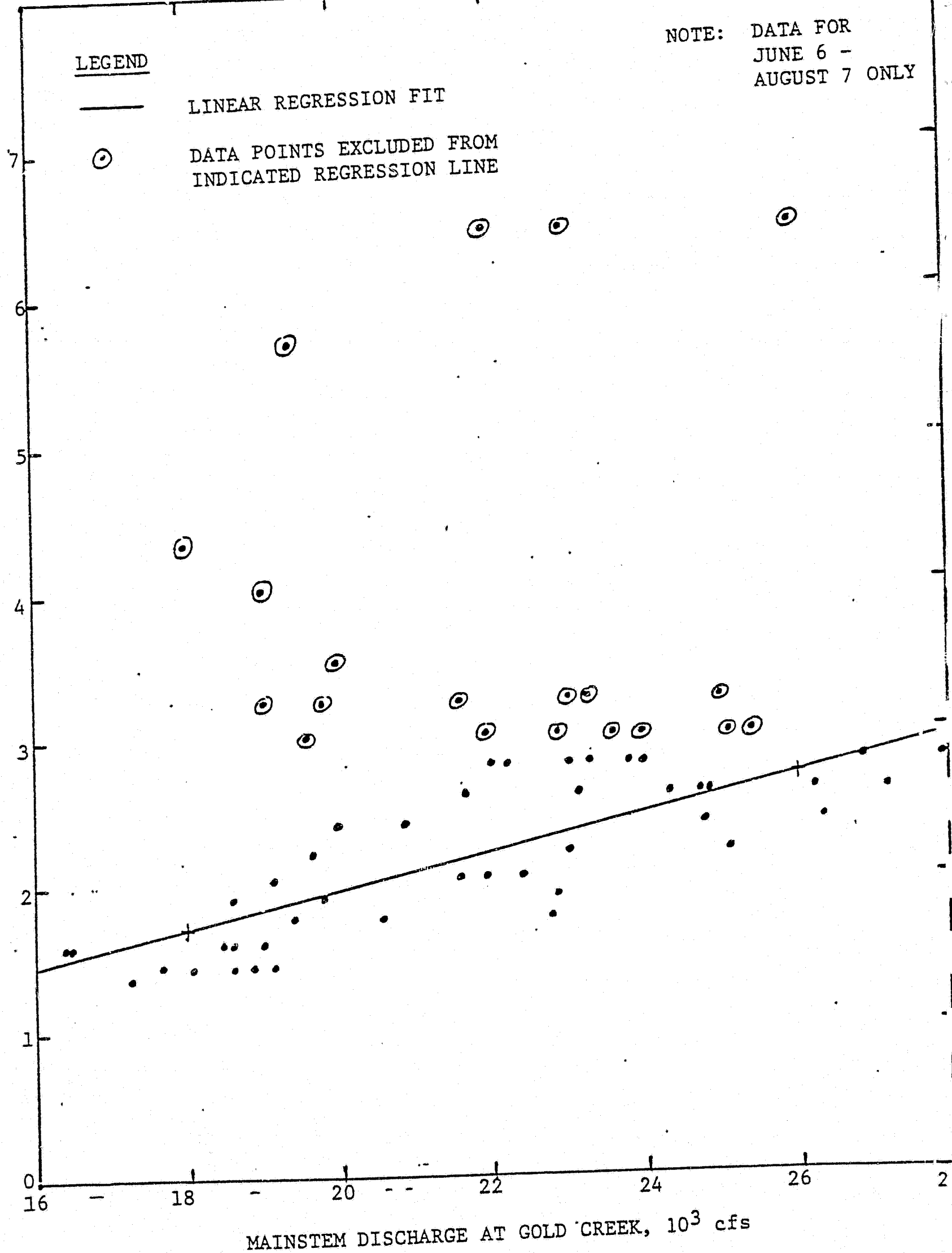
EXHIBIT 18b. SLOUGH 8A DISCHARGE VS. MAINSTEM DISCHARGE AT GOLD CREEK, SUMMER 1983
