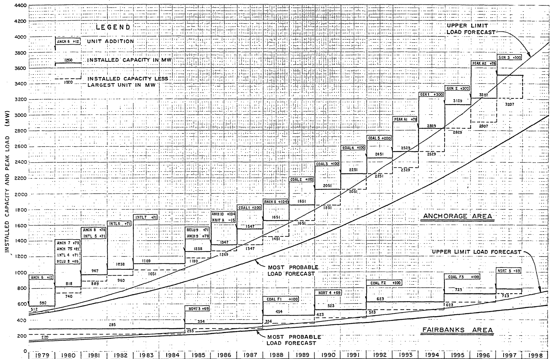
INDEPENDENT SYSTEM EXPANSION PLANS ANCHORAGE AND FAIRBANKS AREAS
