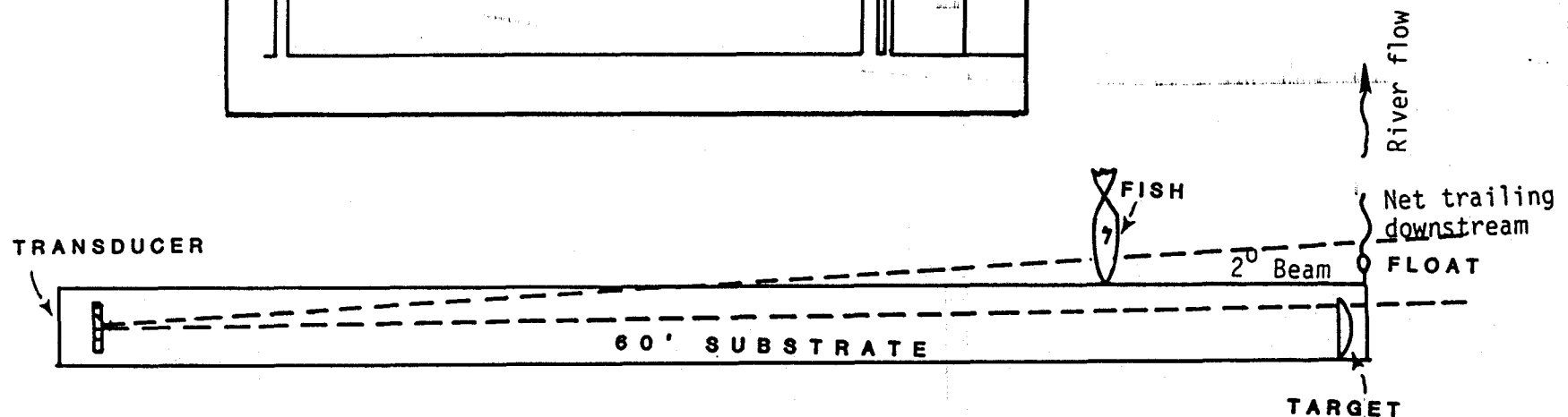
Figure 7. IMPROPERLY aimed transducer. Beamwidth switch is set to 2^\circ and scope is triggered from XM 2^\circ . Transducer is aimed too far downstream, just barely hitting target. This will cause an overcount on salmon in the last half of substrate because salmon tend to linger downstream of pipe before crossing. If salmon tend to overcount near end of substrate, this may be the problem. Reaiming the transducer more upstream will cure the problem.
