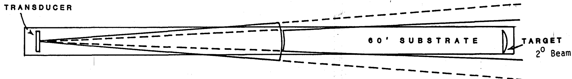
Figure 8. PROPERLY aimed transducer. Transducer beamwidth switch is set to alternate and scope is triggered from XM 4^\circ . This assumes vertical aiming of transducer is correct.
