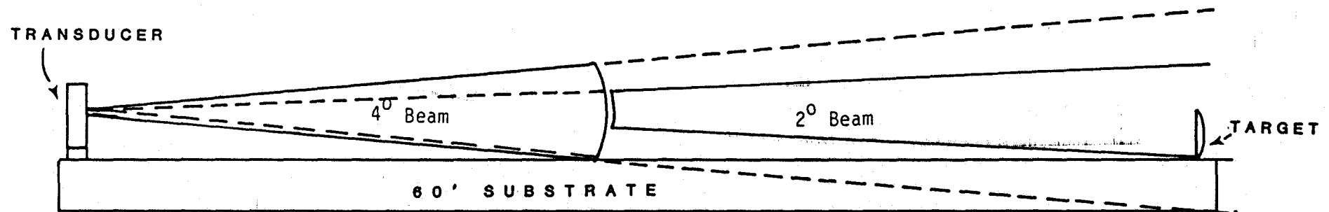
Figure 2. PROPERLY aimed transducer when beamwidth switch is set to alternate and scope is triggered from XM 4^\circ . Note 4^\circ beam is skimming surface of substrate beyond the 50% point on substrate thus causing reflections from imperfections on the substrate surface. This is okay since the 4^\circ beam will not count any echos beyond the 50% point.
