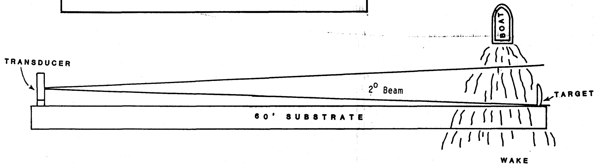
Figure 10. Properly aimed transducer but multiple echos from wake of boat. This will cause many counts, usually in outer sectors, and will probably trigger the debris indicator.
