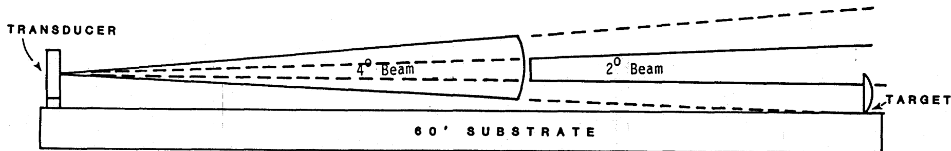
Figure 6. IMPROPERLY aimed transducer. Beamwidth switch is set to Alt. (or 4°). Scope is triggered from XM 4°, Note that beam is aimed too high, although the 4° beam solidly hits the target, the 2° beam just barely hits the target (see figure 5 for 2° scope waveform.) Fish may be missed.
