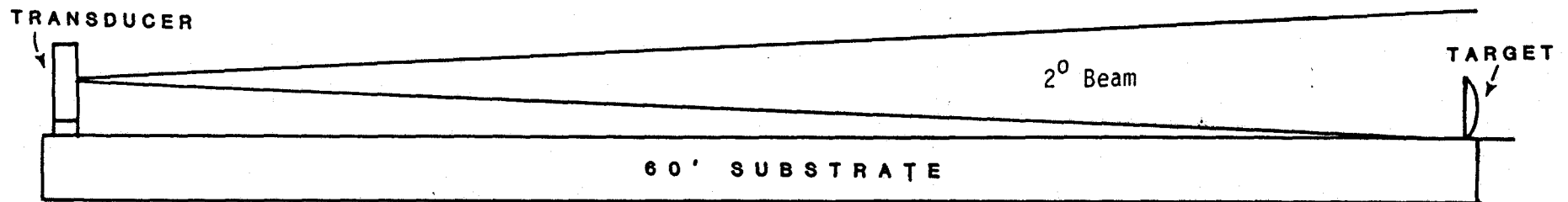
Figure 1. PROPERLY aimed transducer when beamwidth switch is set to 2^{\circ} and scope triggered from XM 2^{\circ} .
