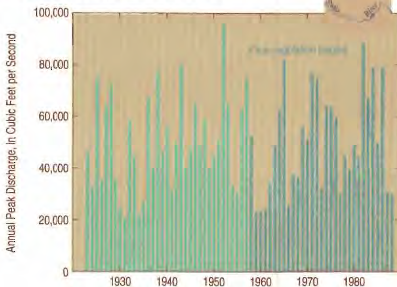
Annual flood series for the Snake River at Hells Canyon Dam, Idaho. Annual floods for 1926 to 1971 are based on correlation with data from the discontinued gaging stations Snake River at Oxbow, Oregon, and Snake River below Pine Creek at Oxbow, Oregon. Regulation by Brownlee, Oxbow, and Hells Canyon dams does not significantly affect the size or frequency of floods on the Snake River.
