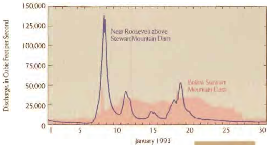
Hydrograph of the Salt River for January 1993. Peak discharge reached 143,000 \text{ft}^3/\text{s} on January 8 above Roosevelt Dam. Releases from Stewart Mountain Dam, the farthest downstream of four dams on the Salt, are dampened and protracted compared to the inflow to Roosevelt Lake.
