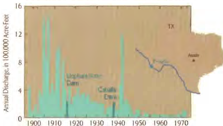
The annual volume of flow in the Rio Grande above the Rio Conchos (at Presidio, Texas) has decreased dramatically with flow regulation. Gradual increases in irrigation of the Mesilla Valley of New Mexico have reduced the annual flow volume by an order of magnitude.
