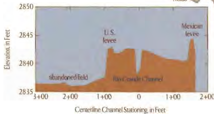
A cross section of the Rio Grande 2 km downstream from Candelaria, Texas. When measured in 1974, the channel bed was higher than its flood plain. (From Everitt, 1993)
