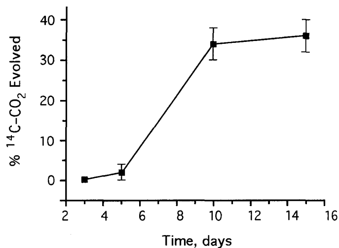
Figure 1. Mineralization of ^{14}\text{C} -labeled phenanthrene ( 10\ \mu\text{g/mL} ) with time for freshly collected Jakolof Bay sediment slurries (1:10 sediment to mineral salts medium). The values are means of duplicate points, and the range in values is shown with error bars.
