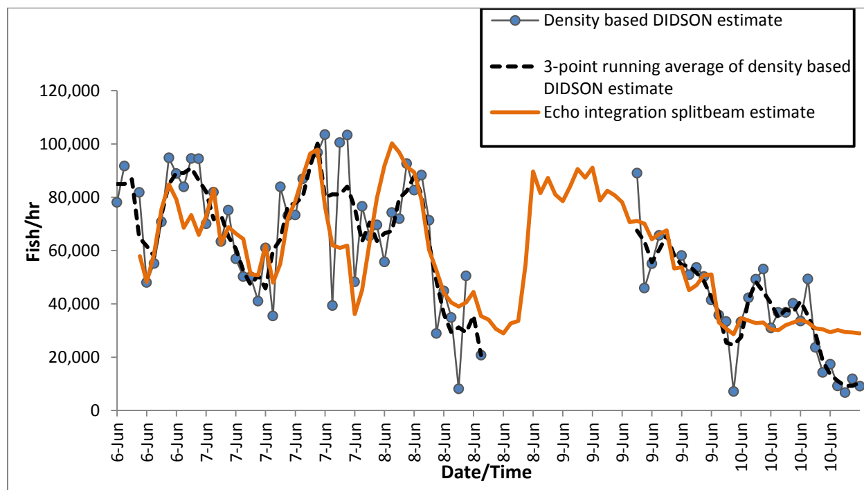
Figure 5.1-8. Comparison of density-based DIDSON and echo integration splitbeam estimates of eulachon passage at the fixed sonar site (Project River Mile 17.5) in 2013.
