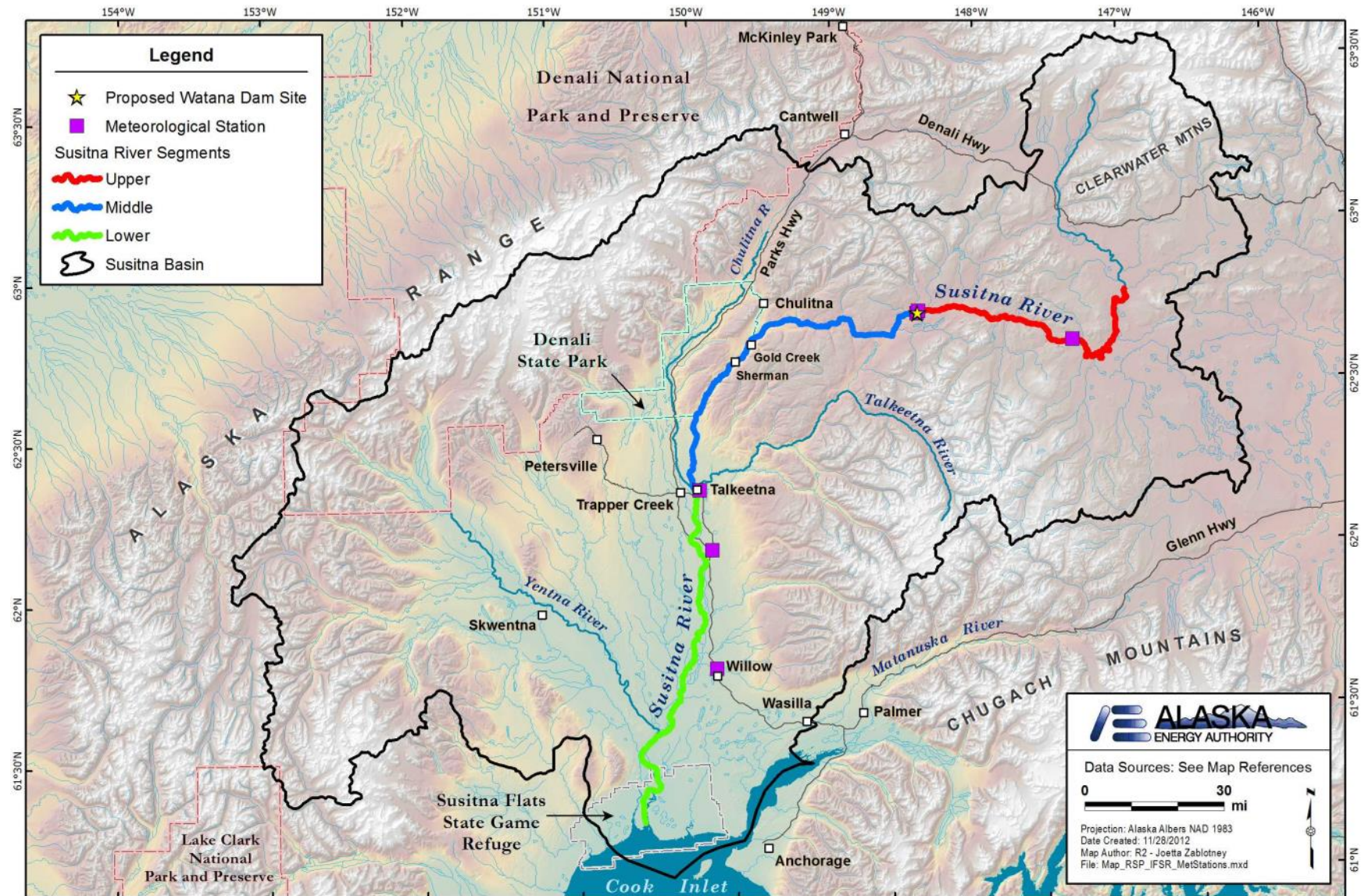
Figure 4.3-3. Susitna Project area meteorological station locations.
