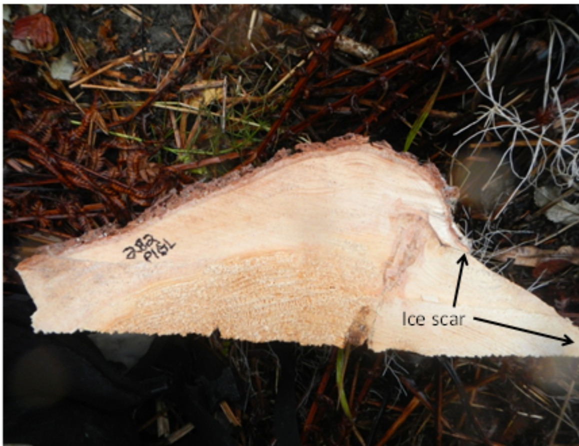
Figure 4.4-4. Tree ice scar wedge ( Picea glauca , white spruce).
