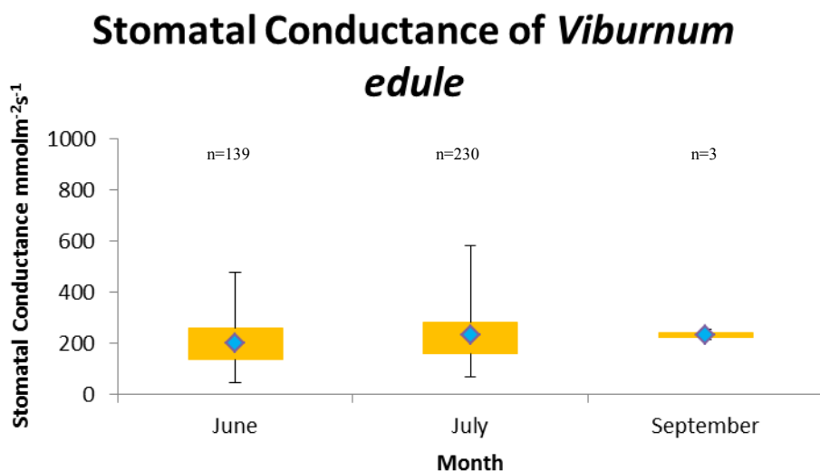
Figure 5.6-8. Seasonal Stomatal Conductance Distribution by Selected Species for (a) M. struthiopteris , and (b) V. edule .
