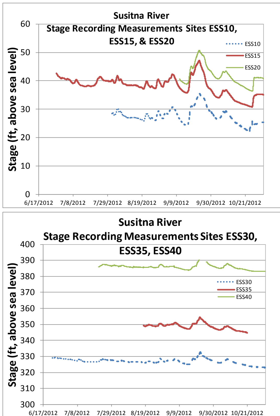
Figure 5.3-5. Stage readings for mainstem Susitna River sites ESS10-ESS40 for available data from June through October 2012. See Figure 4.4-1 for site locations.
