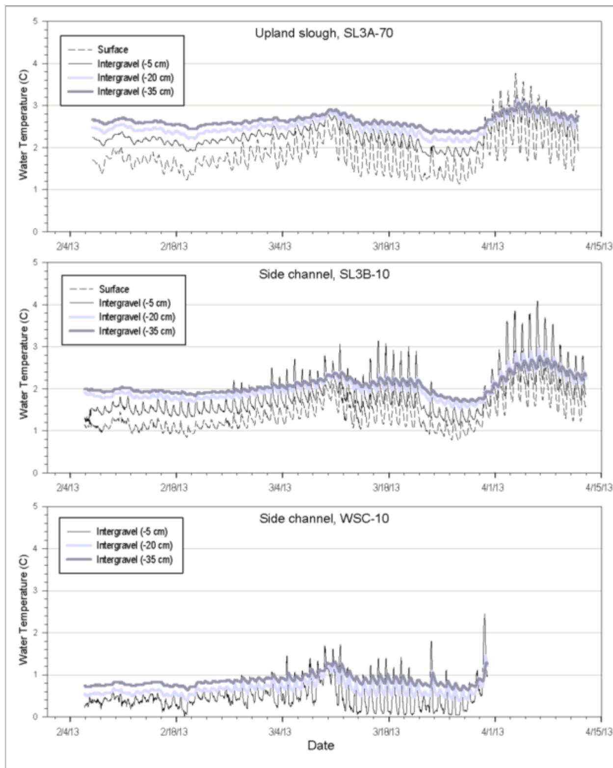
Figure 5.5-14. Water temperature recorded above the substrate surface and at intergravel depths of 5 cm, 20 cm, and 35 cm at upland slough (SL3A-70) and side channel (SL3B-10, WSC-10) continuous monitoring sites in FA-104 (Whiskers Slough) during February - April 2013. Habitat designations are based on 2012 Middle Susitna River remote line habitat mapping (HDR 2013).
