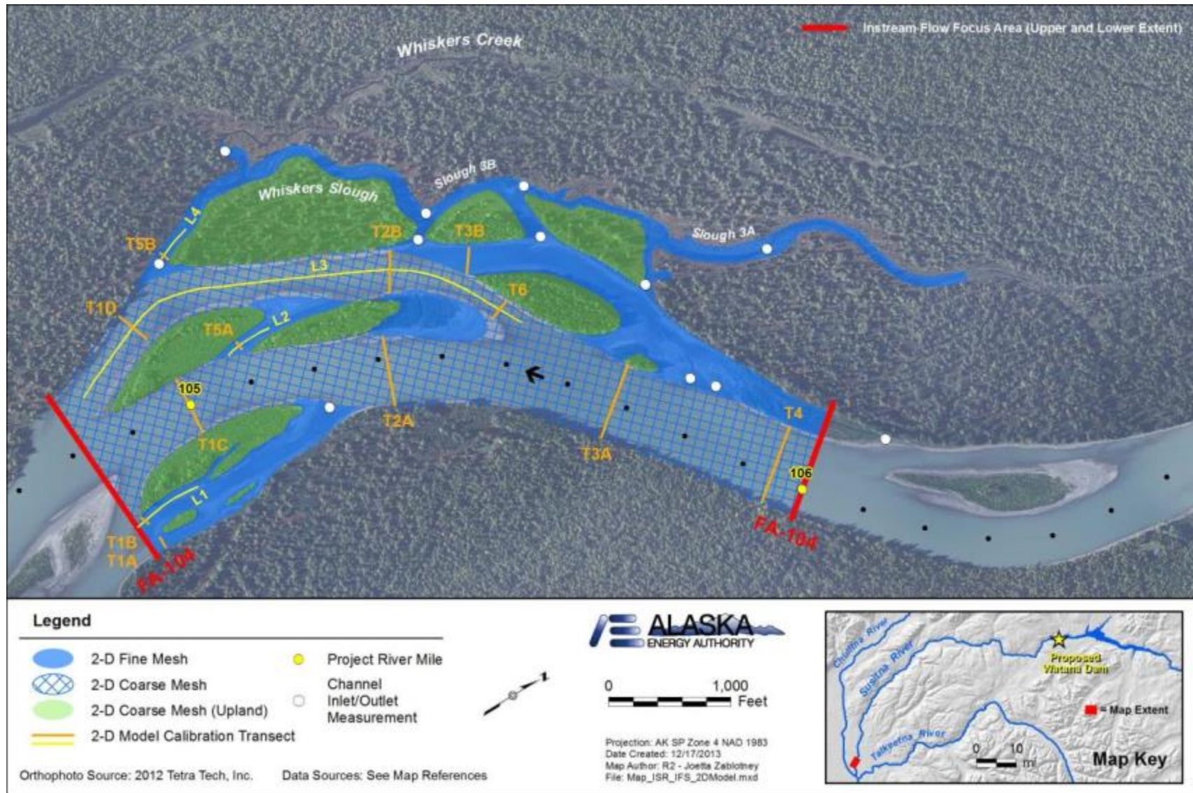
Figure 5.6-1. FA-104 (Whiskers Slough) showing fine and coarse mesh overlays, channel inlet and outlet measurement locations, and alignment of 2013 calibration transects.
