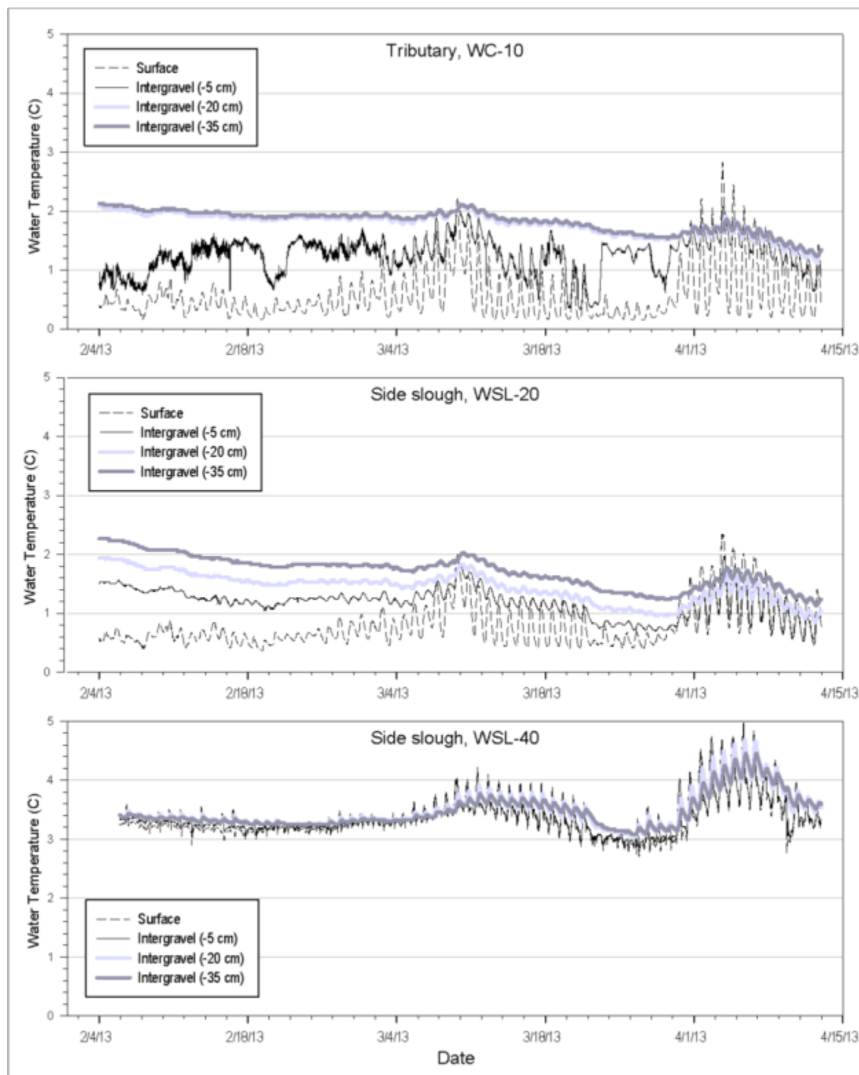
Figure 5.5-15. Water temperature recorded above the substrate surface and at intergravel depths of 5 cm, 20 cm, and 35 cm at tributary (WC-10) and side slough (WSL-20, WSL-40) continuous monitoring sites in FA-104 (Whiskers Slough) during February - April 2013. Habitat designations are based on 2012 Middle Susitna River remote line habitat mapping (HDR 2013).
