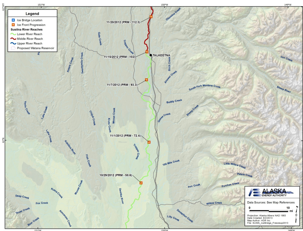
Figure 2.1-4. 2012 Ice Front Progression and Ice Bridge Locations–Middle Susitna River.
