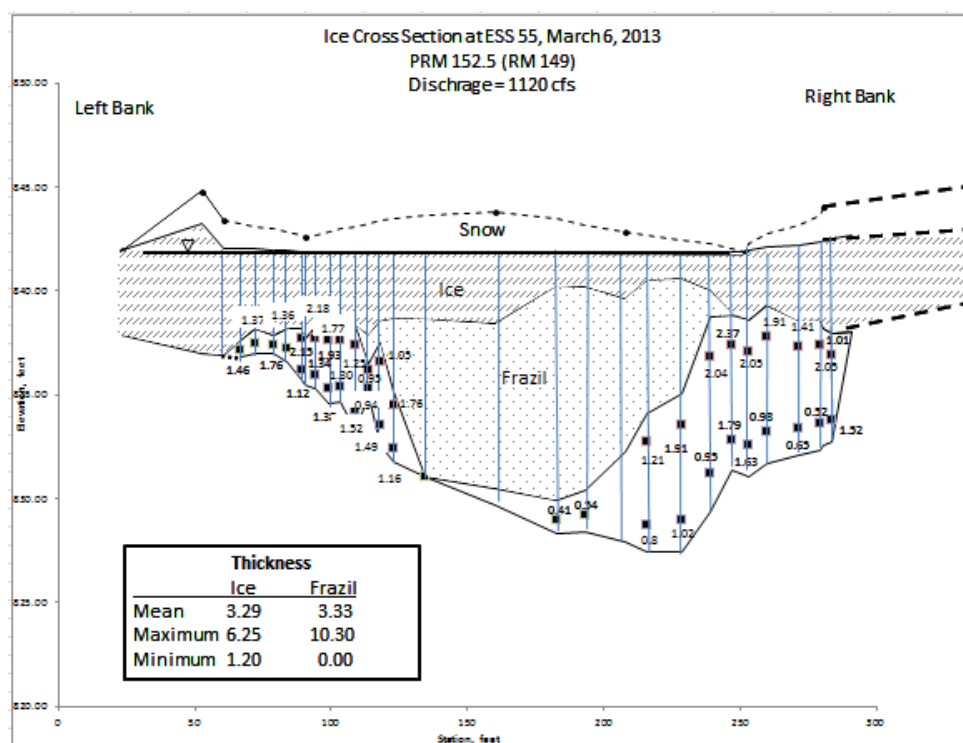
Figure 5.1-8. Cross Sectional Diagram of ESS55. HDR Alaska.
