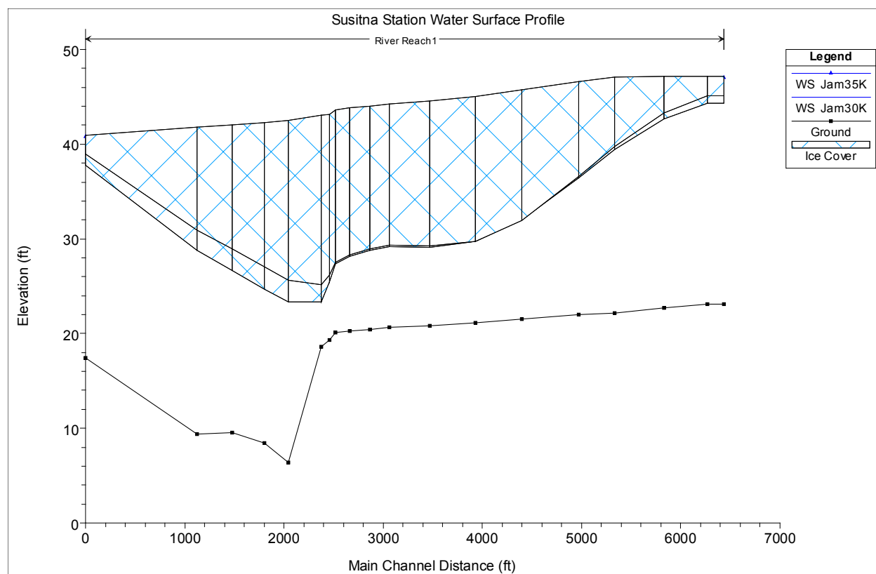
Figure 4.3-3. HEC-RAS profile plot of the modeled reach at Susitna Station at the completion of the freeze-up period at discharge levels of 30,000 to 35,000 cfs.
