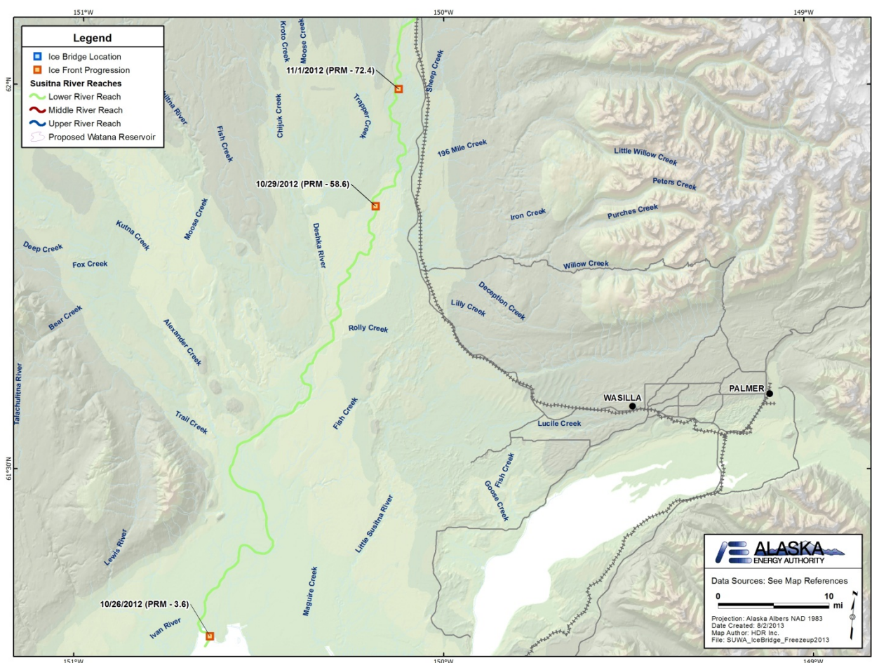
Figure 2.1-1. 2012 Ice Front Progression and Ice Bridge Locations—Lower Susitna River.
