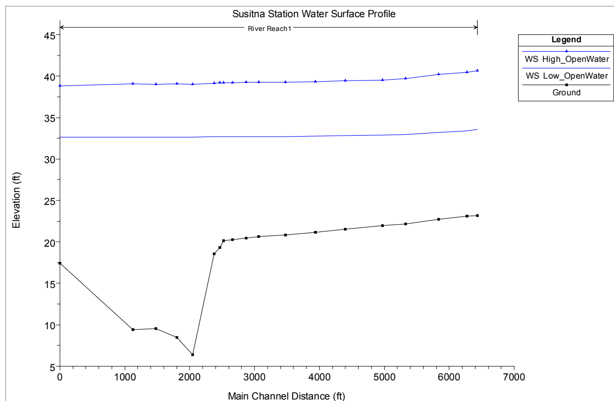
Figure 4.3-1. HEC-RAS profile plot of the modeled reach at Susitna Station at the start of the freeze-up period at discharge levels of 11,000 and 58,000 cfs.
