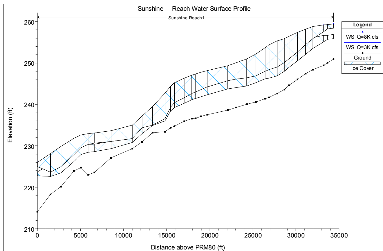
Figure 4.2-2. HEC-RAS profile plot of the modeled reach near Sunshine at the completion of the freeze-up period at discharge levels of 3,000 and 8,000 cfs with an ice jam.
