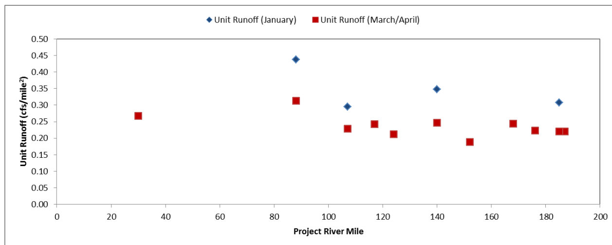
Figure 5.1-15. Unit Runoff Plotted Against Project River Mile for the January and March/April Field Events
