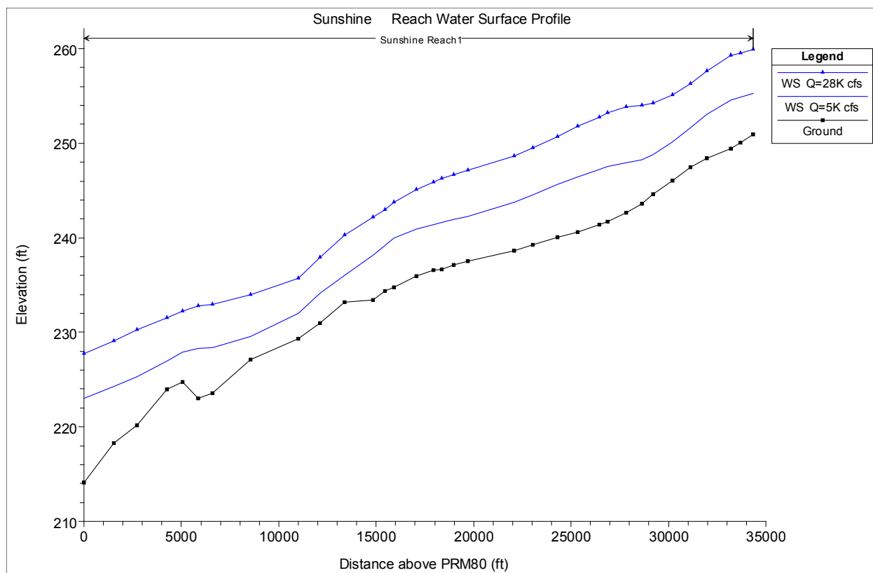
Figure 4.2-1. HEC-RAS profile plot of the modeled reach near Sunshine at the start of the freeze-up period at discharge levels of 5,000 and 28,000 cfs.
