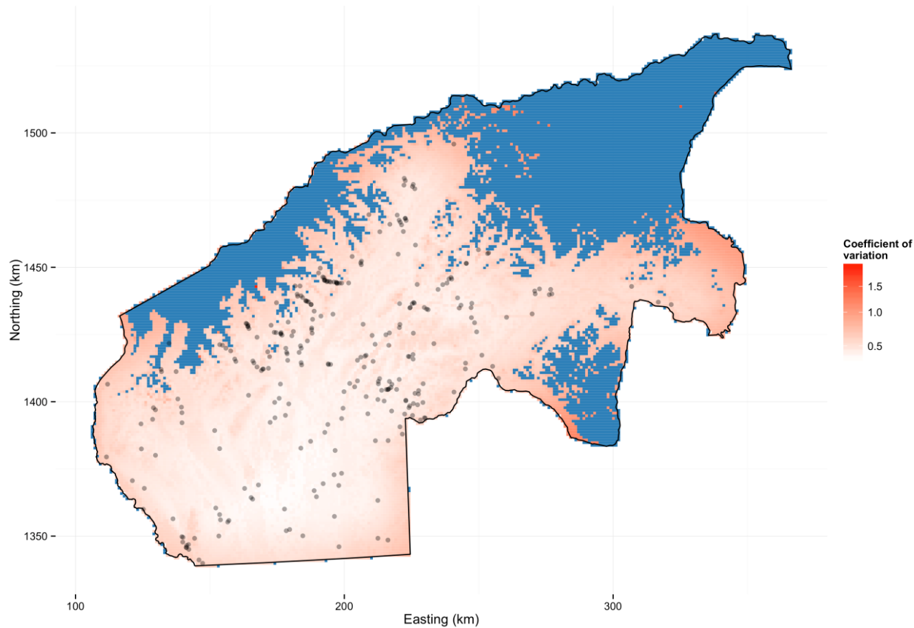
Figure 5.1-6. Density Surface Map of the Coefficient of Variation of the Predicted Number of Black Bears per 1-km 2 .
