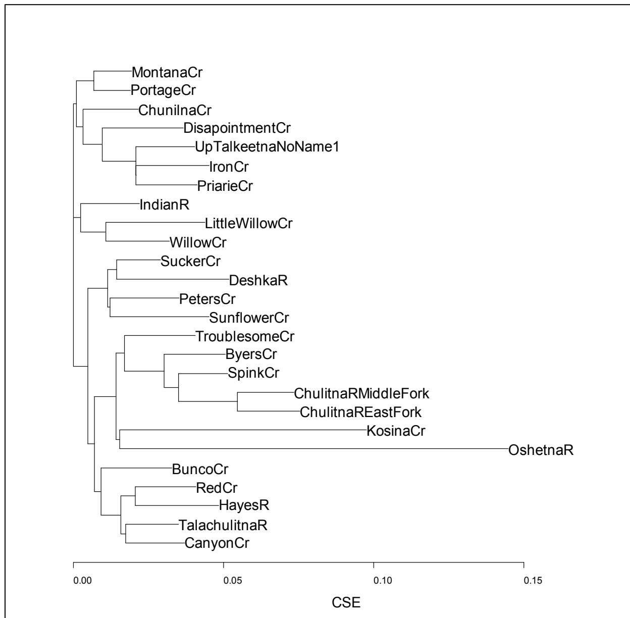
Figure B3. Neighbor-joining tree based on Cavalli-Sforza and Edwards genetic distances among collections of Chinook salmon collected from the Susitna and Yentna River drainages.
