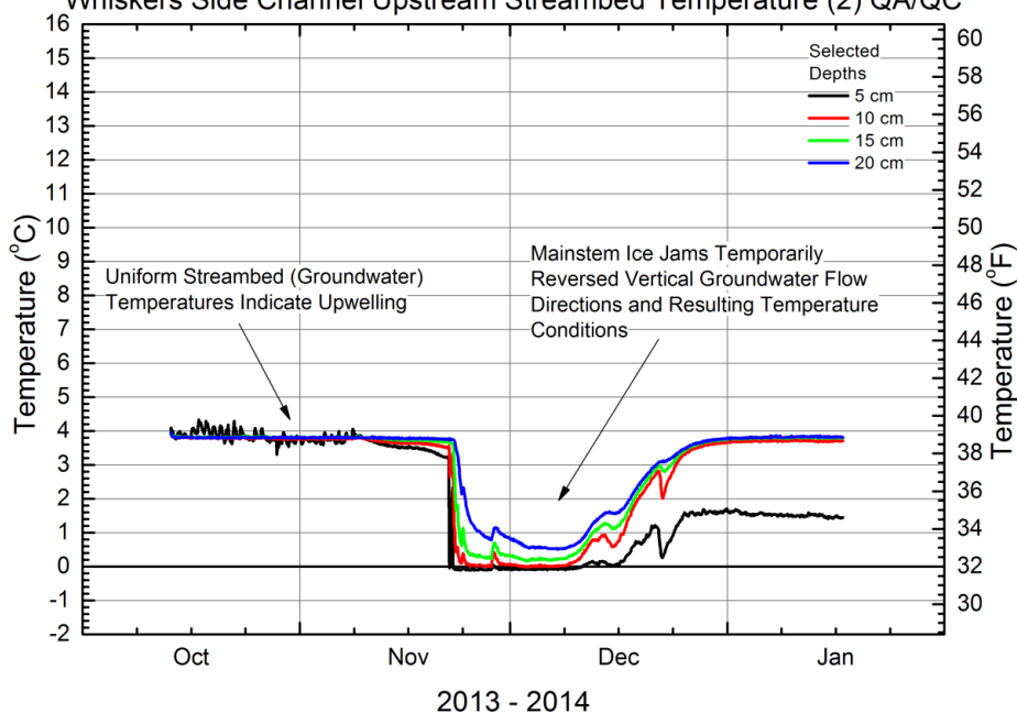
Figure 5.7-10. Example of streambed temperature measurement in the Aquatic Transect in FA-104 (Whiskers Slough) from groundwater station ESGFA104-10. This is the upstream streambed profile sensor at the station (Figure 4.5-19). This station is located at the upstream end of Whiskers Side Channel.
