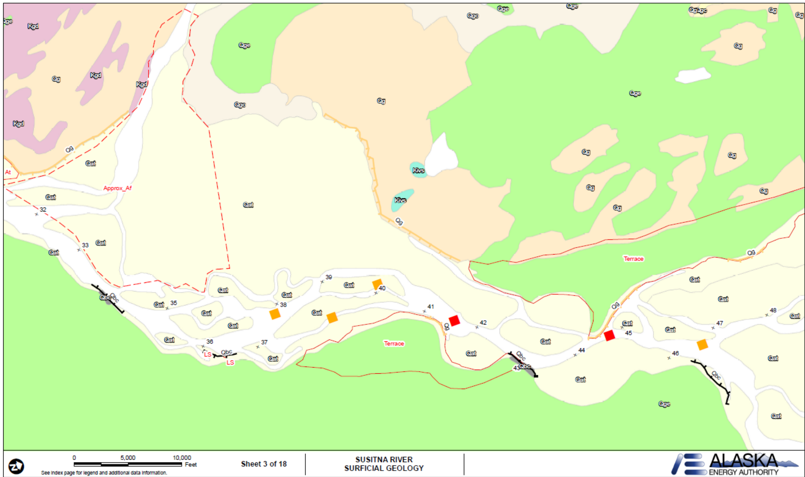
Figure A.1-4: Susitna River Surficial Geology Mapbook Sheet 3.
