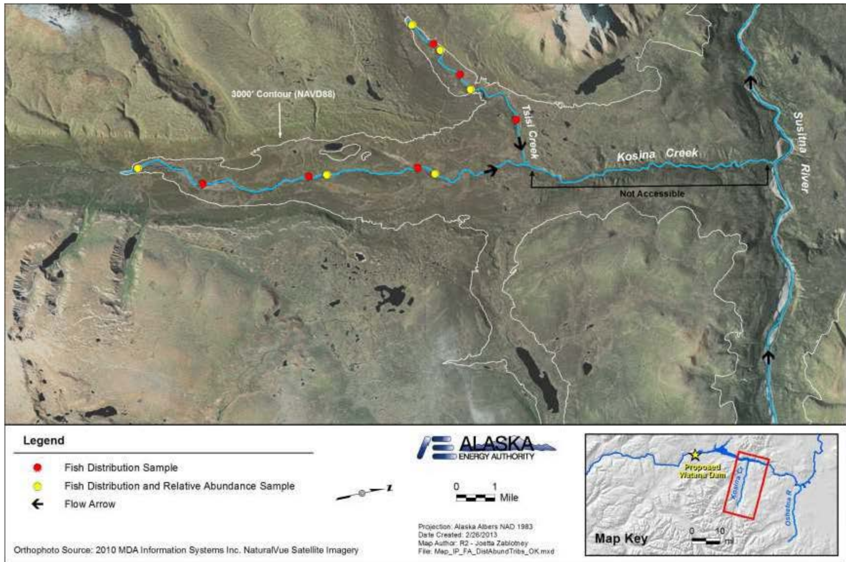
Figure 5.2-6. Map showing sample locations in Kosina and Tsisi creeks. Dots represent locations of 800 meters (Kosina Creek) or 400 meters (Tsisi Creek) sampling units.
