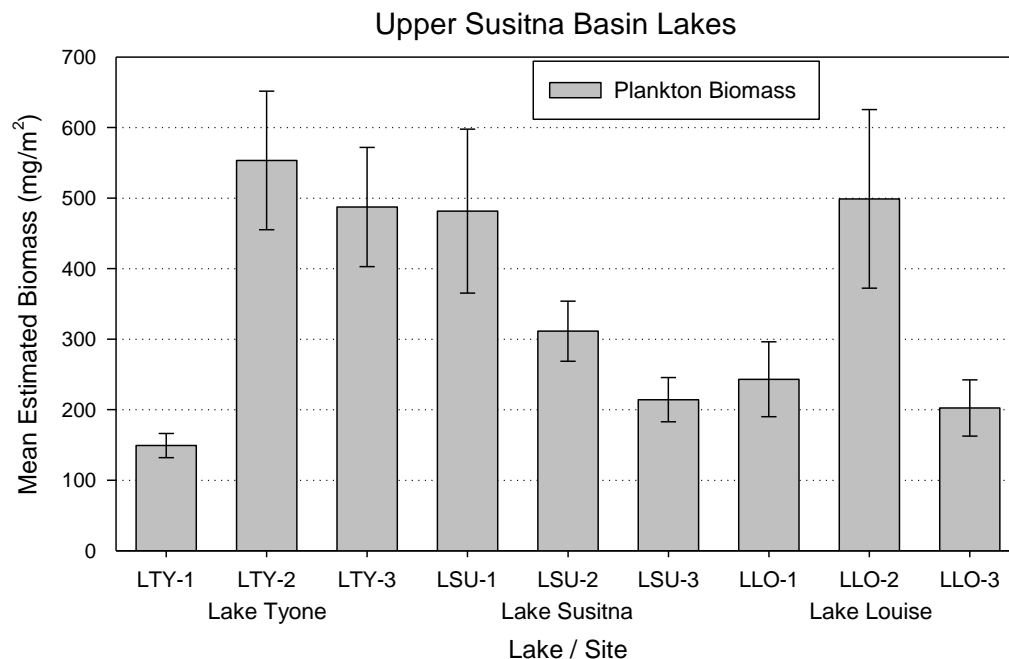
Figure 5.8-22. Mean plankton tow dry weight biomass estimates (mg/m 2 ) from vertical tow net samples (n=5) collected in July 2014 for sites within three lakes in the Upper River Segment of the Susitna River for the River Productivity Study. Error bars represent 95-percent confidence intervals.
