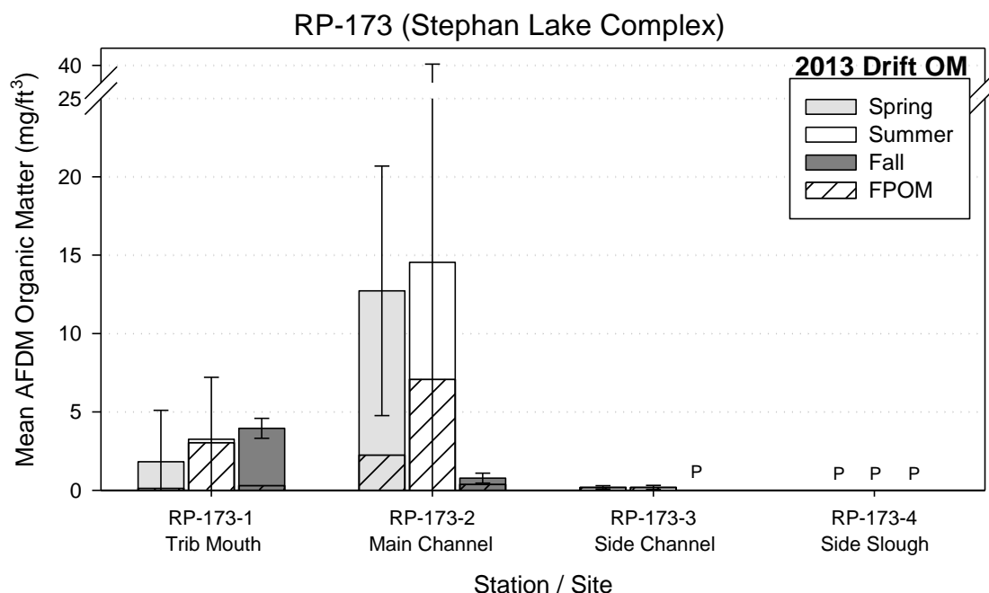
Figure 5.6-5. Drift (seston) organic matter estimates (mg/ft 3 ) from drift samples (n=2) collected in 2013 during three sampling events for sites within the Stephan Lake Complex Focus Area (FA-184) in the Middle River Segment of the Susitna River for the River Productivity Study. Error bars represent 95-percent confidence intervals. “P” indicates plankton tow samples were taken, and no organic matter was collected.
