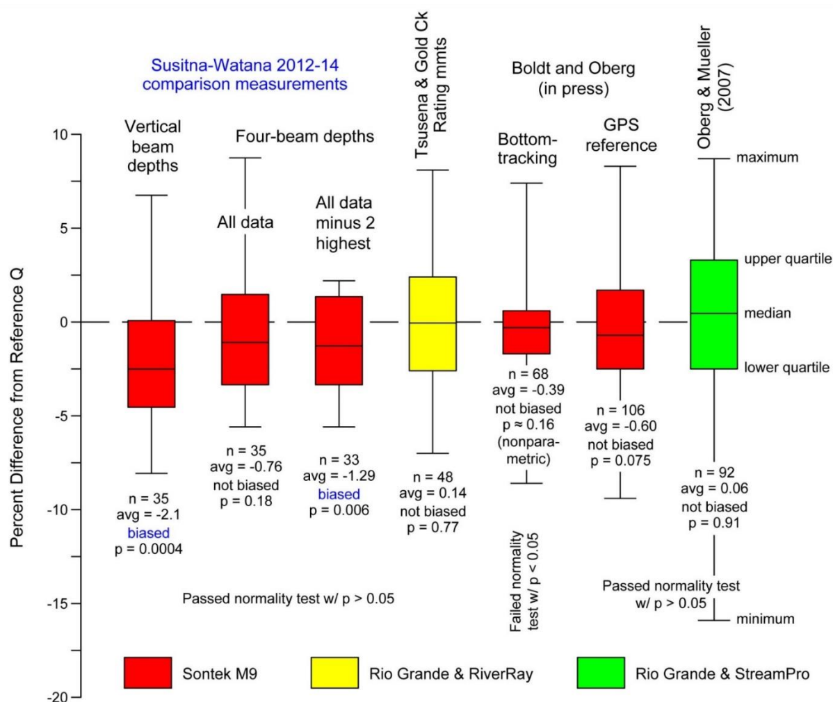
Figure 10. Comparison measurements, rating measurements, and published Acoustic Doppler Current Profiler accuracy data.
