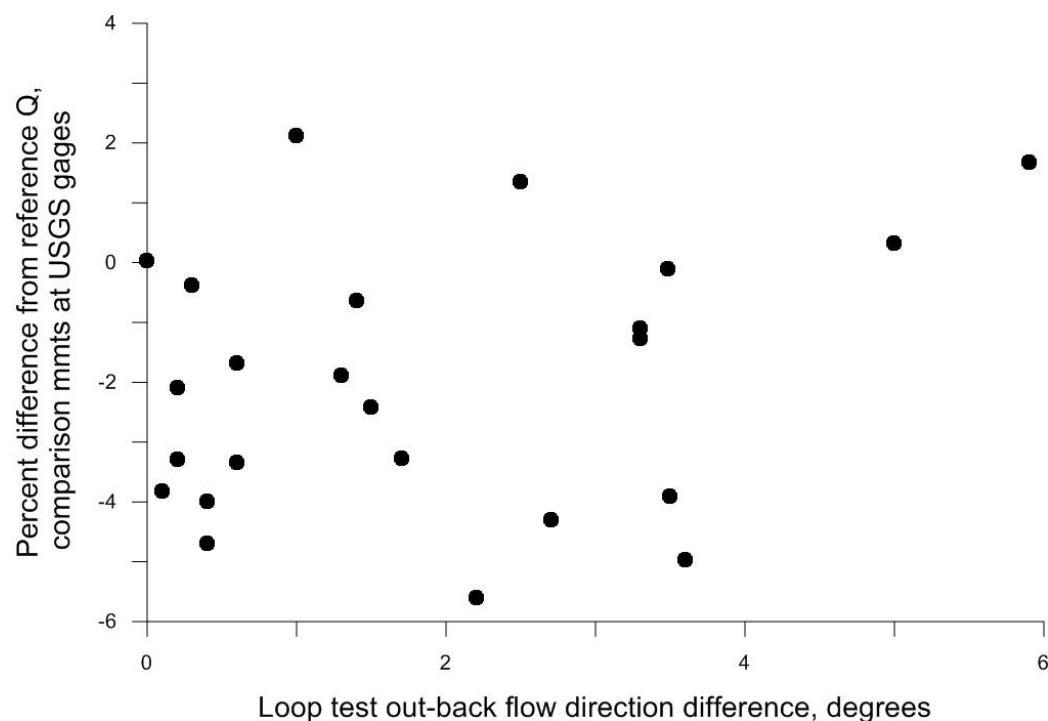
Figure 6. USGS comparisons measurement accuracy vs. out-back difference completed on the Susitna River as part of Acoustic Doppler Current Profiler measurements in 2014.
