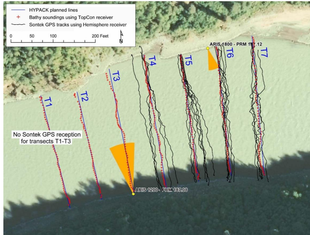
Figure 14. SonTek vs. TopCon GPS tracks at PRM 187.2 in the Susitna River.
