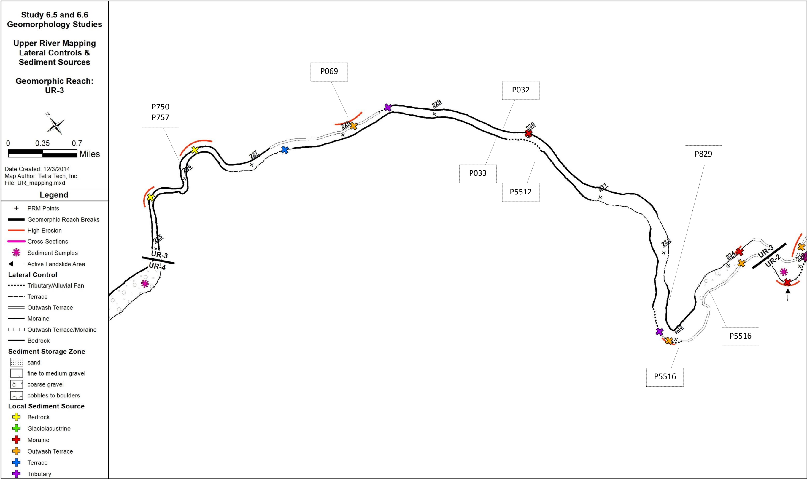
Figure 5.1-6: Upper River Lateral Control and Sediment Source Mapping with illustrative photo numbers noted (See Appendix A for photos) for geomorphic reach UR-3.
