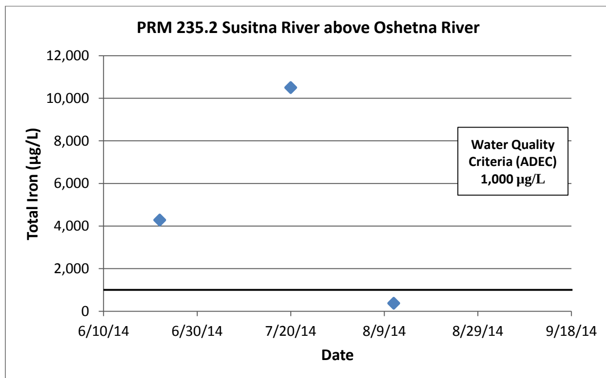
Figure 6.3-1. Surface Water Concentrations for Total Iron at PRM 235.2 (2014)
