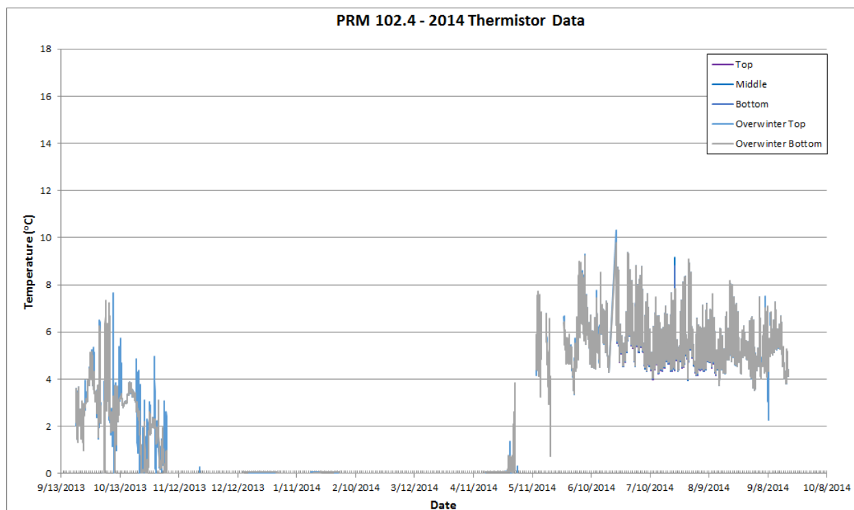
Figure 5.2-4. Thermistor Data at Chulitna River (Winter 2013 through Summer 2014)
