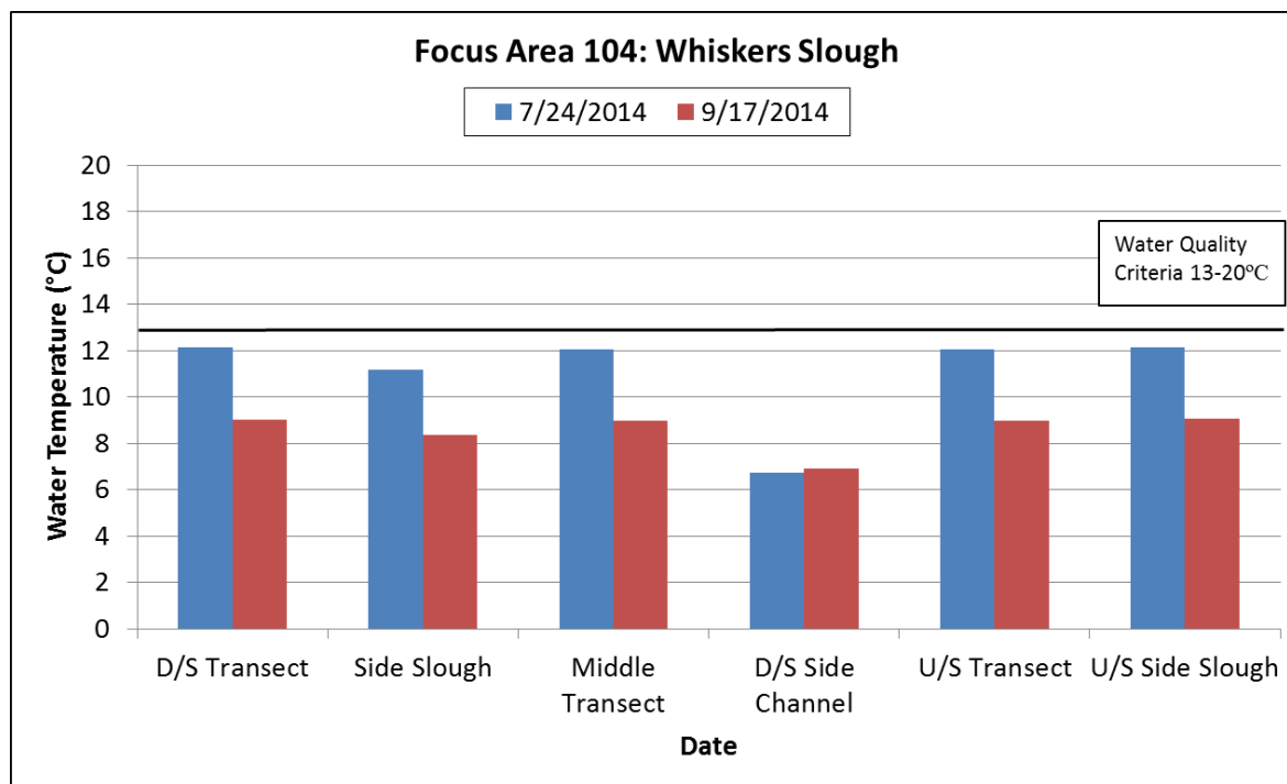
Figure 5.4-199. FA-104 (Whiskers Slough) Temperature Field Measurements (Summer 2014)
