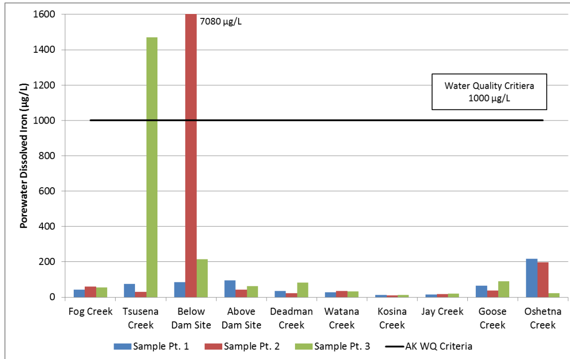
Figure 5.5-3. Porewater Dissolved Iron Concentrations (2014)
