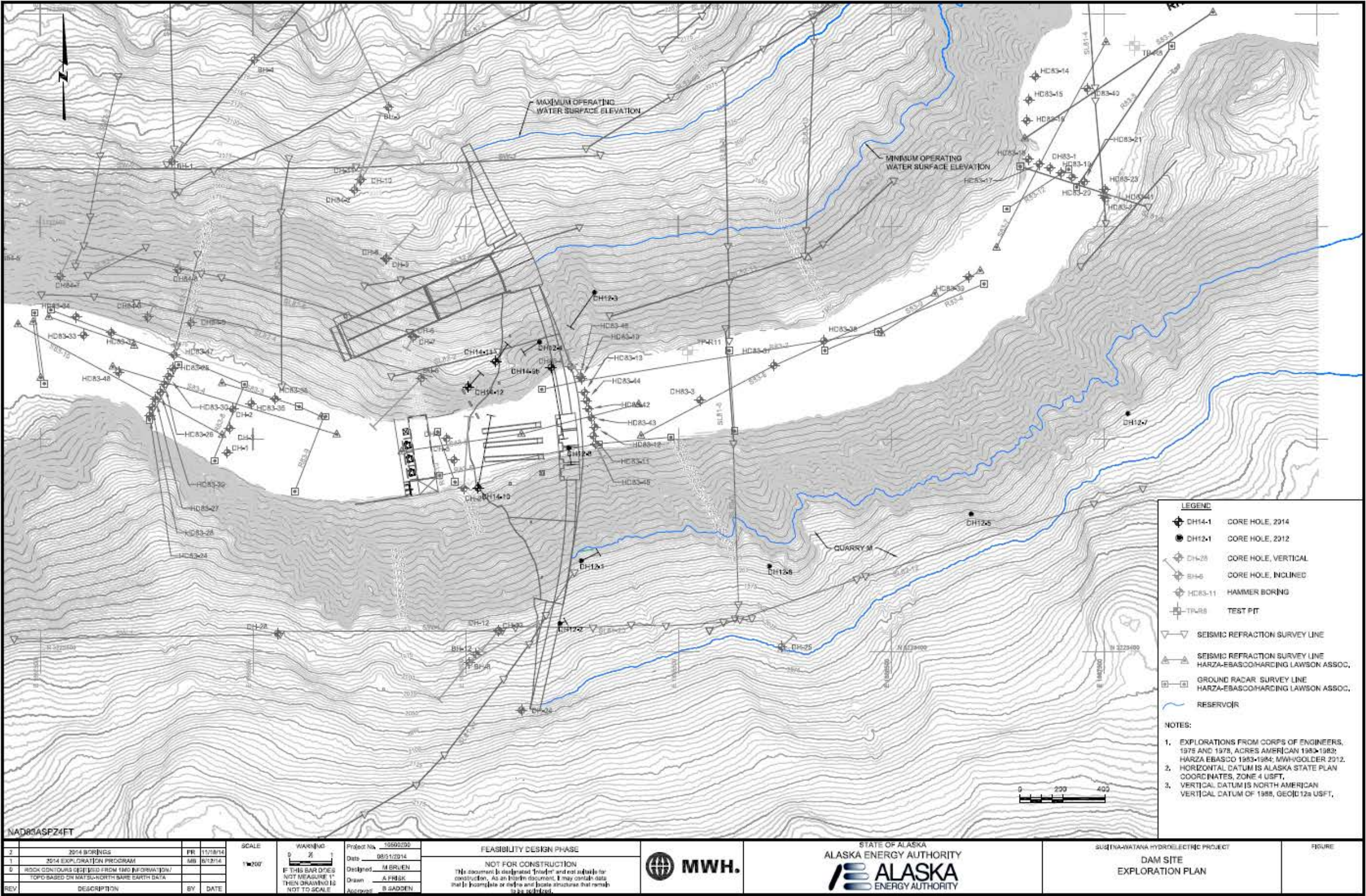
Figure 4.3-1. Dam Site Exploration Plan – 2014
