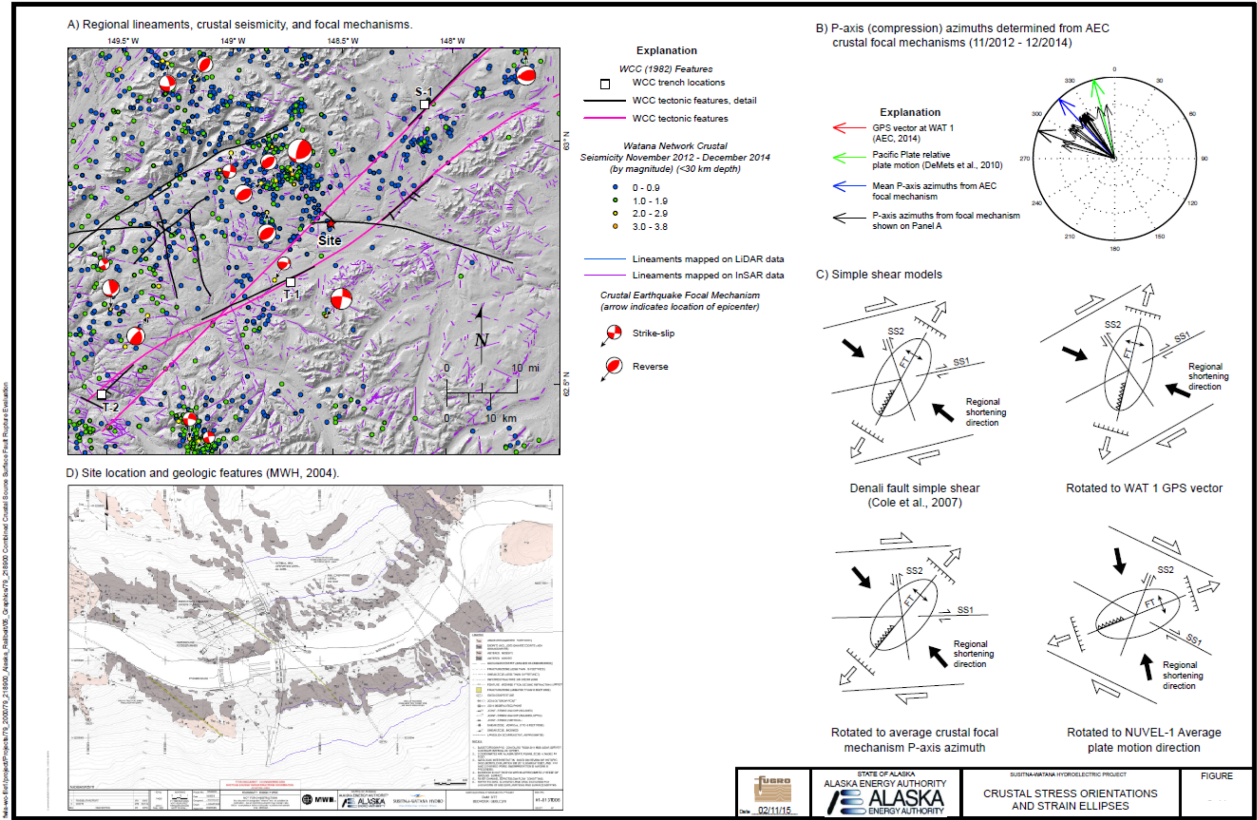
Figure 5.5-1. Crustal Stress Orientations and Strain Ellipses (Fugro 2015b)
