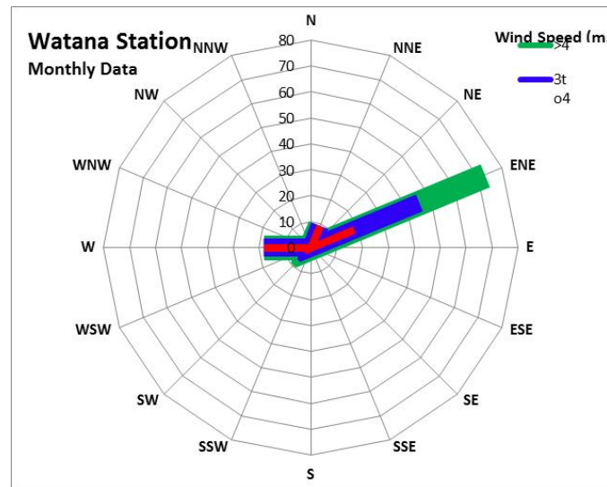
Figure 8.10-1. Wind Rose Full Year
