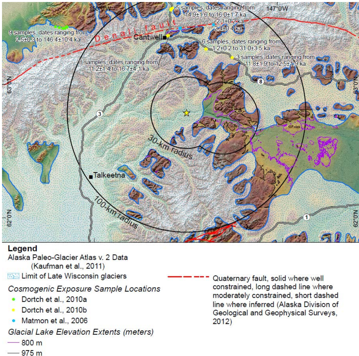
Figure 6.3-14. Late Wisconsin Glacial Limits and Age Control (Kaufman et al. 2011)
