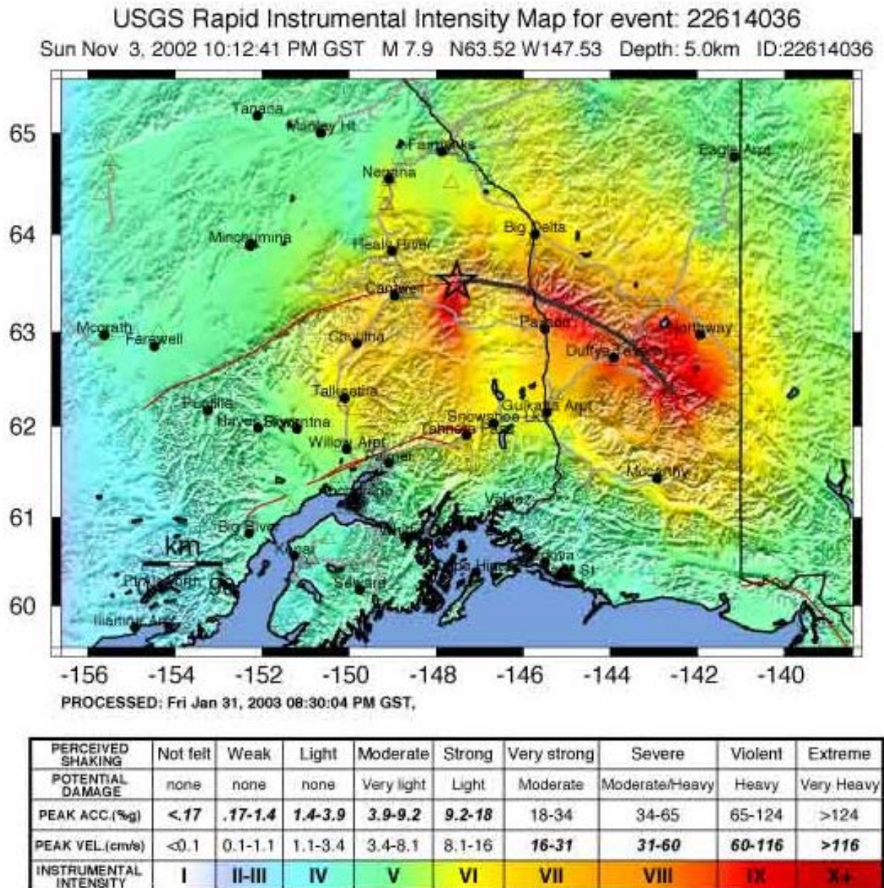
Figure 6.3-17. USGS Shake Map for 2002 Denali Earthquake (USGS)
