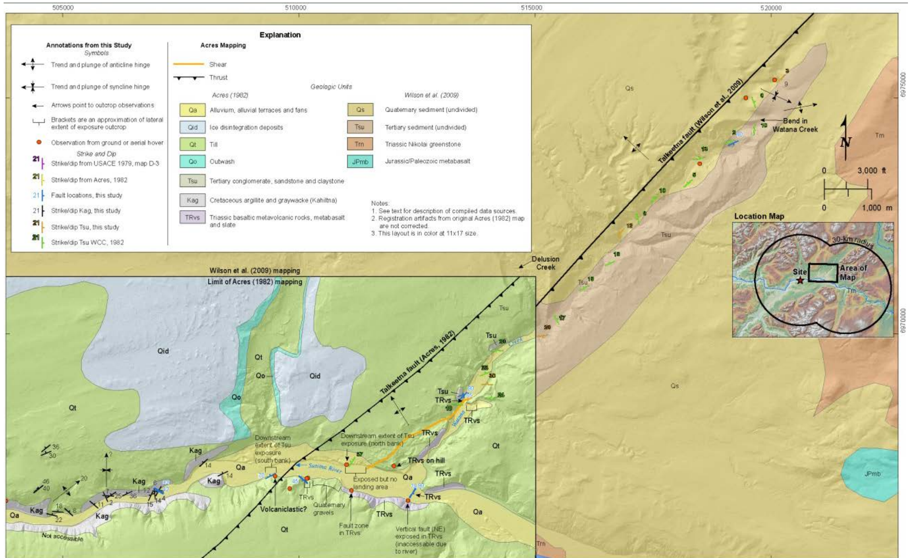
Figure 6.3-7. Acres Geologic Map Updated With Observations from 2014 (Fugro 2014)
