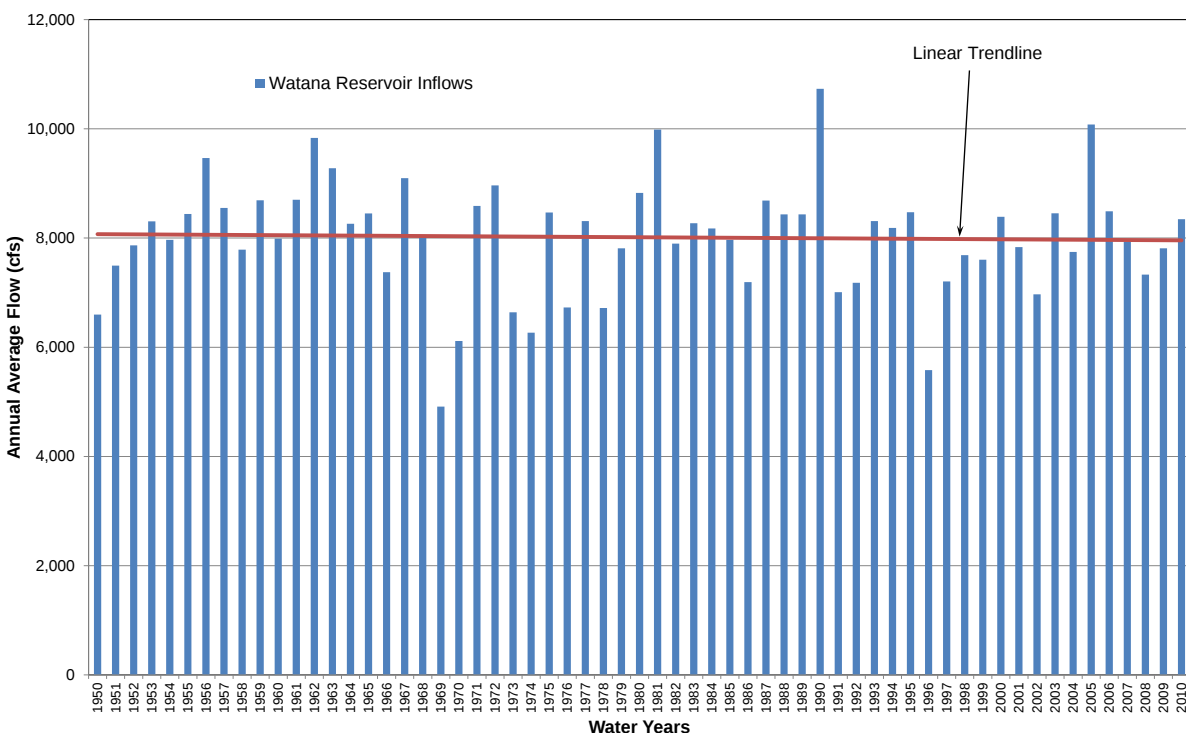
Figure 6.2-13. Watana Reservoir Annual Inflows and Trendline
