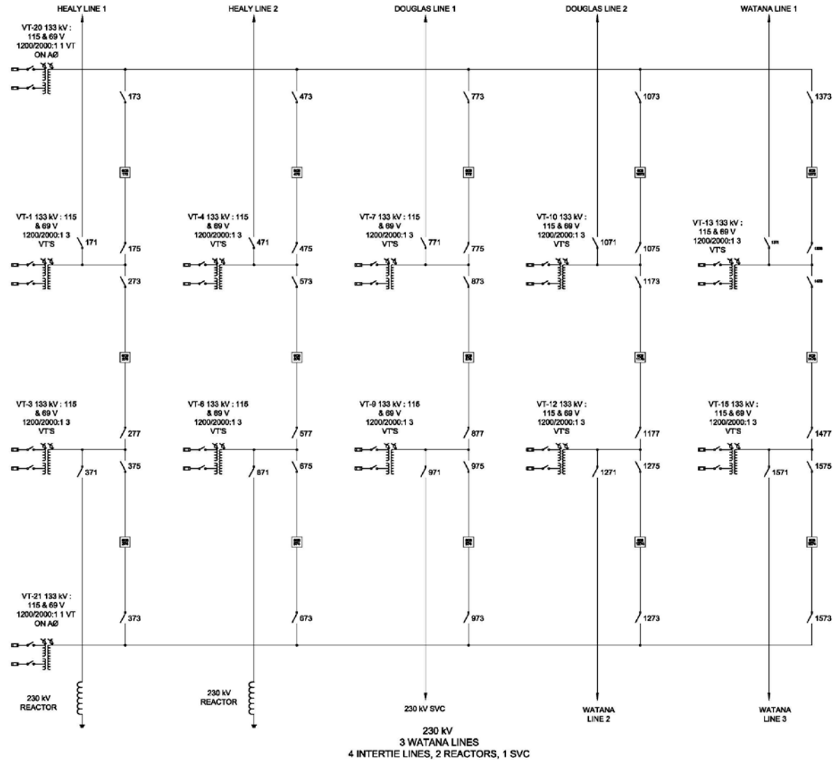
Figure 11.4-1. Typical Intertie Connection
