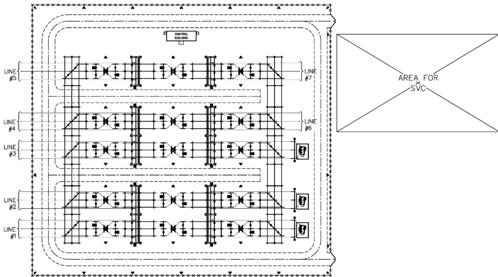
Figure 11.4-2. Typical Layout of the Substation Interconnection
