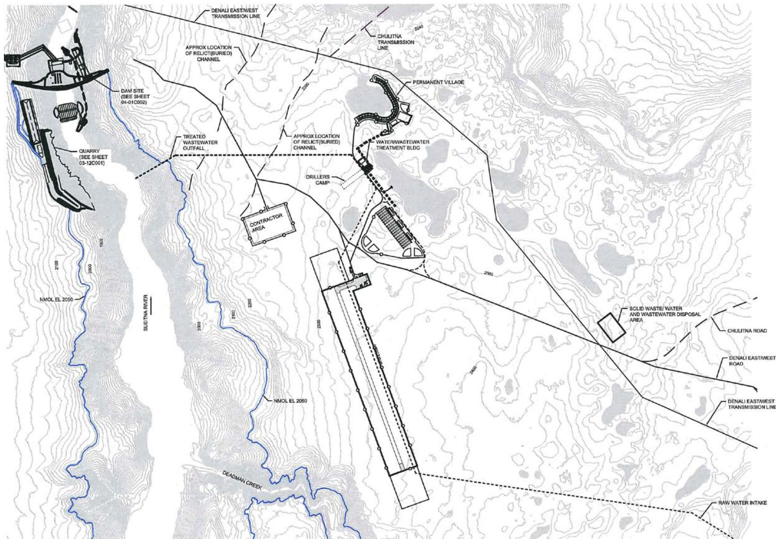
Figure 1.1-3. Site Plan
