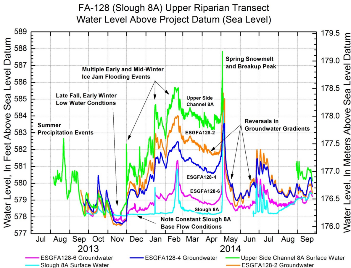
Figure 27. Water level data for Upper Side Channel 8A, Slough 8A, and groundwater wells between the two surface-water features on the Upper Riparian Transect in FA-128 (Slough 8A).
