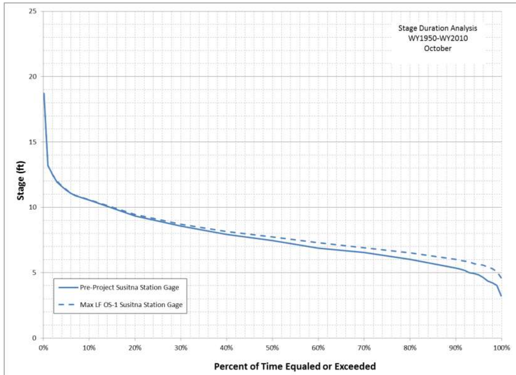
Figure J-15 - Monthly Stage Exceedance Curves for October for pre-Project and Max LF OS-1 Conditions, Susitna Station Gage
