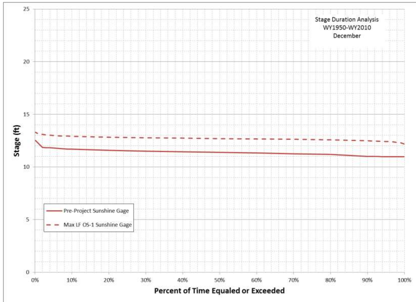
Figure J-4 - Monthly Stage Exceedance Curves for December for pre-Project and Max LF OS-1 Conditions, Sunshine Gage
