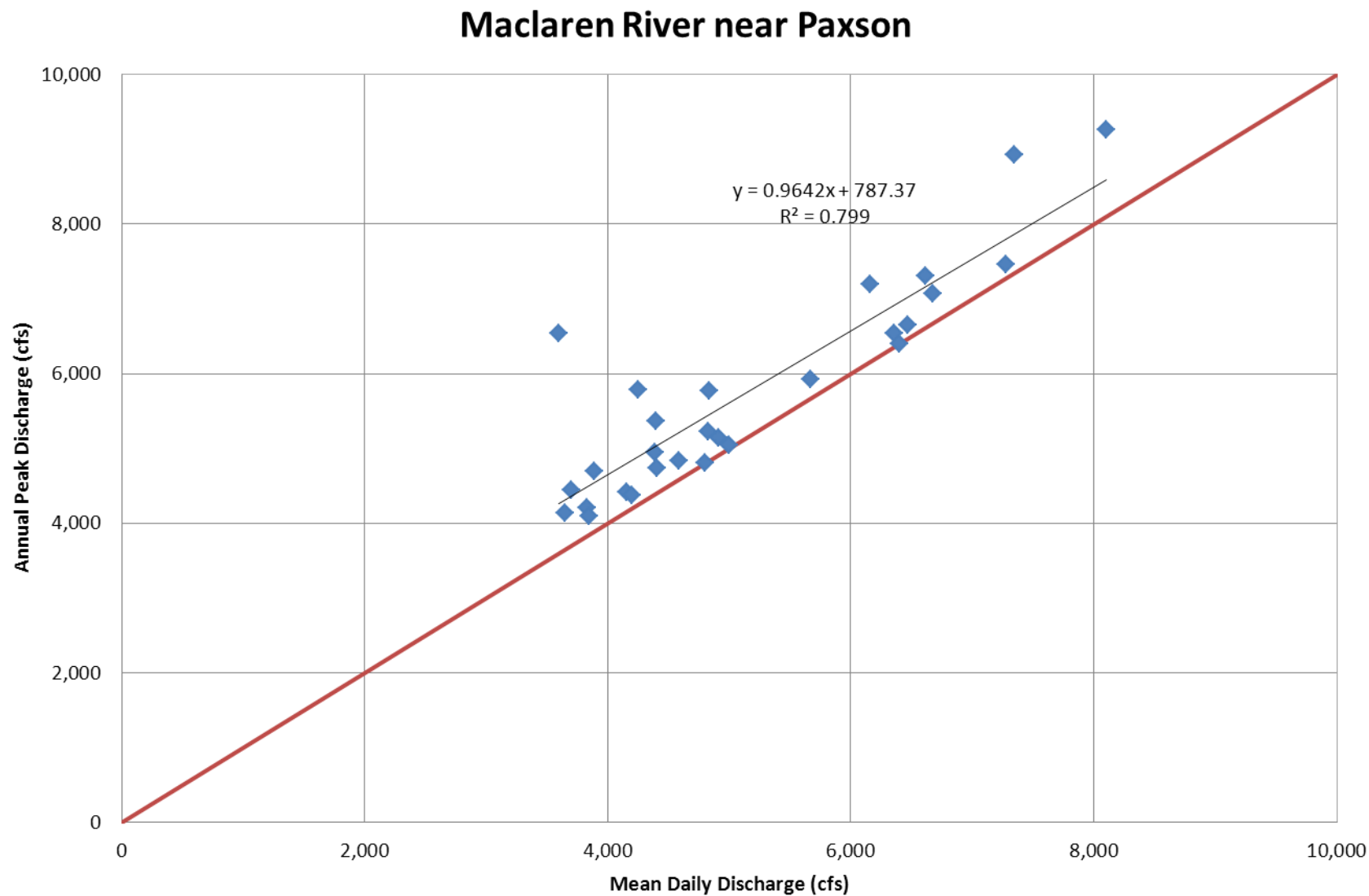
Figure D-2 – Maclaren River near Paxson regression to extend the Pre-Project USGS available record annual peak data.
