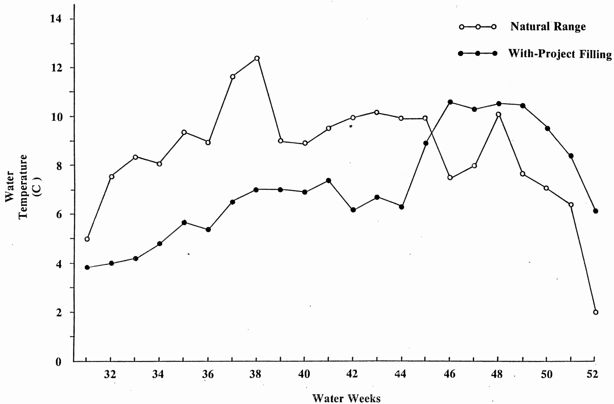
Figure 15. Simulated weekly river temperatures (C) at river mile 150 for summer 1981, natural and Watana 1992 demand filling results.
