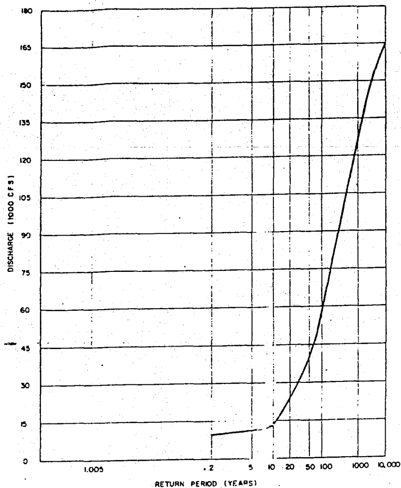
FLOOD FREQUENCY CURVE (INFLOW AFTER ROUTING THROUGH WATPNA)
