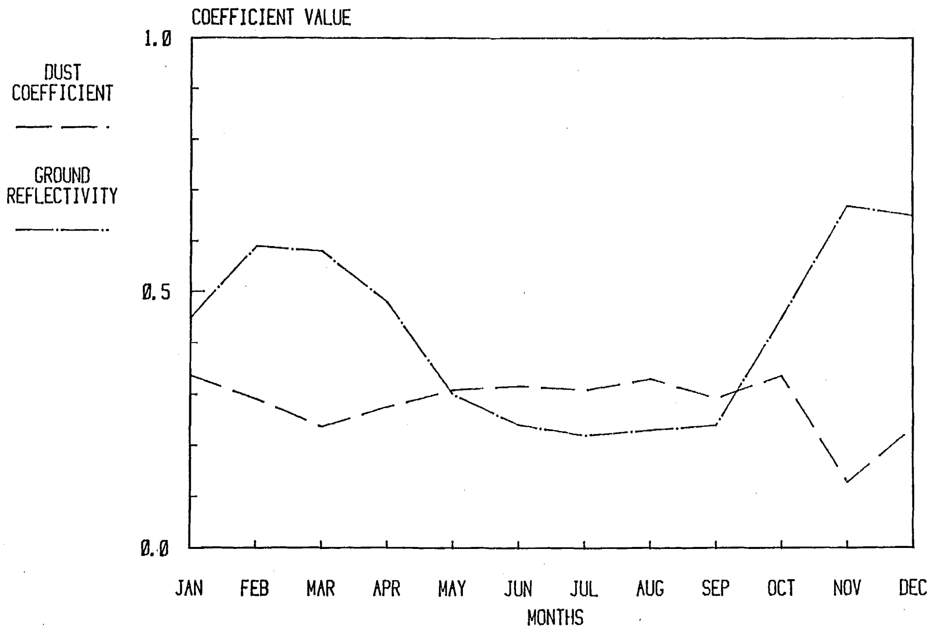
Figure 17. Ground reflectivity and atmospheric dust coefficients, Matanuska Agricultural Experiment Station, Palmer.
