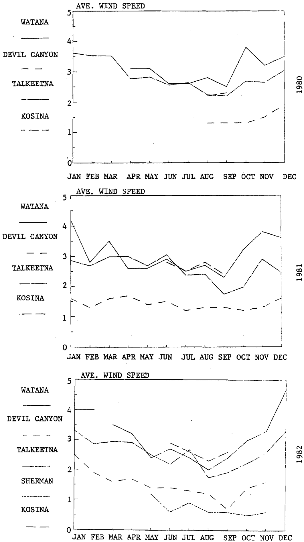
Figure 20. Average monthly wind speeds' (M/S), 1980, 1981, 1982.
