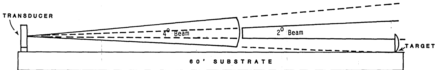
Figure 6. IMPROPERLY aimed transducer. Beamwidth switch is set to Alt. (or 4^\circ ). Scope is triggered from XM 4^\circ . Note that beam is aimed too high, although the 4^\circ beam solidly hits the target, the 2^\circ beam just barely hits the target (see figure 5 for 2^\circ scope waveform.) Fish may be missed.
