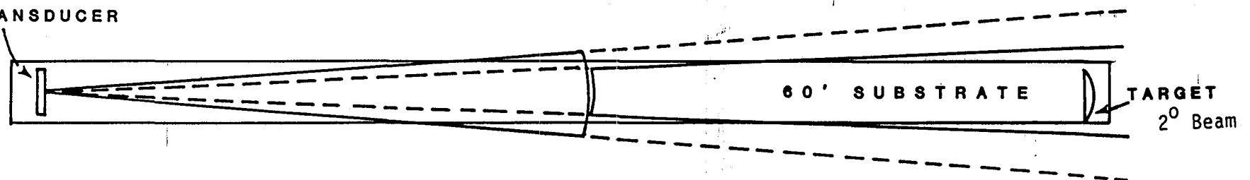
Figure 8. PROPERLY aimed transducer. Transducer beamwidth switch is set to alternate and scope is triggered from XM 4^\circ . This assumes vertical aiming of transducer is correct.
