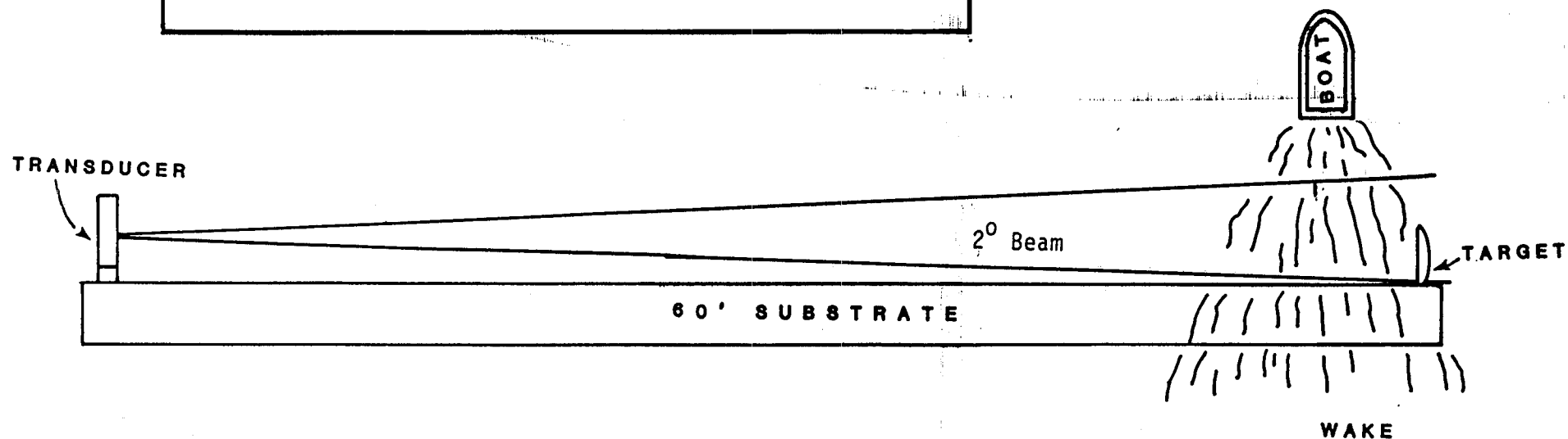
Figure 10. Properly aimed transducer but multiple echos from wake of boat. This will cause many counts, usually in outer sectors, and will probably trigger the debris indicator.
