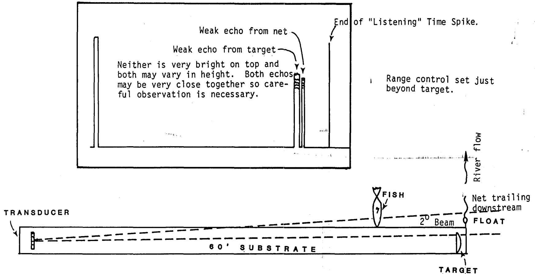
Figure 7. IMPROPERLY aimed transducer. Beamwidth switch is set to 2^\circ and scope is triggered from XM 2^\circ . Transducer is aimed too far downstream, just barely hitting target. This will cause an overcount on salmon in the last half of substrate because salmon tend to linger downstream of pipe before crossing. If salmon tend to overcount near end of substrate, this may be the problem. Reaiming the transducer more upstream will cure the problem.
