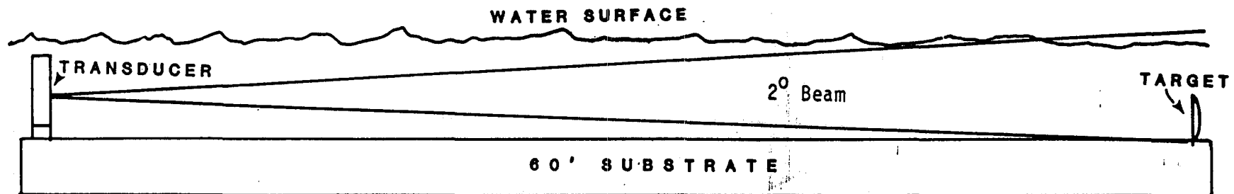
Figure 11. Improperly aimed transducer. Beamwidth switch set to 2^{\circ} and scope triggered from 2^{\circ} . Note water is too shallow even for 2^{\circ} beam which is boxed in. Counting range on side scanner would have to be reduced to about 50' to prevent surface echos from counting. Target will be obscured by surface echos.
