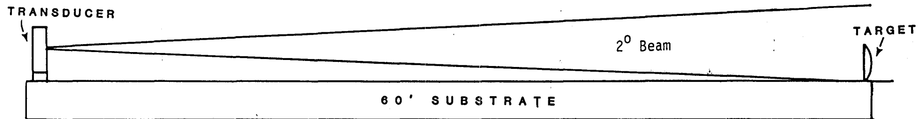
Figure 1. PROPERLY aimed transducer when beamwidth switch is set to 2° and scope triggered from XM 2°.
