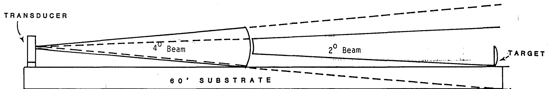
Figure 2. PROPERLY aimed transducer when beamwidth switch is set to alternate and scope is triggered from XM 4^\circ . Note 4^\circ beam is skimming surface of substrate beyond the 50% point on substrate thus causing reflections from imperfections on the substrate surface. This is okay since the 4^\circ beam will not count any echos beyond the 50% point.
