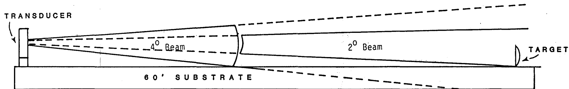
Figure 3. PROPERLY aimed transducer when beamwidth is set to alternate but scope is triggered from XM 2°.
