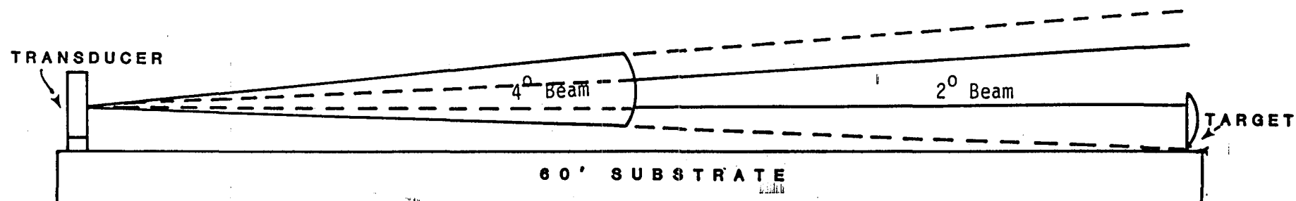
Figure 5. IMPROPERLY aimed transducer. Beamwidth switch is set to 4° and scope is triggered from XM 2°. Note that beam is aimed too high and is just catching target in 2° beam although 4° beam does hit target. See figure 6. Low passing fish may be missed.
