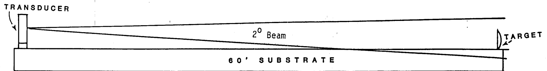
Figure 4. IMPROPERLY aimed transducer when beamwidth switch is set to 2° and scope is triggered from XM 2°. Note that beam is aimed too low, causing echos to be returned from last Y 3 of substrate imperfections even though target echo is strong and doesn't vary in height.
