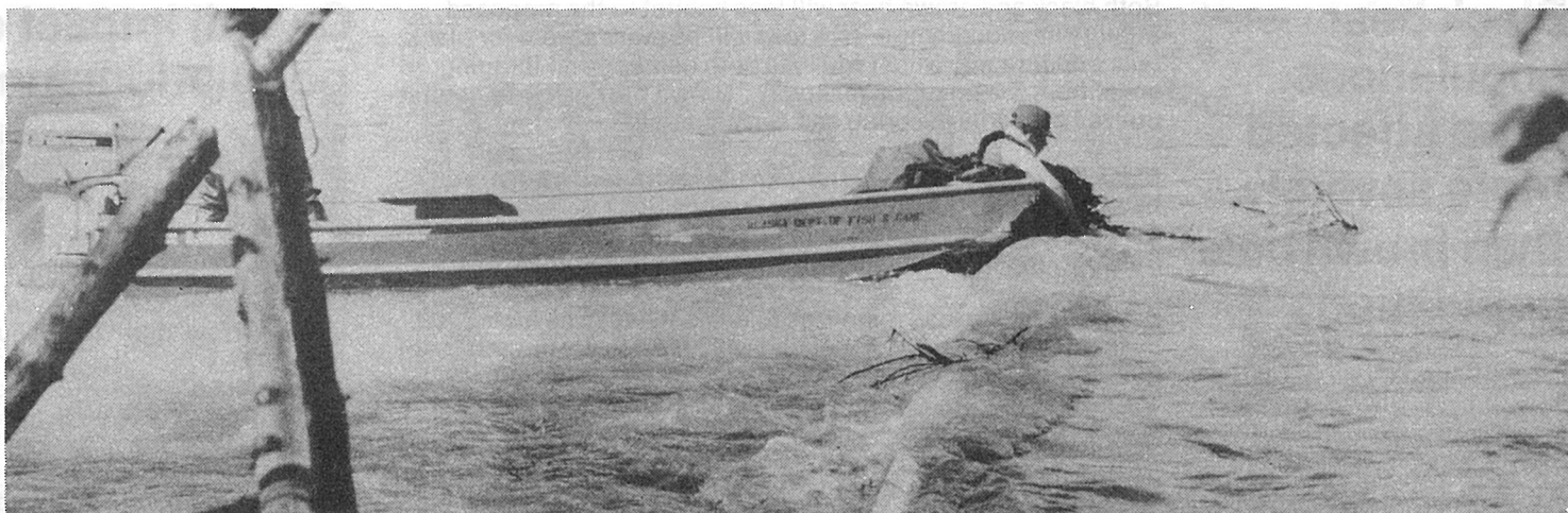
Removing debris from the aluminum tube on a sonar counter which has been raised to the surface for cleaning.
