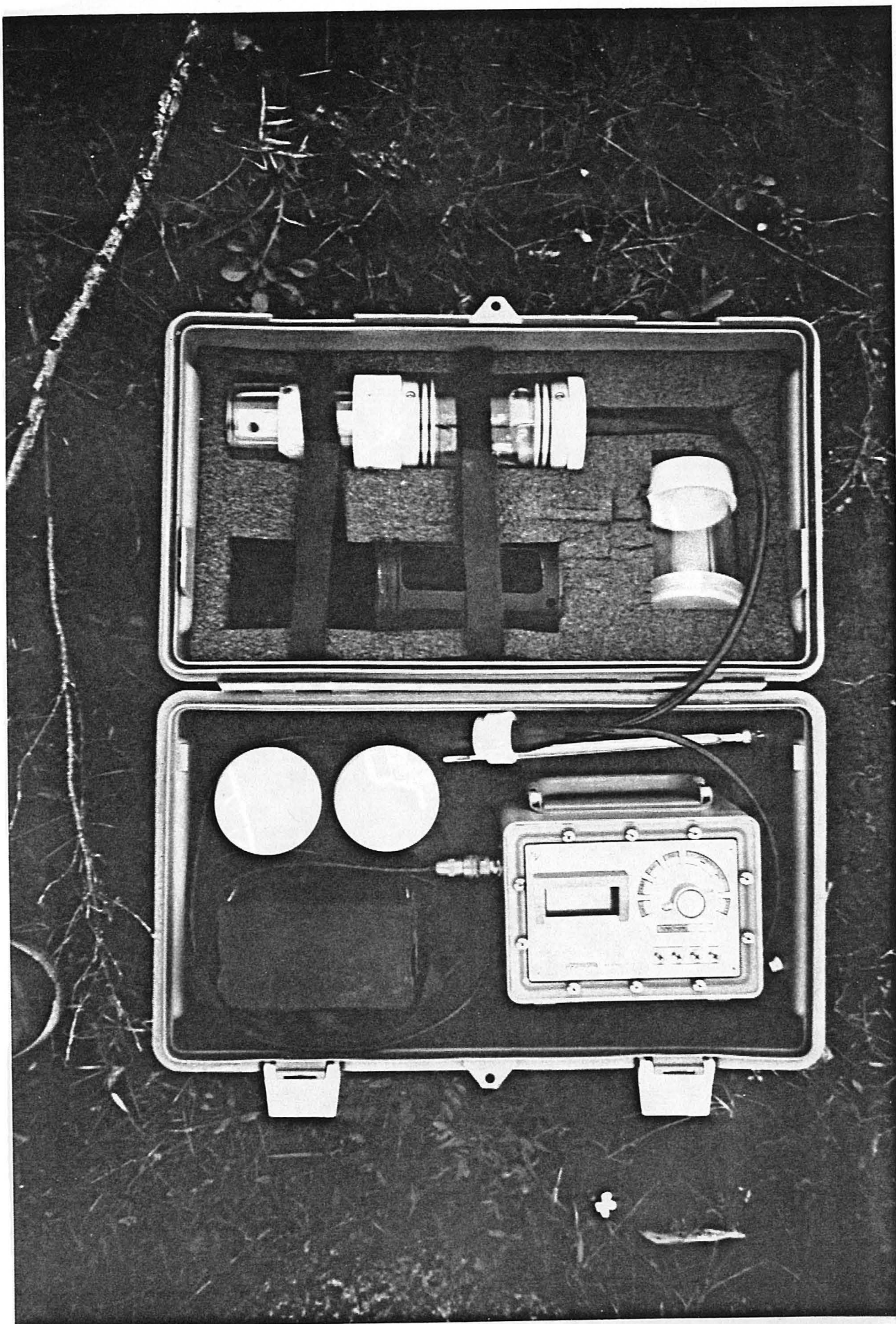
Plate 1. Hydrolab instrument used to collect water quality parameters.
