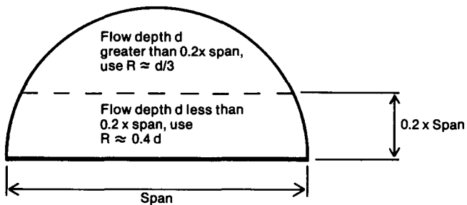
Figure H-1. Methods of estimating hydraulic radius of culverts.
