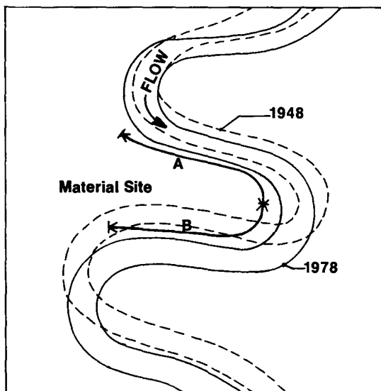
Figure A-9. Schematic of a river with a regular meander pattern and a proposed location for a material site.
