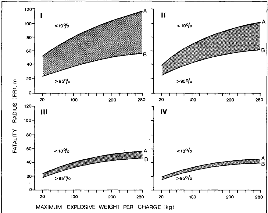
Figure G-1. Relationship of kilogram per charge to fatality radii (FR): A = 10-20% mortality, B = 95% mortality.
