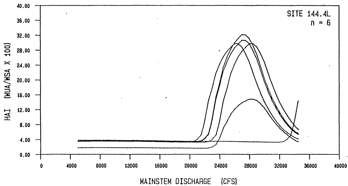
Figure 28. Response of chinook rearing habitat availability to mainstem discharge within non-modeled specific areas of the middle Susitna River which are associated with modeling site 144.4L of Representative Group II.
