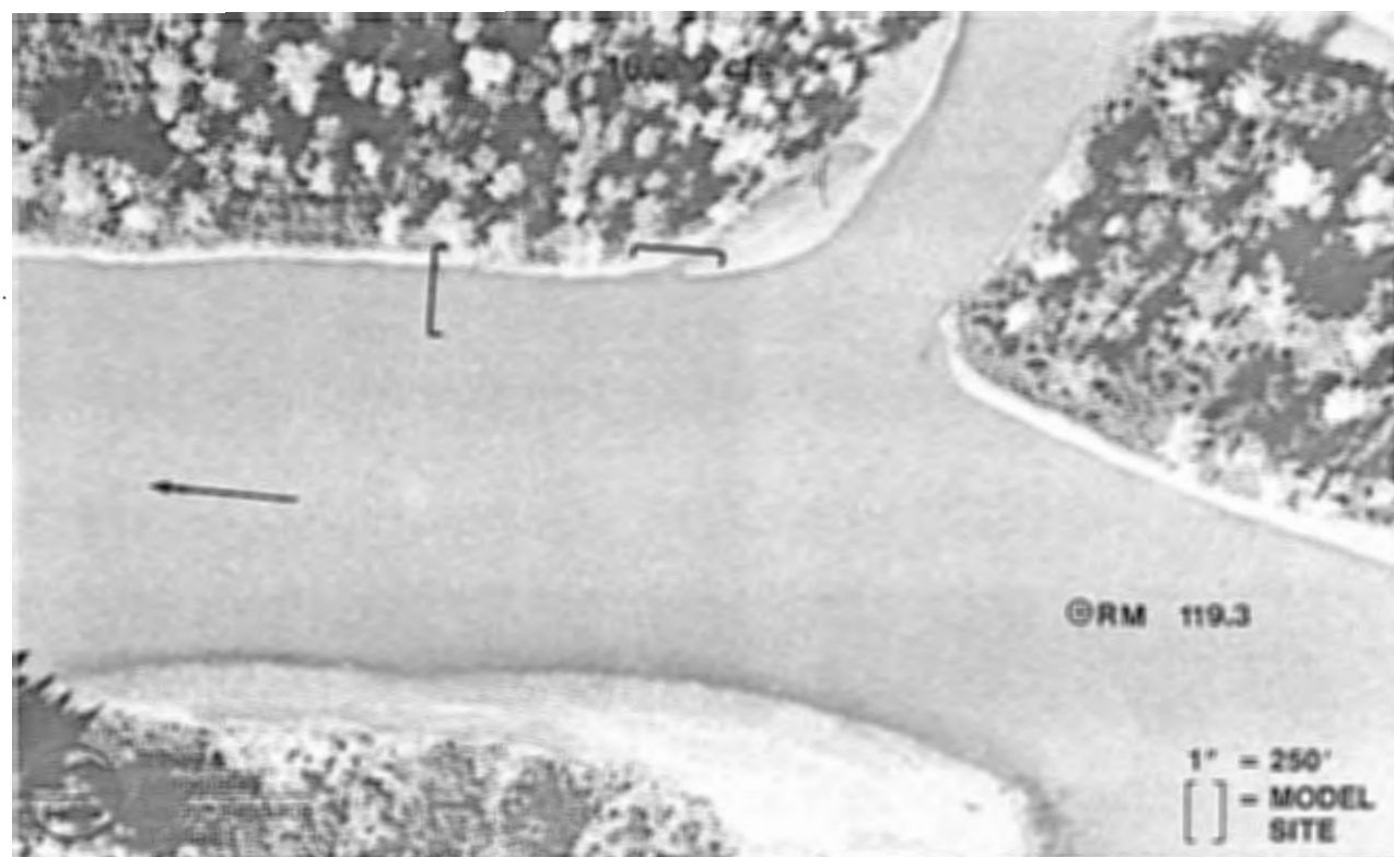
Plate A-35 Aerial photography of modeling site 119.1L at mainstem discharges of 23,000 cfs and 16,000 cfs. Site is mainstem shoal habitat and is included in Representative Group X.
