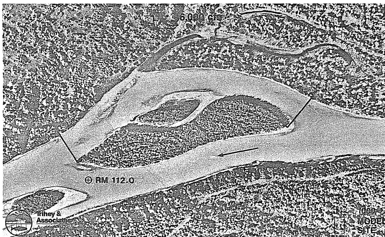
Plate A-15 Aerial photography of modeling site 112.6L at mainstem discharges of 23,000 cfs and 16,000 cfs. Site breaches at < 5,100 cfs and is included in Representative Group IV.
