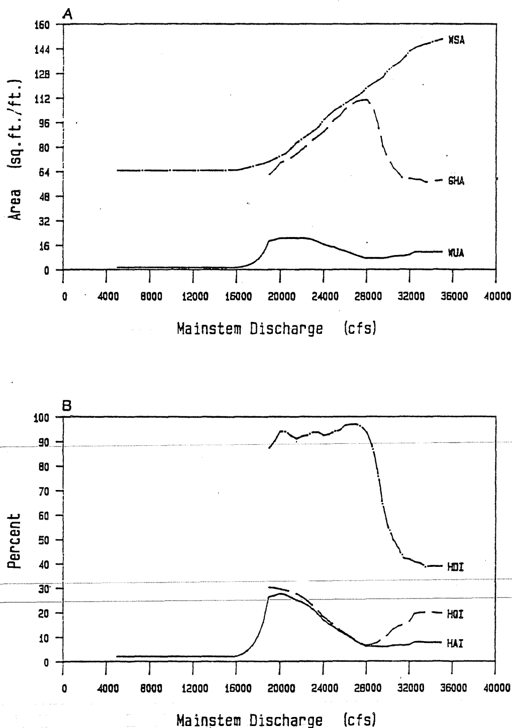
Figure 31. Surface area and chinook rearing habitat index response curves for modeling site 128.8R. A - Wetted surface area (WSA), gross habitat area (GHA) and weighted usable area (WUA). B - Habitat availability index (HAI), habitat distribution index (HDI) and habitat quality index (HQI) response functions.
