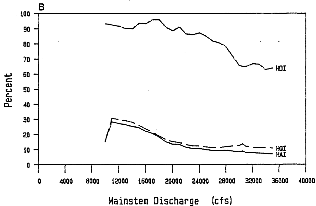
Figure 32. Surface area and chinook rearing habitat index response curves for modeling site 132.6L. A - Wetted surface area (WSA), gross habitat area (GHA) and weighted usable area (WUA). B - Habitat availability index (HAI), habitat distribution index (HDI) and habitat quality index (HQI) response functions.
