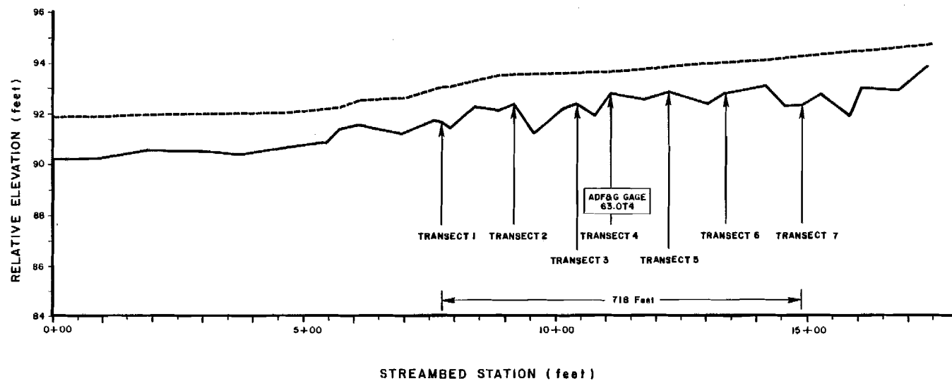
Attachment Figure C-8. Thalweg profile of the study site at Caswell Creek.
