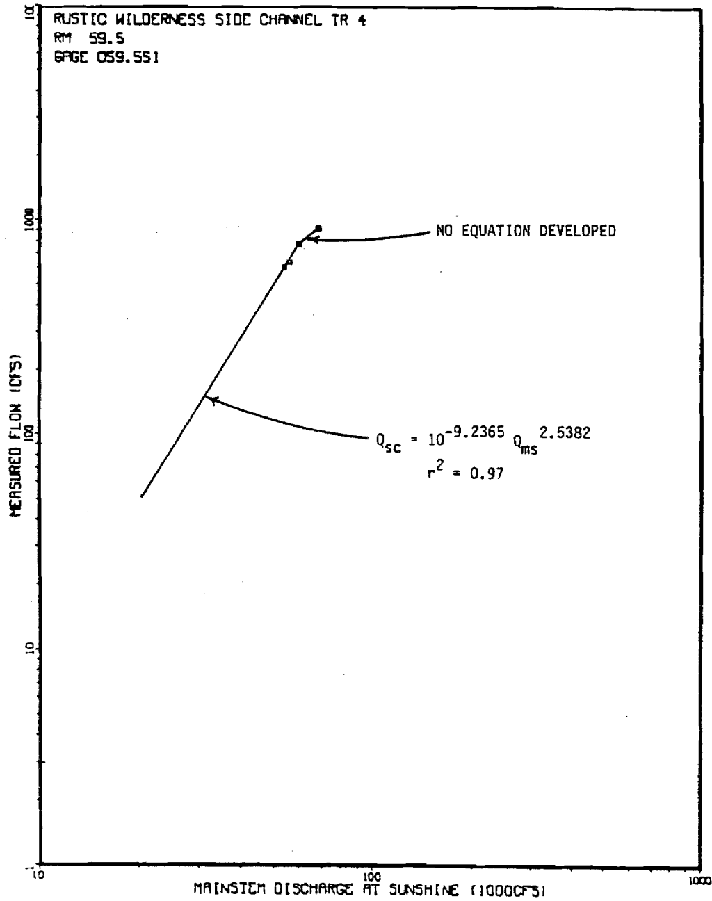
Figure 26. Rustic Wilderness Side Channel streamflow versus mainstem discharge at Sunshine Station (USGS 15292780) rating curve at transect 4 Q Site.
