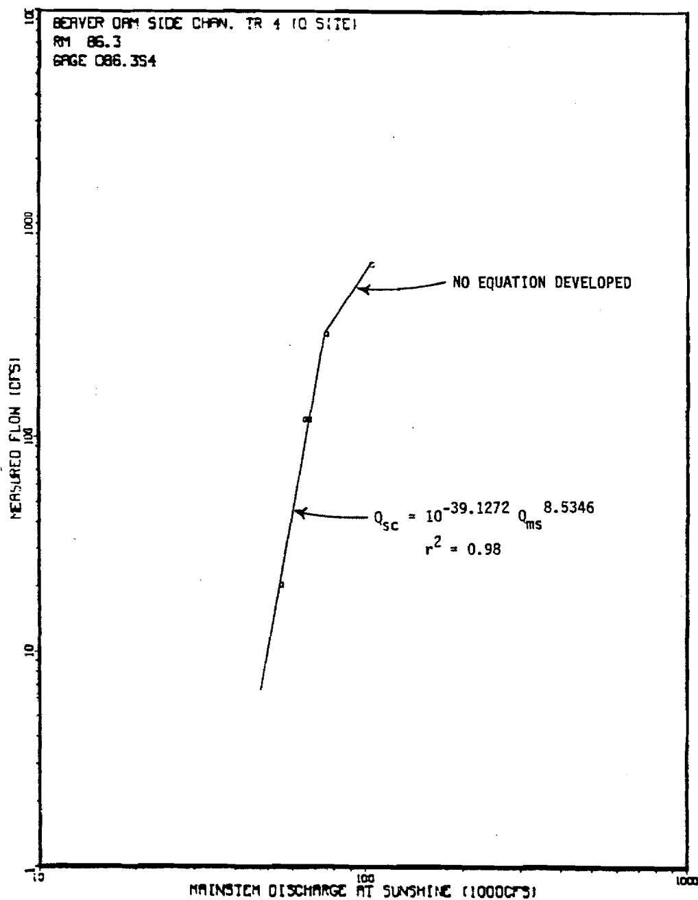
Figure 67. Beaver Dam Side Channel streamflow versus mainstem discharge at Sunshine Station (USGS 15292780) rating curve at transect 4 Q Site.
