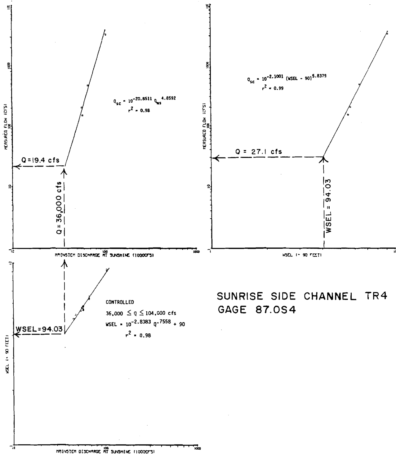
Figure 77. Comparison of rating curves for Sunrise Side Channel transect 4 Q Site.
