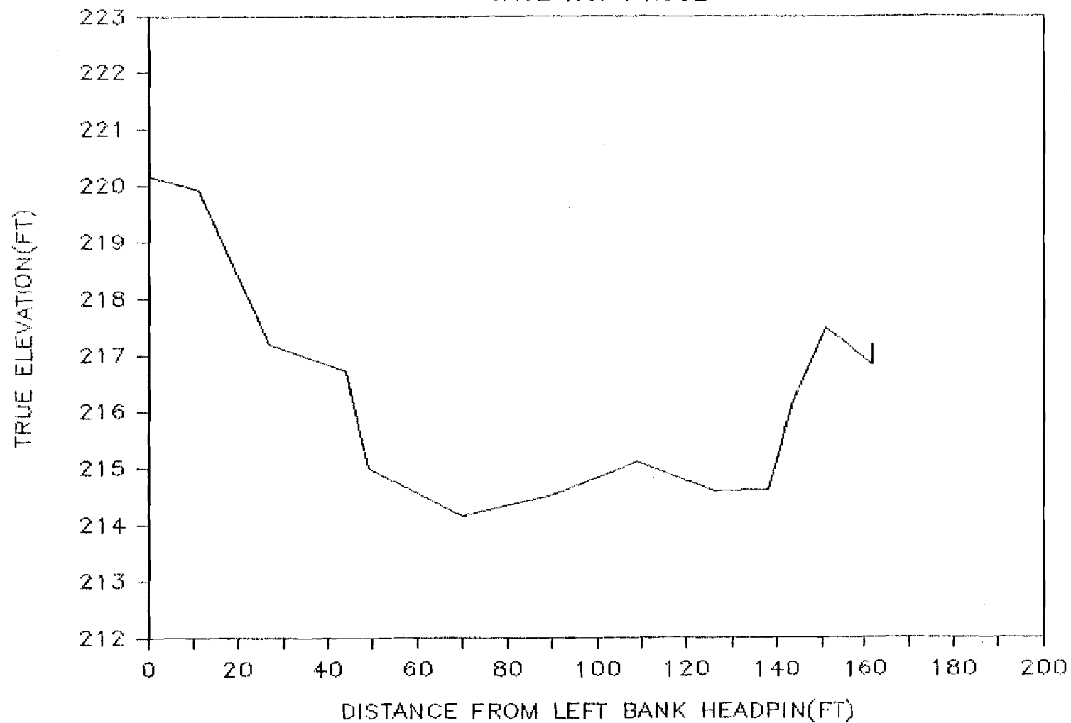
Attachment Figure D-24. Cross sectional profile obtained at transect 2 of Goose 2 Side Channel.
