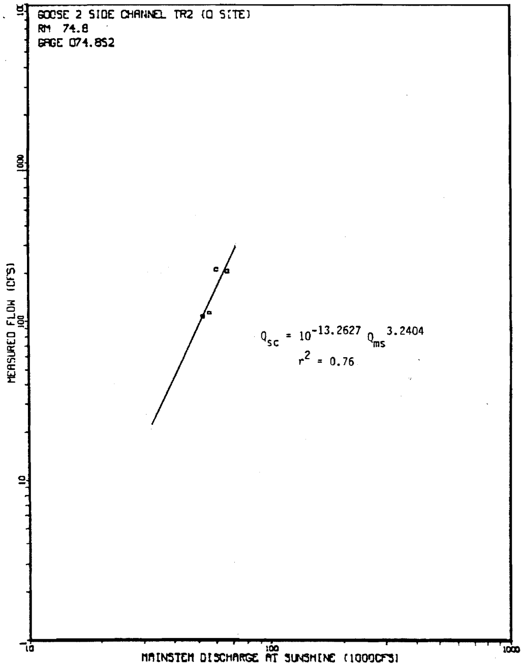
Figure 43. Goose 2 Side Channel streamflow versus mainstem discharge at Sunshine Station (USGS 15292780) rating curve at transect 2 Q Site.
