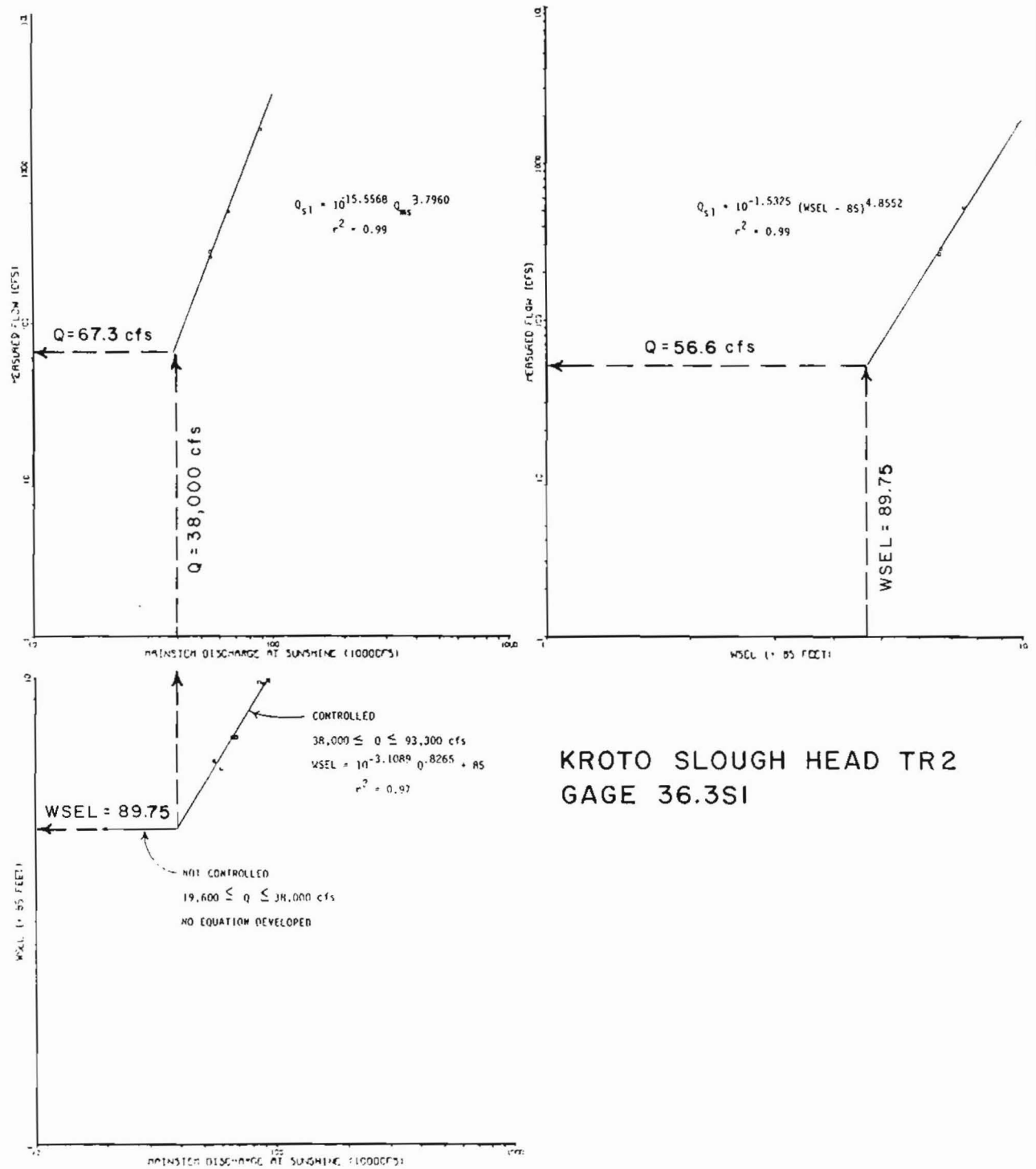
Figure 12. Comparison of rating curves for Kroto Slough Head at transect 2 Q Site.
