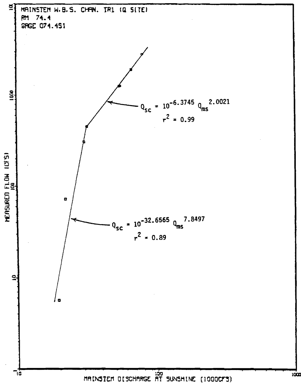
Figure 38. Mainstem West Bank Side Channel streamflow versus mainstem discharge at Sunshine Station (USGS 15292780) rating curve at transect 1 Q Site.
