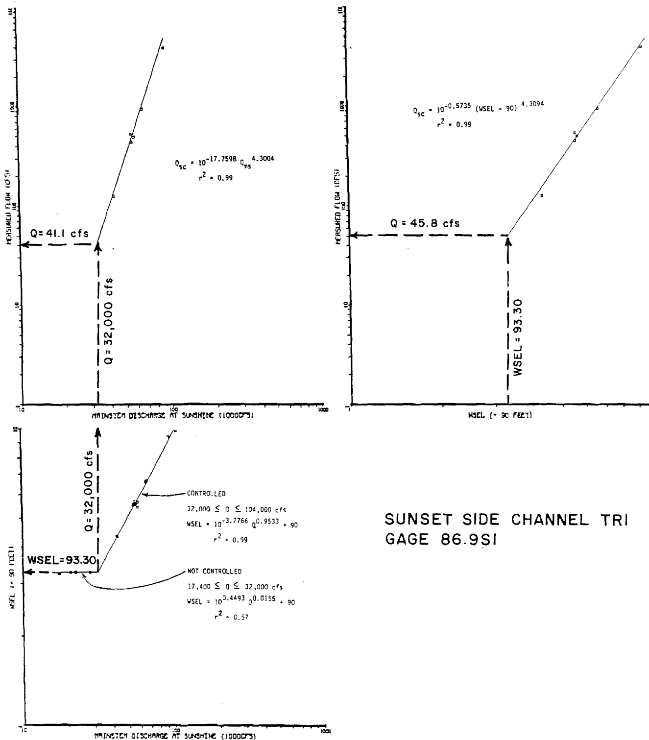
Figure 73. Comparison of rating curves for Sunset Side Channel transect 1 Q Site.
