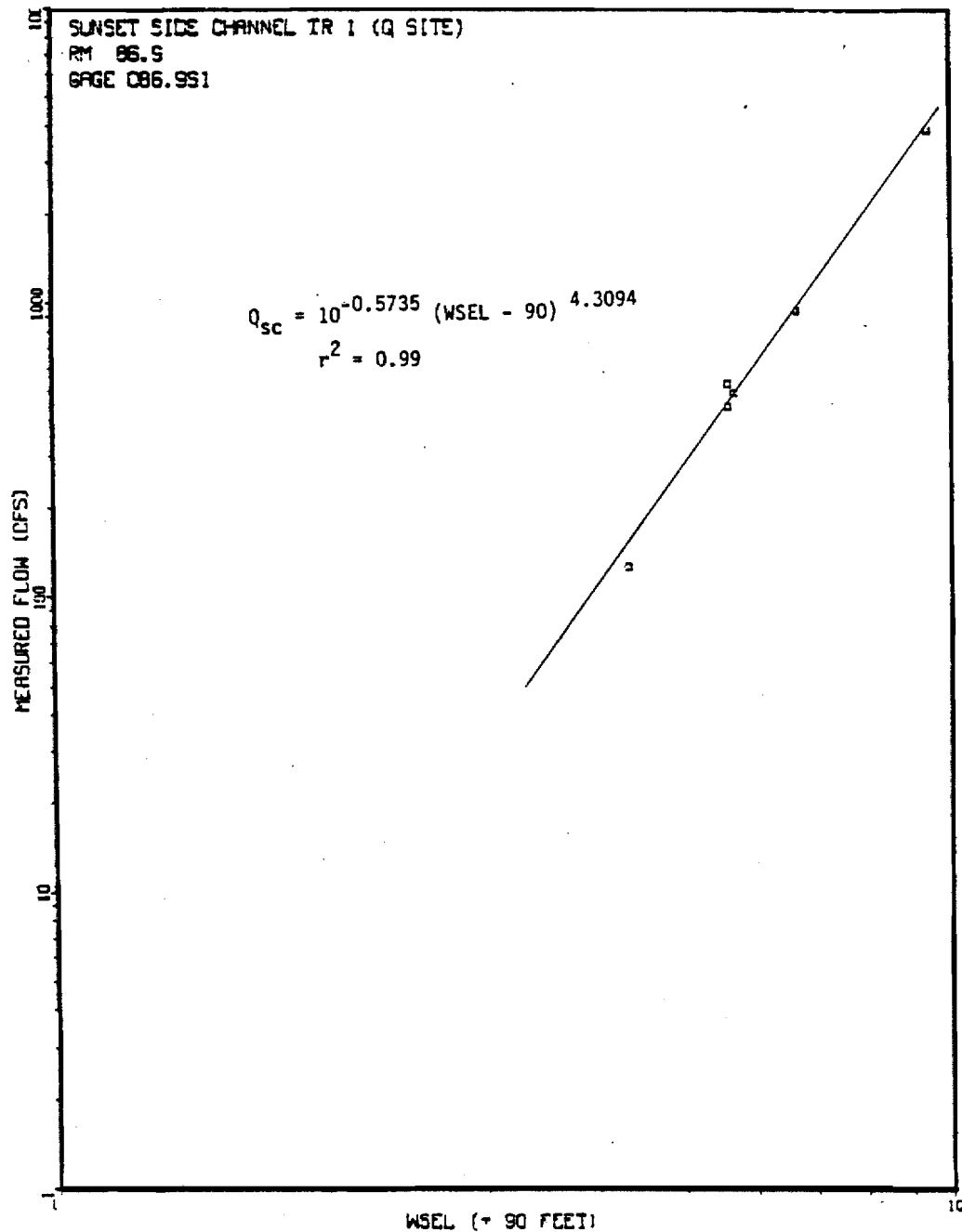
Figure 71. Sunset Side Channel streamflow versus WSEL rating curve at transect 1 Q Site.
