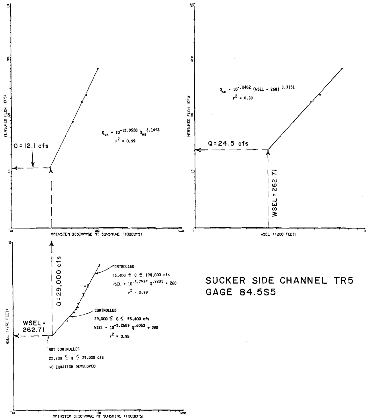
Figure 63. Comparison of rating curves for Sucker Side Channel transect 5 Q Site.
