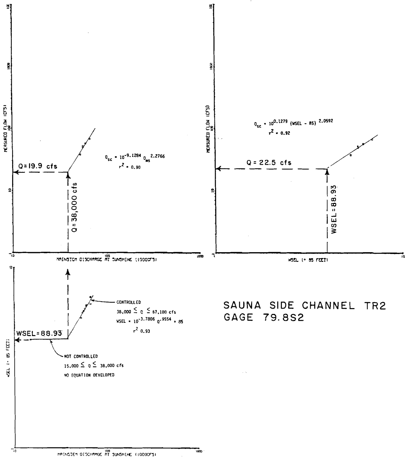
Figure 55. Comparison of rating curves for Sauna Side Channel transect 2 Q Site.
