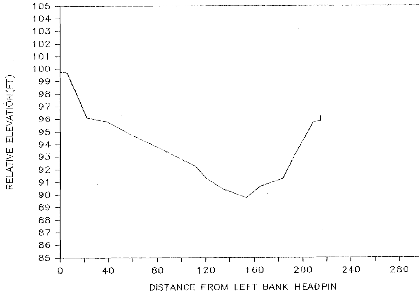
Attachment Figure D-2. Cross sectional profile obtained at transect 2 of Eagle's Nest Side Channel.
