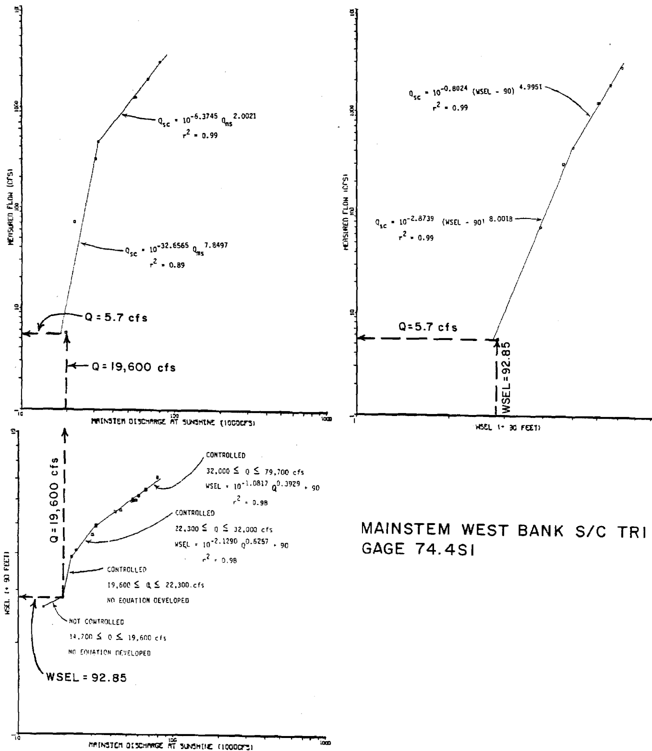
Figure 39. Comparison of rating curves for Mainstem West Bank Side Channel transect 1 Q Site.
