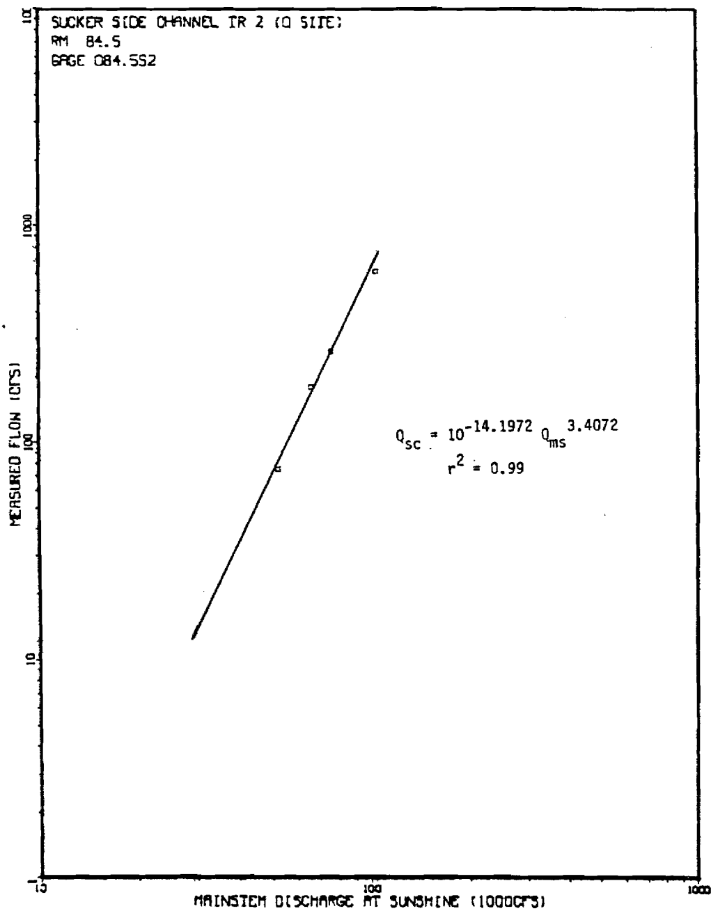
Figure 60. Sucker Side Channel streamflow versus mainstem discharge at Sunshine Station (USGS 15292780) rating curve at transect 2 Q Site.
