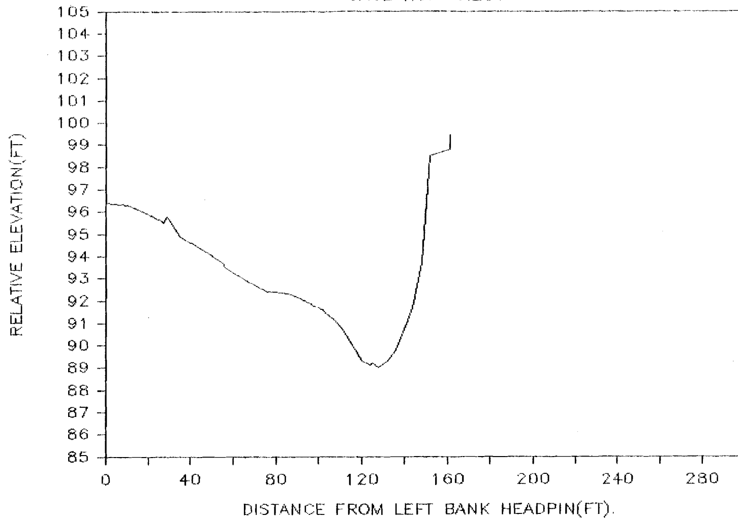
Attachment Figure D- 16. Cross sectional profile obtained at transect 6 of Island Side Channel.
