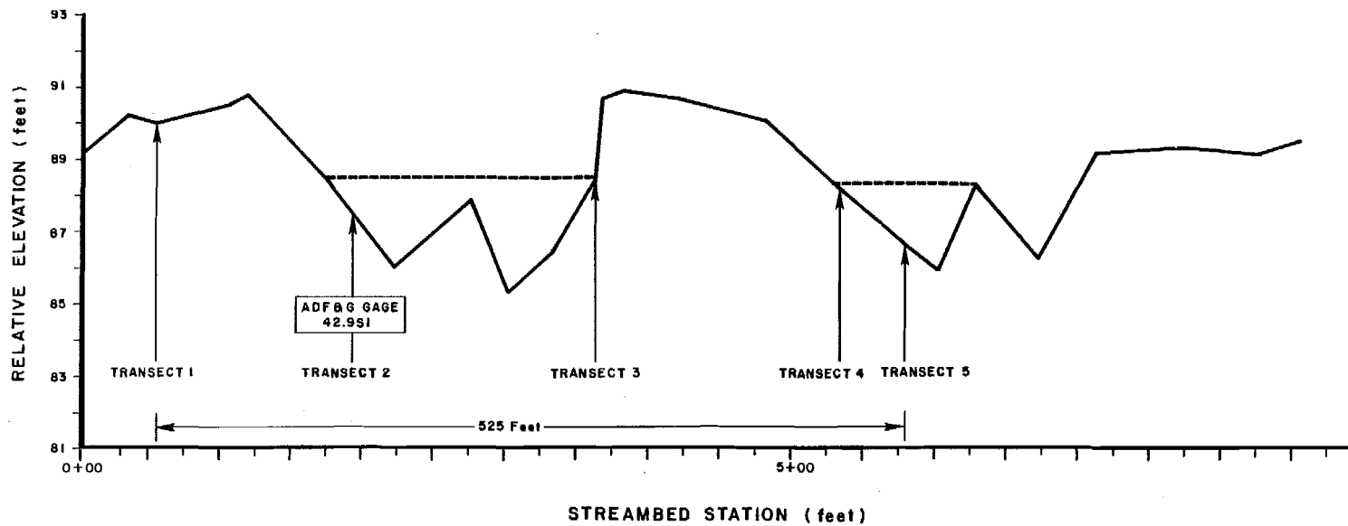
Attachment Figure C- 5. Thalweg profile of the study site at Bear Bait Side Channel.
