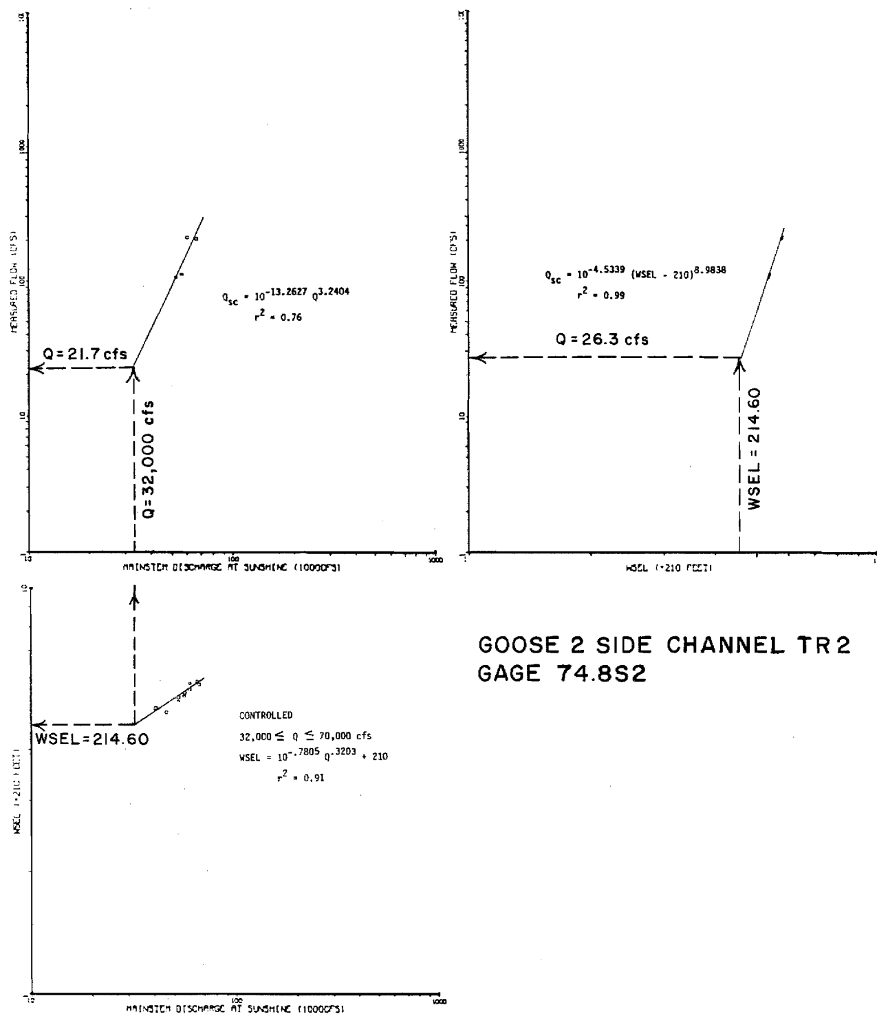
Figure 44. Comparison of rating curves for Goose 2 Side Channel transect 2 Q Site.
