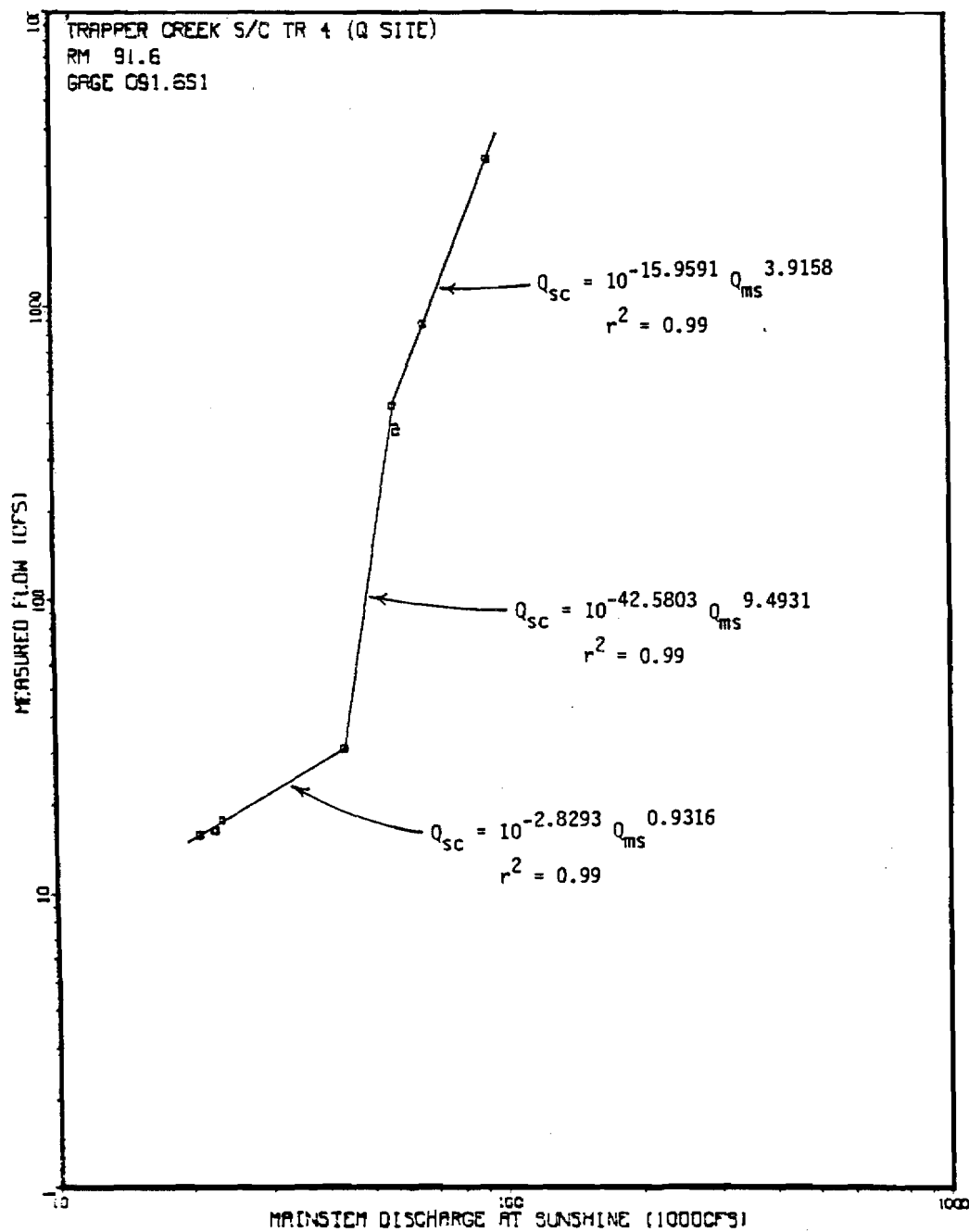
Figure 84. Trapper Creek Side Channel streamflow versus mainstem discharge at Sunshine Station (USGS 15292780) rating curve at transect 4 Q Site.
