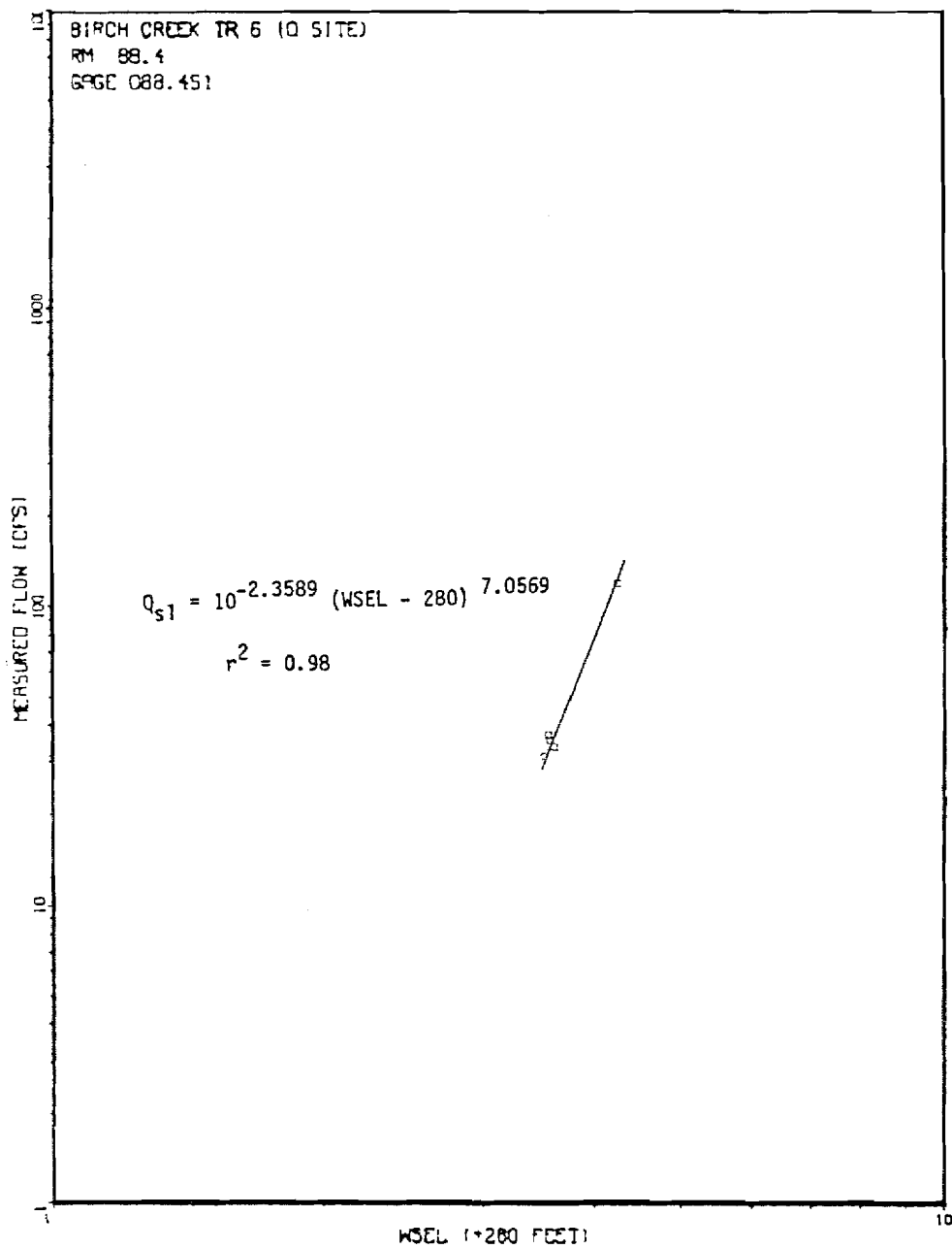
Figure 80 Birch Creek Slough streamflow versus WSEL rating curve at transect 6 Q Site.
