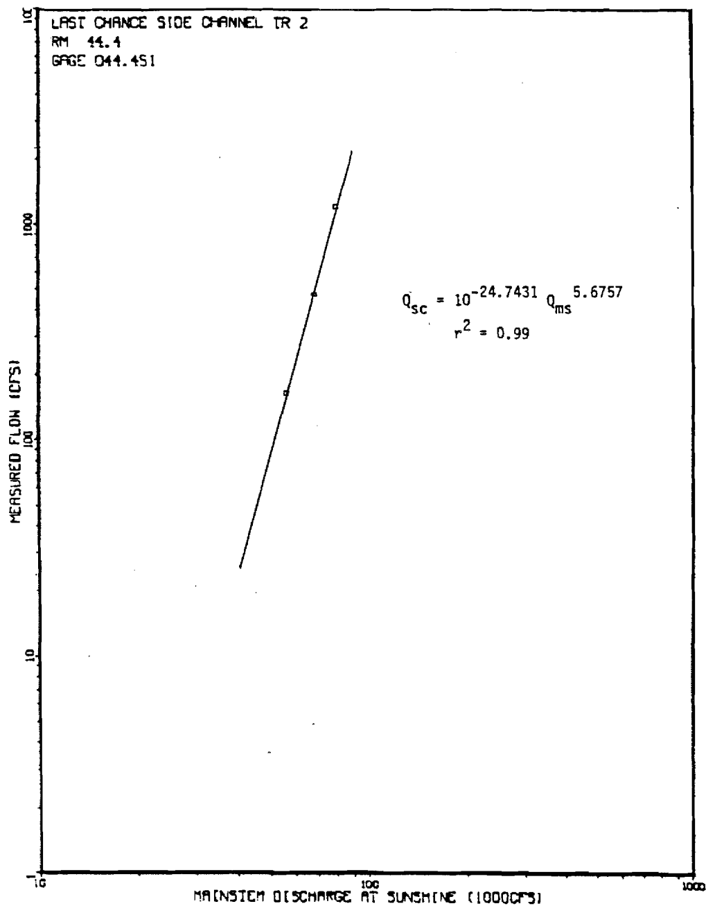
Figure 22. Last Chance Side Channel streamflow versus mainstem discharge at Sunshine Station (USGS 15292780) rating curve at transect 2 Q Site.
