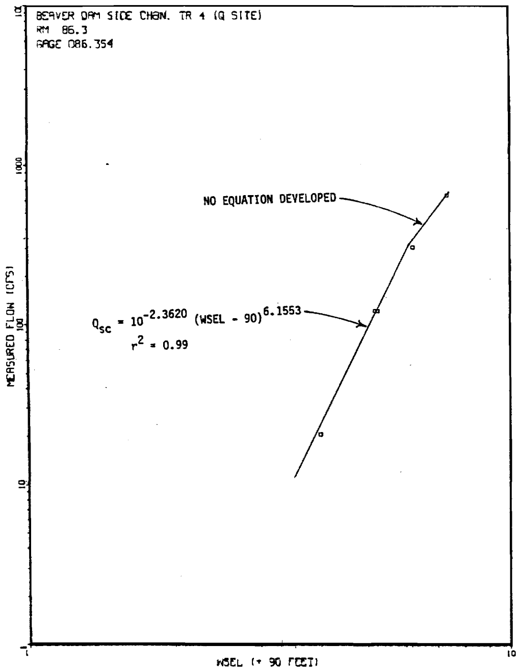
Figure 66. Beaver Dam Side Channel streamflow versus WSEL rating curve at transect 4 Q Site.
