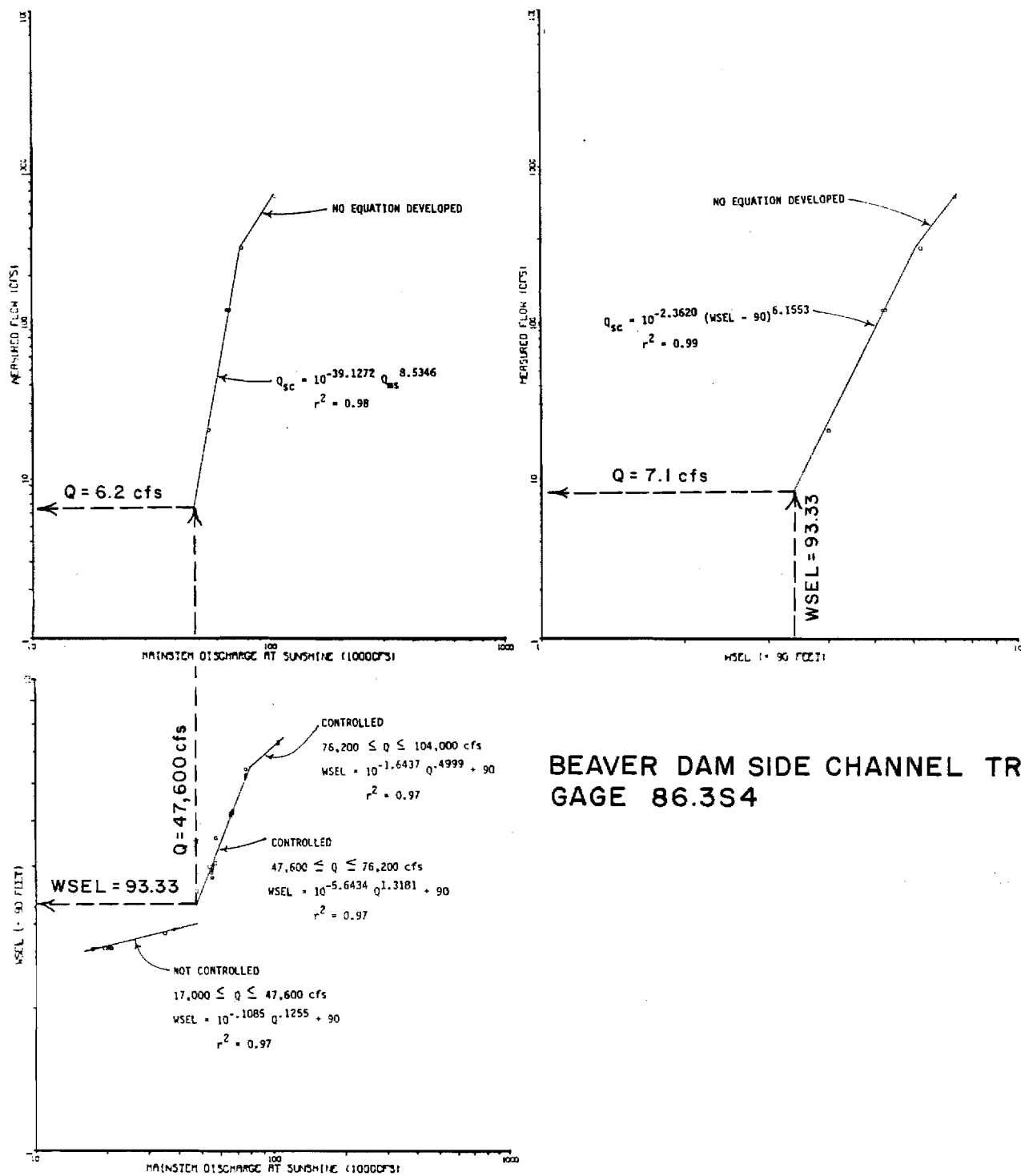
Figure 68. Comparison of rating curves for Beaver Dam Side Channel transect 4 Q Site.
