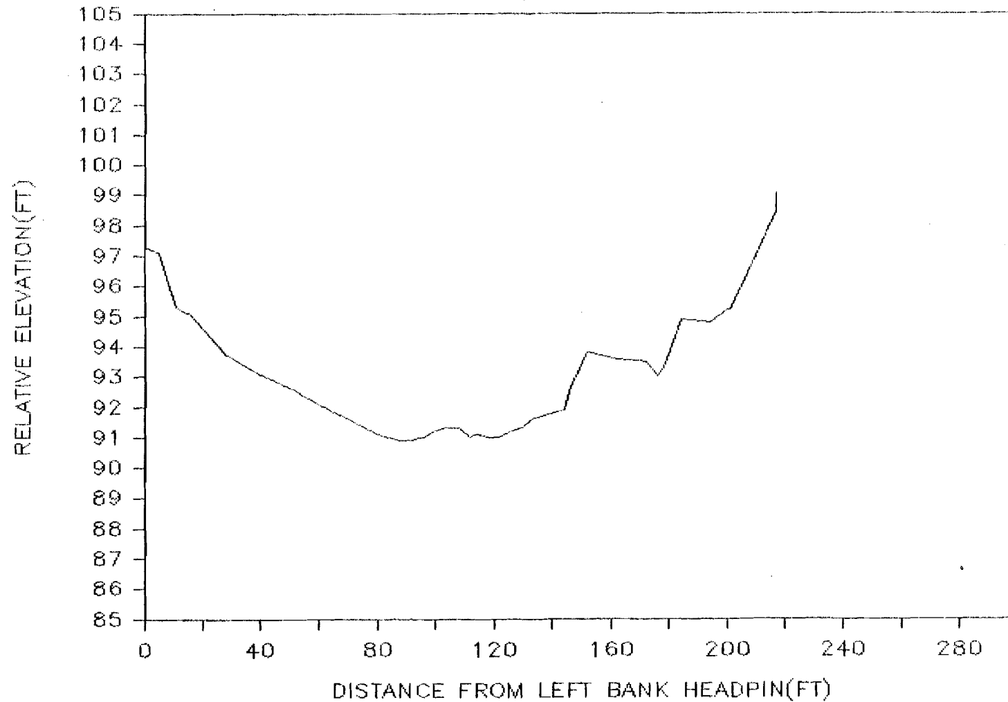
Attachment Figure D- 14. Cross sectional profile obtained at transect 4A of Island Side Channel.
