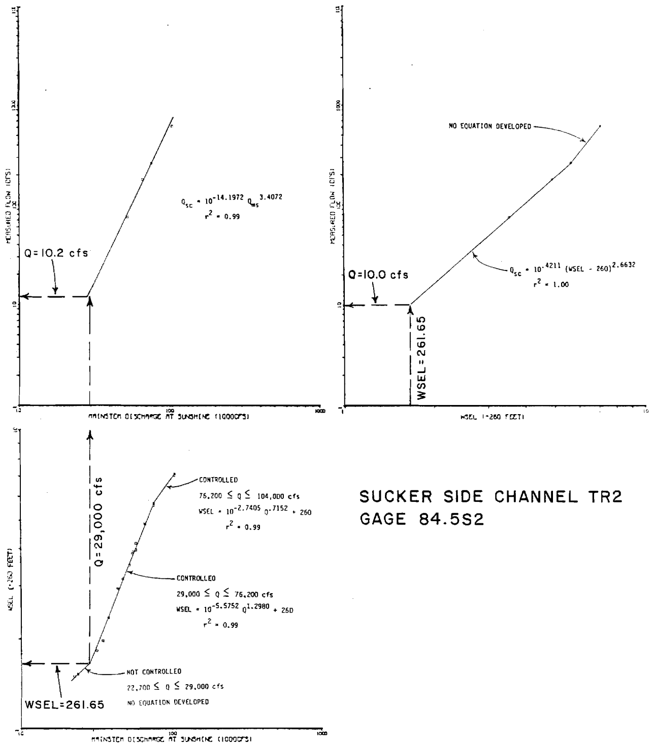
Figure 62. Comparison of rating curves for Sucker Side Channel transect 2 Q Site.
