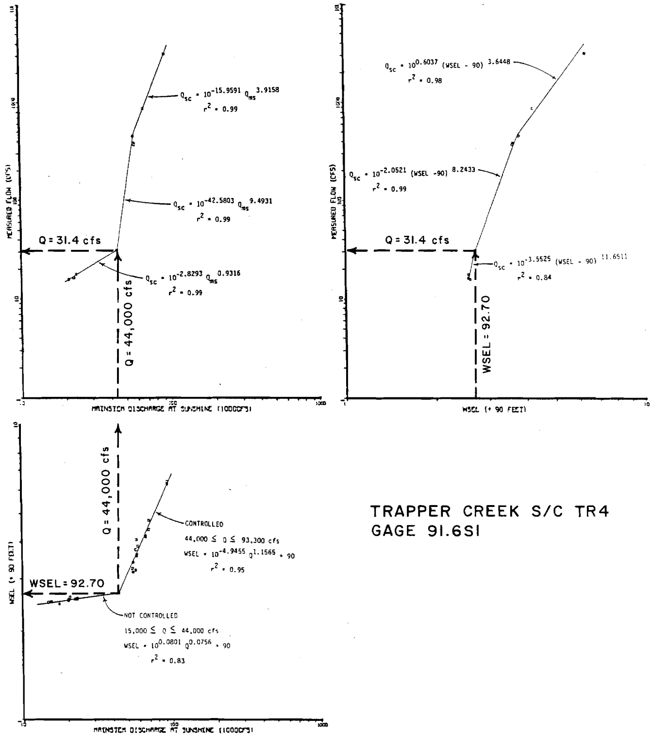
Figure 85. Comparison of rating curves for Trapper Creek Side Channel Transect 4 Q Site.
