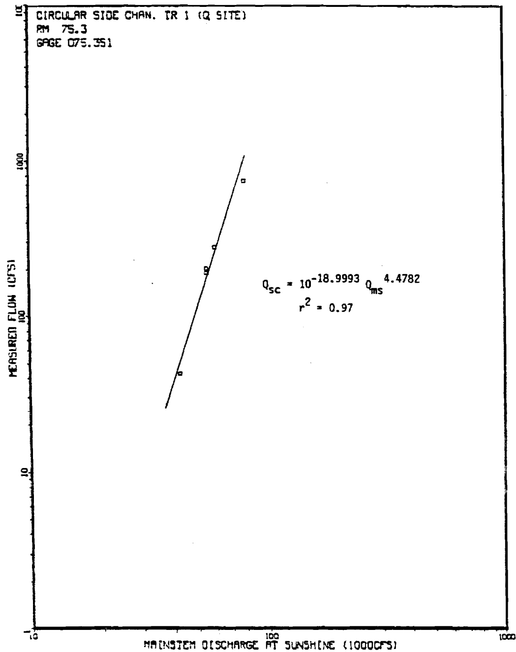
Figure 48. Circular Side Channel streamflow versus mainstem discharge at Sunshine Station (USGS 15292780) rating curve at transect 1 Q Site.
