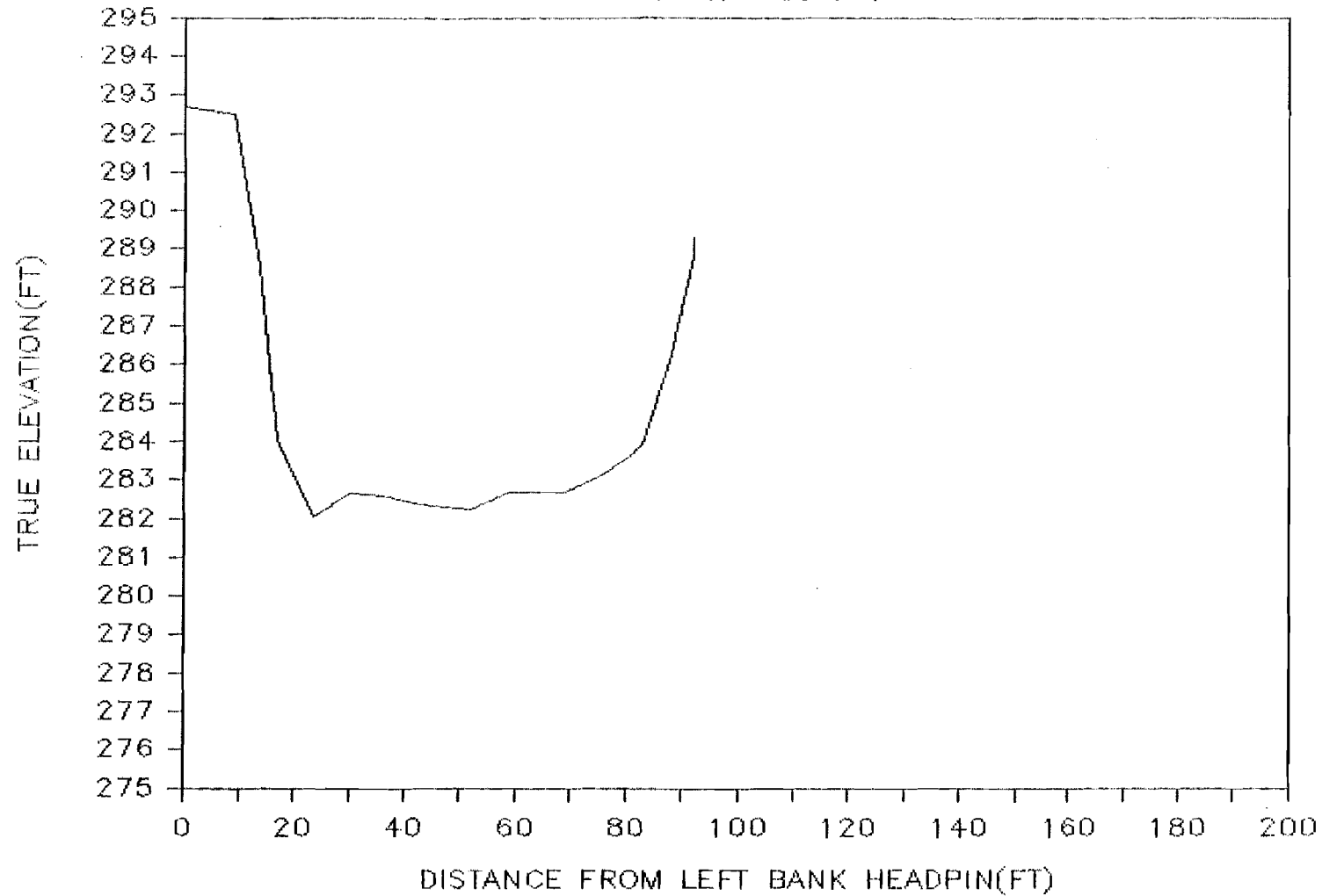
Attachment Figure D-48. Cross sectional profile obtained at transect 6 of Birch Creek Slough.
