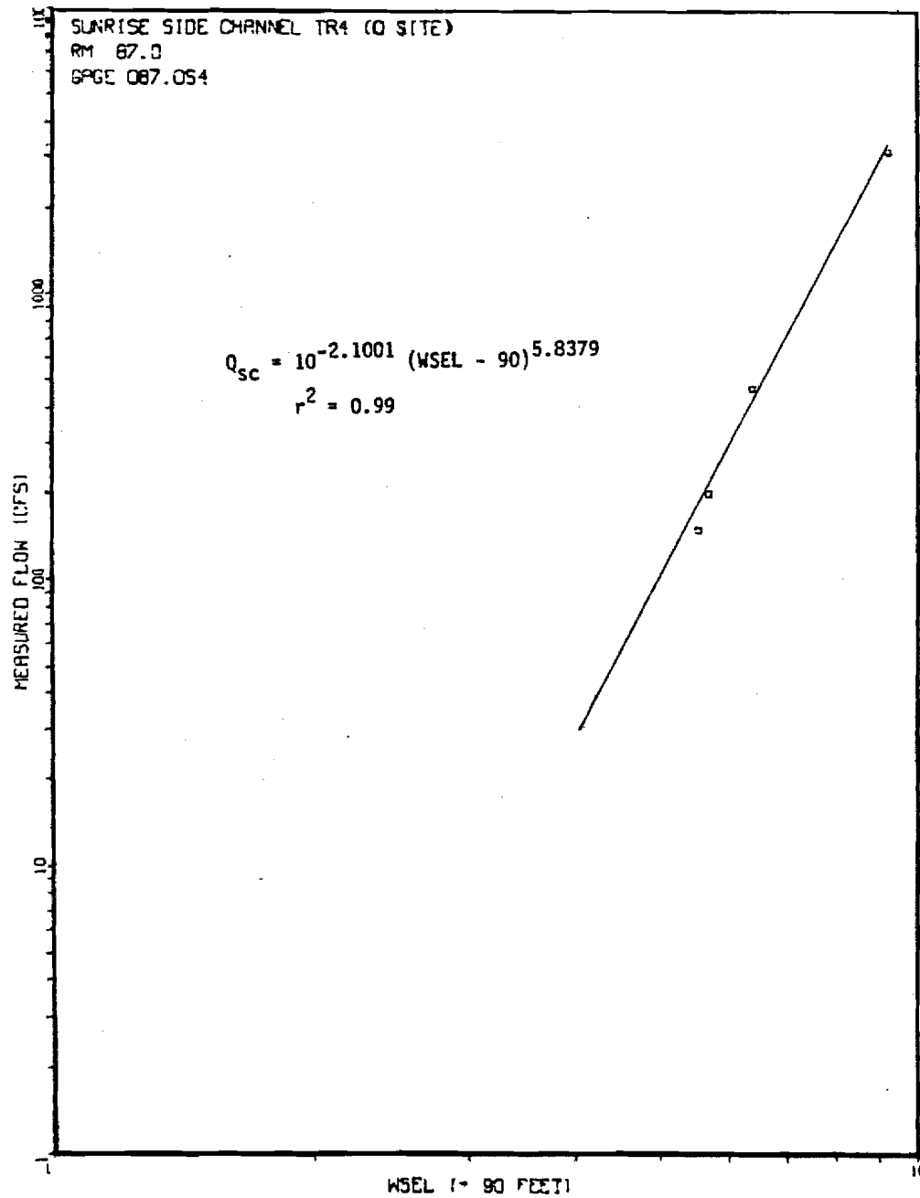
Figure 75. Sunrise Side Channel streamflow versus WSEL rating curve at transect 4 O Site.
