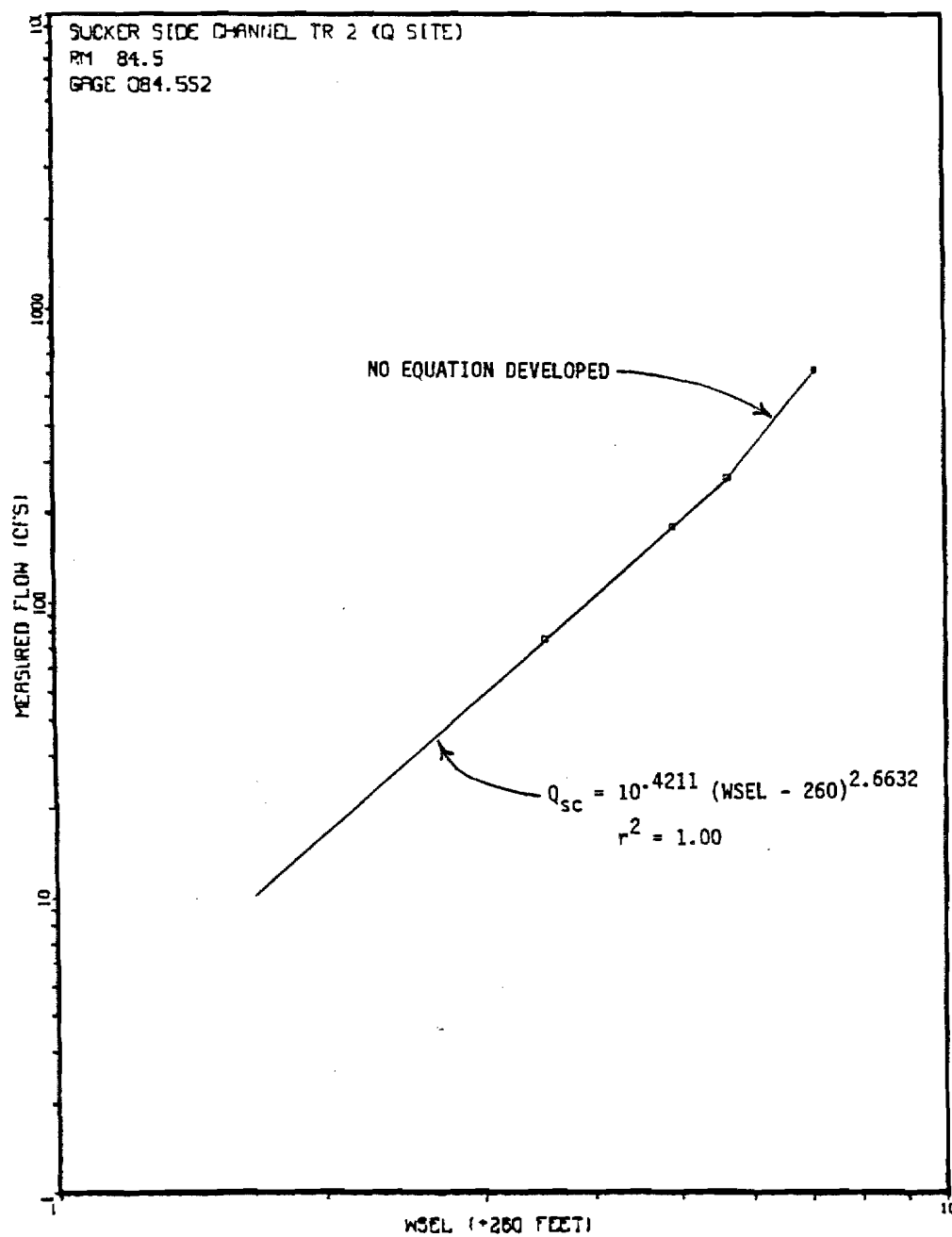
Figure 58. Sucker Side Channel streamflow versus WSEL rating curve at transect 2 Q Site.
