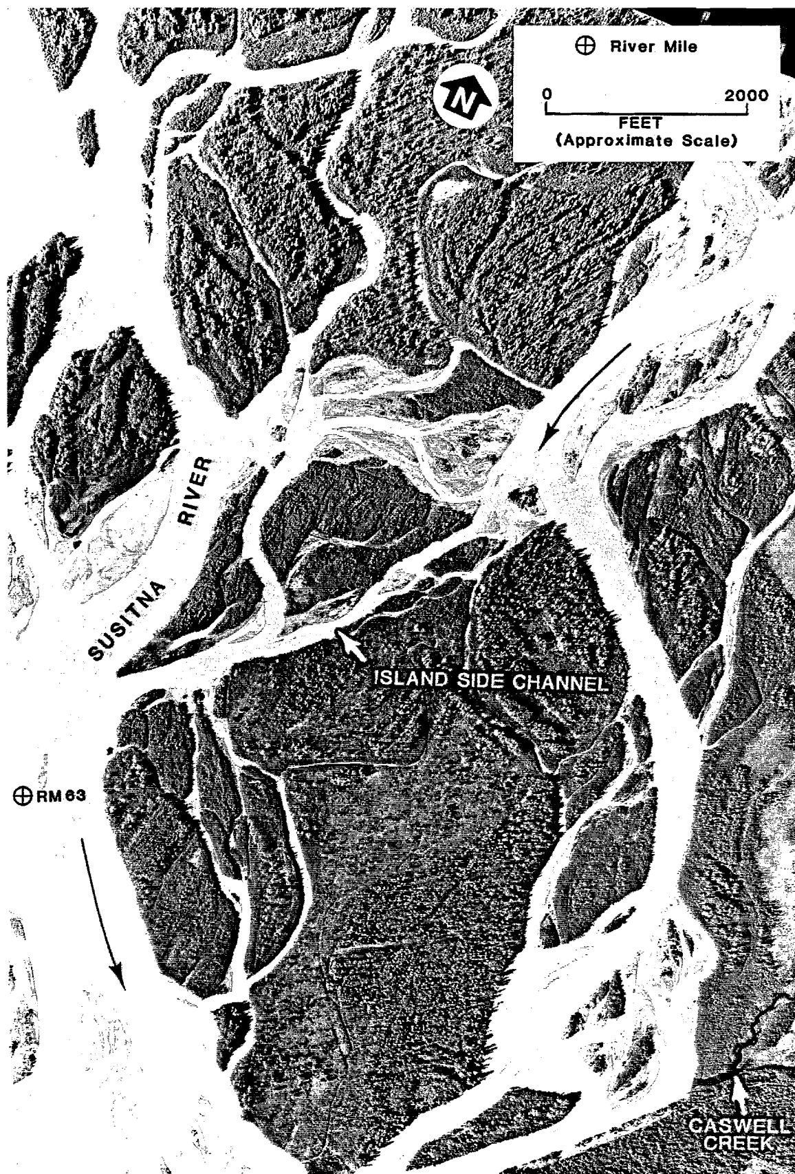
Figure 27. Overview of Caswell Creek (RM 63.0) and Island Side Channel (RM 63.2).
