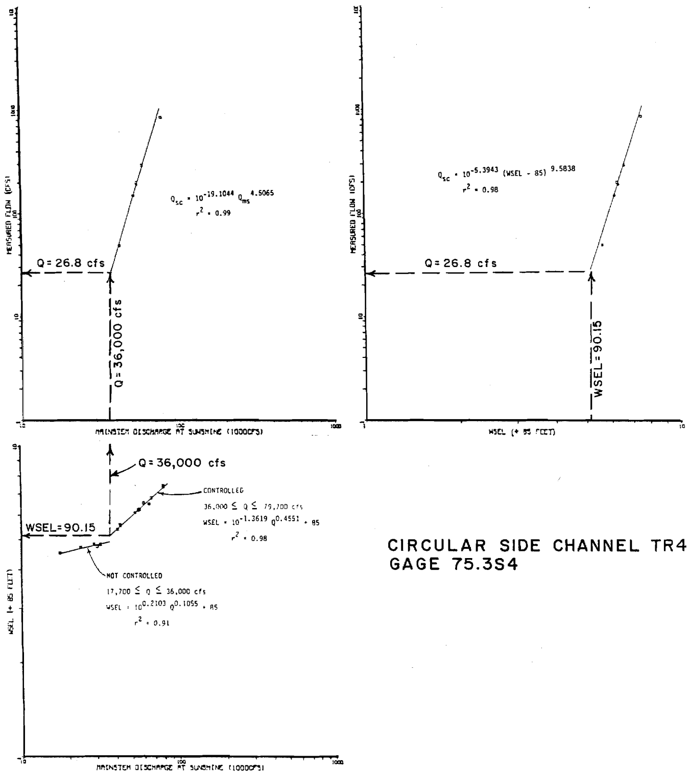
Figure 50. Comparison of rating curves for Circular Side Channel at transect 4 Q Site.
