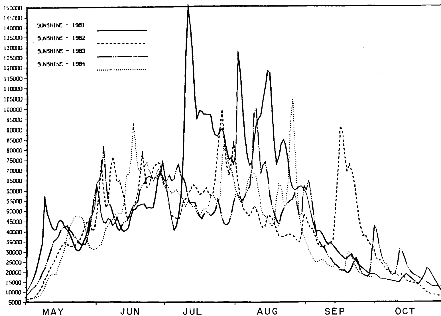
Figure 86. Susitna River hydrograph for May-October 1981, 1982, 1983 and 1984 at Sunshine Station (USGS 15292780).
