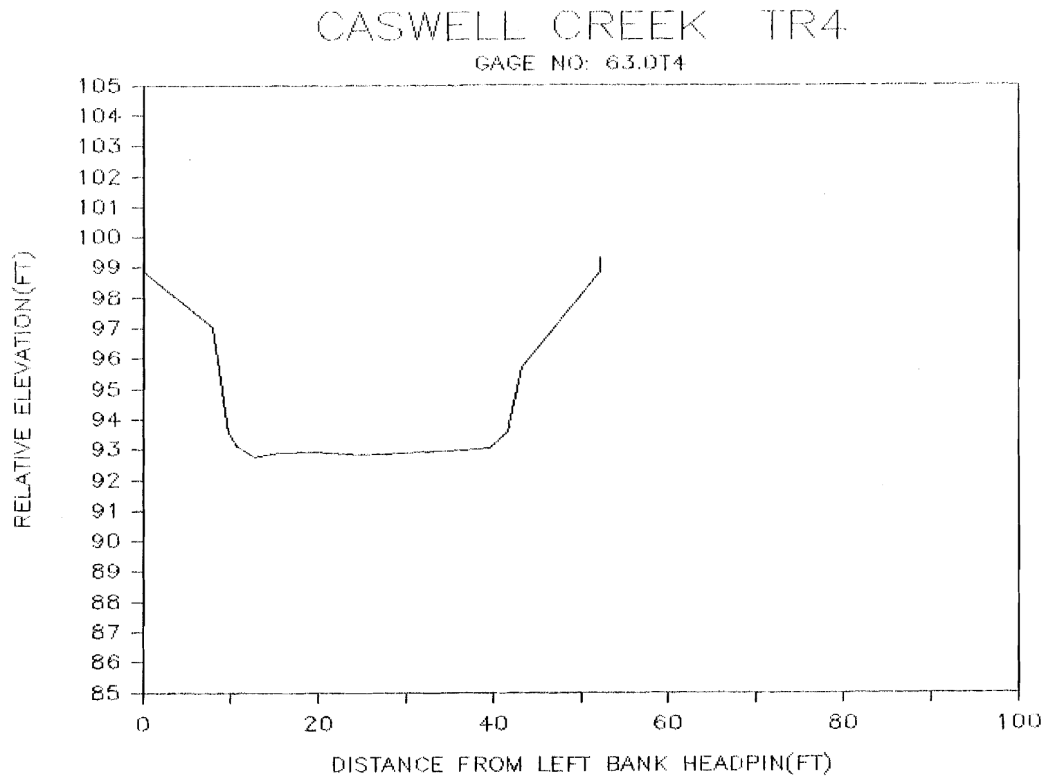
Attachment Figure D- 8. Cross sectional profile obtained at transect 4 of Caswell Creek.
