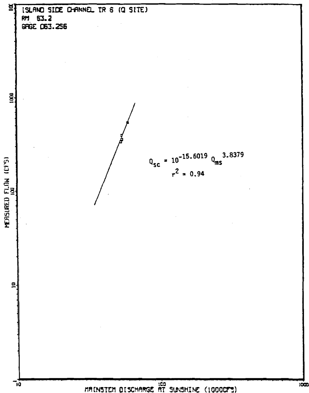
Figure 33. Island Side Channel streamflow versus mainstem discharge at Sunshine Station (USGS 15292780) rating curve at transect 6 Q Site.
