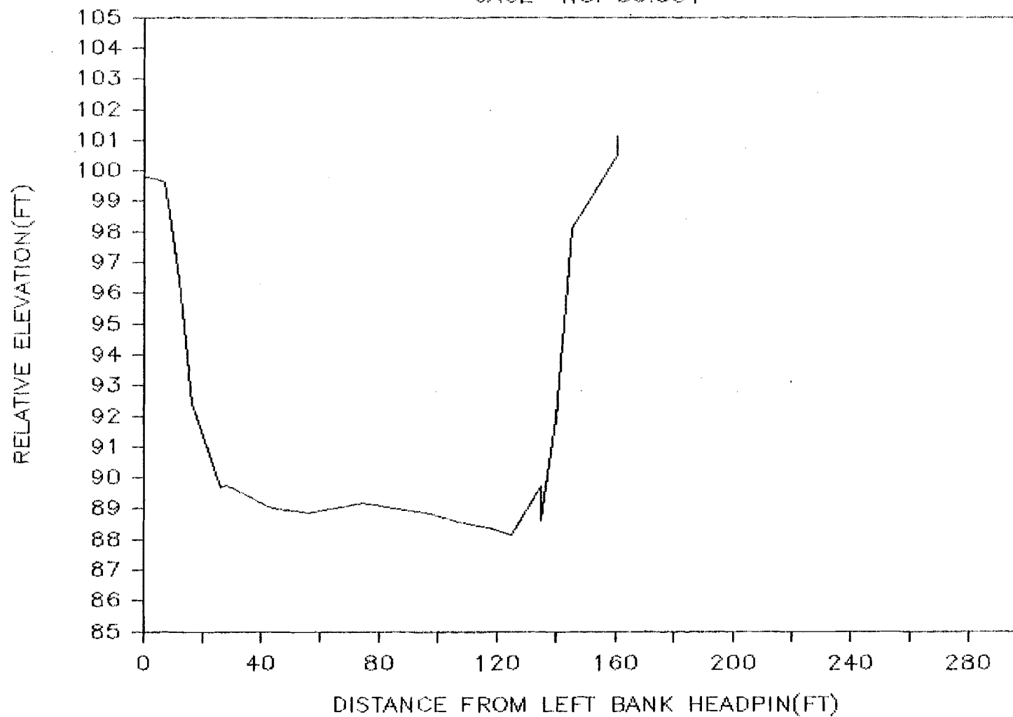
Attachment Figure D-3. Cross sectional profile obtained at transect 2 of Kroto Slough Head.
