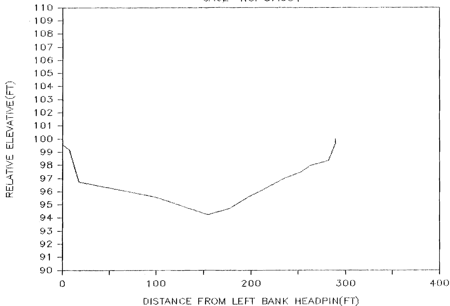
Attachment Figure D- 46. Cross sectional profile obtained at transect 4 of Sunrise Side Channel.
