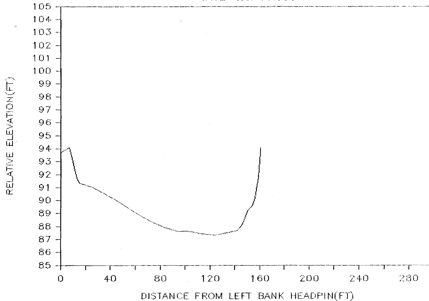
Attachment Figure D-25. Cross sectional profile obtained at transect 1 of Circular Side Channel.
