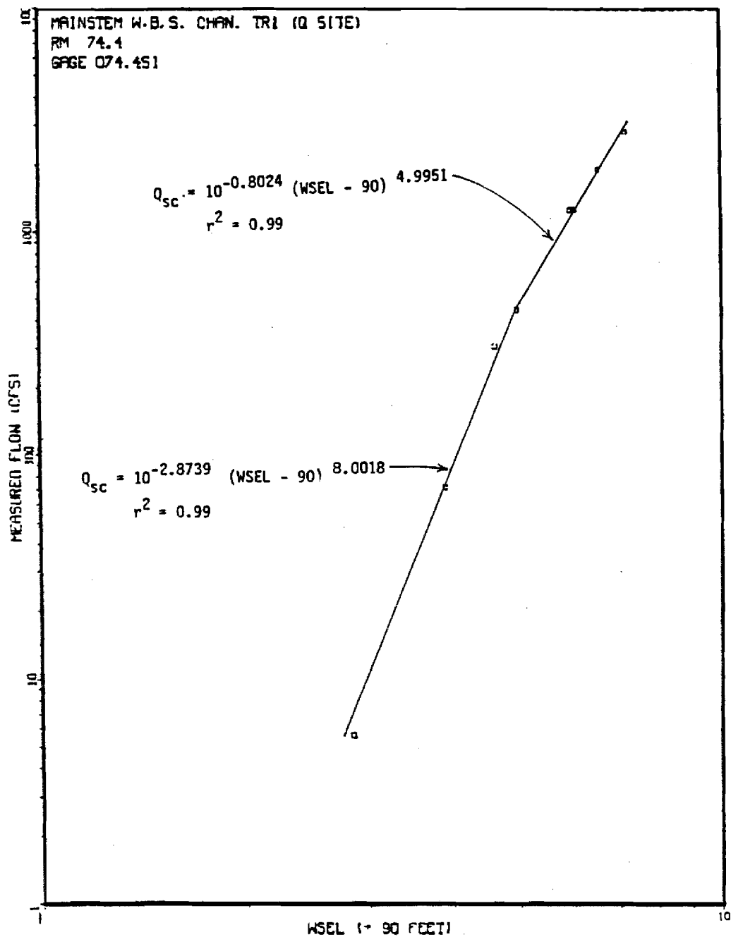
Figure 37. Mainstem West Bank Side Channel streamflow versus WSEL rating curve at transect 1 Q Site.
