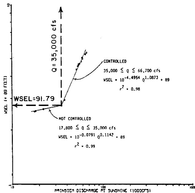
Figure 34. Comparison of rating curves for Island Side Channel transect 6 Q Site.
