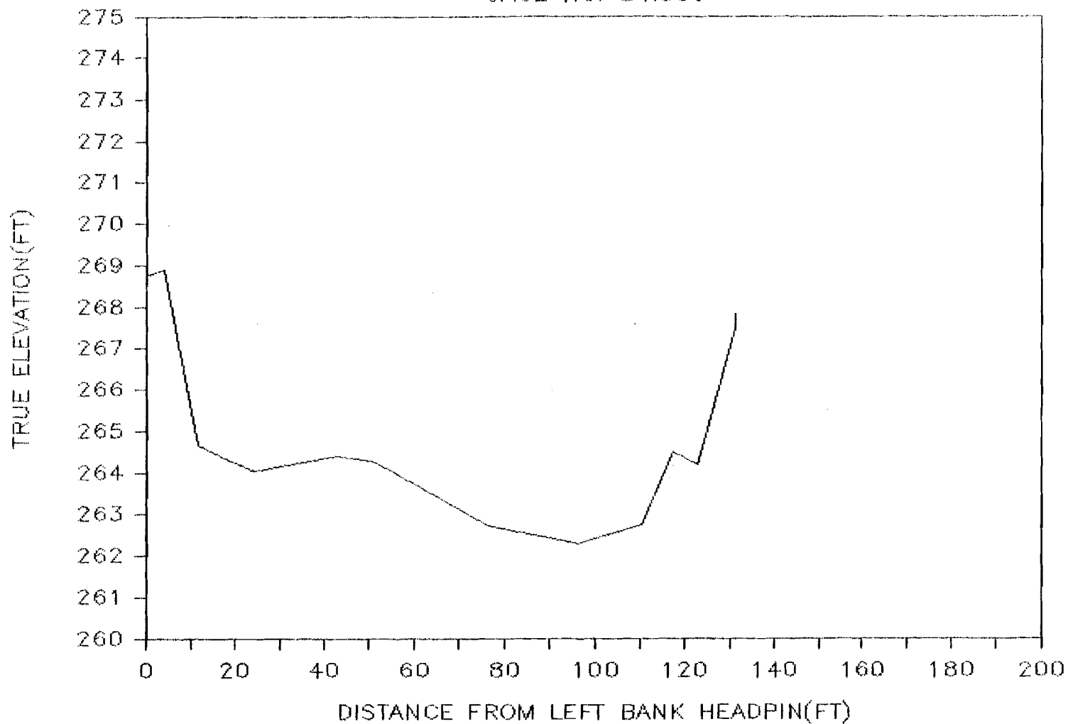
Attachment Figure D-36. Cross sectional profile obtained at transect 5 of Sucker Side Channel.
