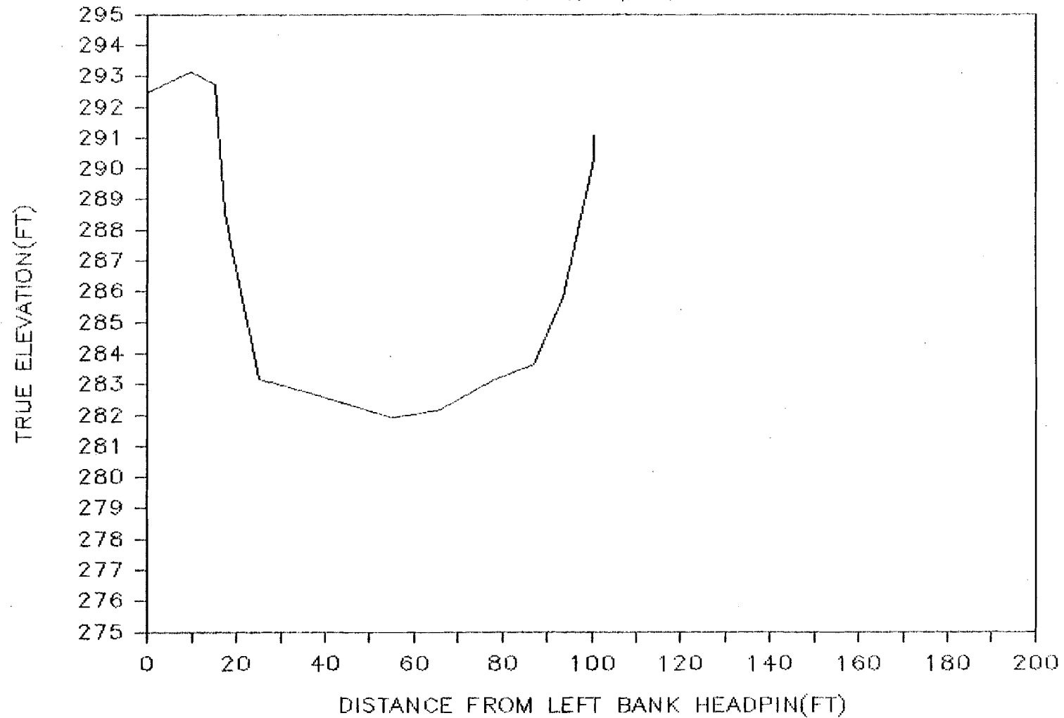
Attachment Figure D- 47. Cross sectional profile obtained at transect 2 of Birch Creek Slough.
