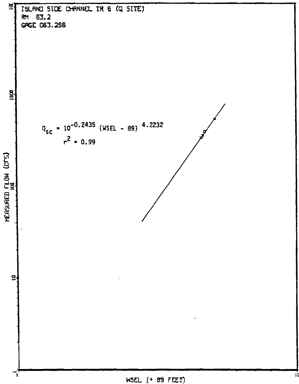
Figure 31. Island Side Channel streamflow versus WSEL rating curve at transect 6 Q Site.
