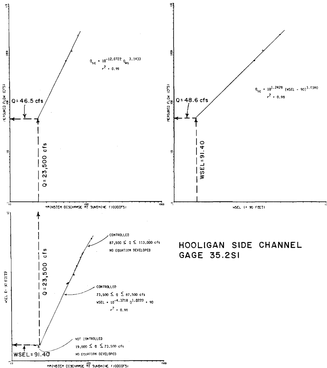
Figure 6. Comparison of rating curves for Hooligan Side Channel Q site located 50 feet upstream from transect 3.
