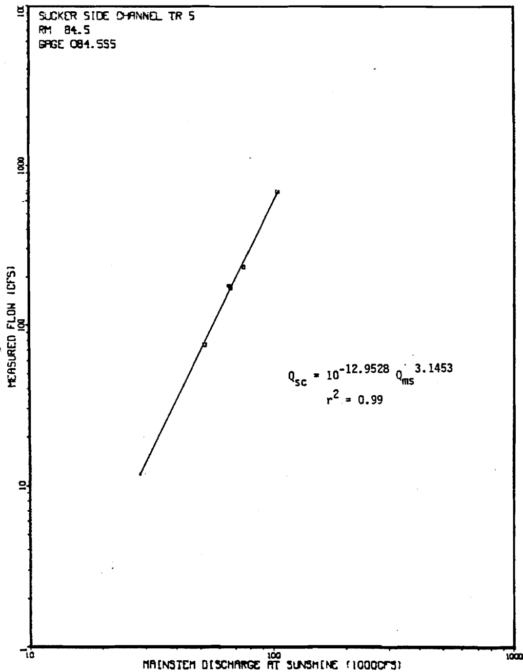
Figure 61. Sucker Side Channel streamflow versus mainstem discharge at Sunshine Station (USGS 15292780) rating curve at transect 5 Q Site.
