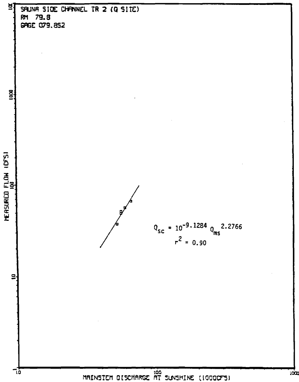
Figure 54. Sauna Side Channel streamflow versus mainstem discharge at Sunshine Station (USGS 15292780) rating curve at transect 2 Q Site.
