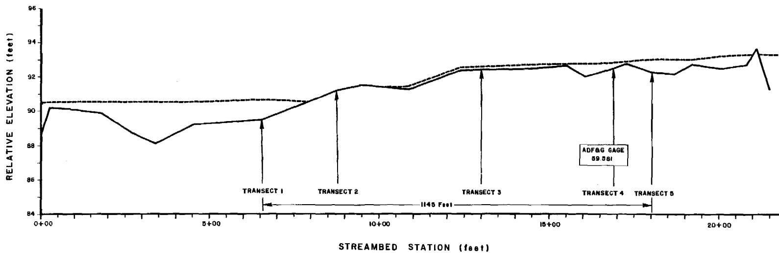
Attachment Figure C-7. Thalweg profile of the study site at Rustic Wilderness Side Channel.
