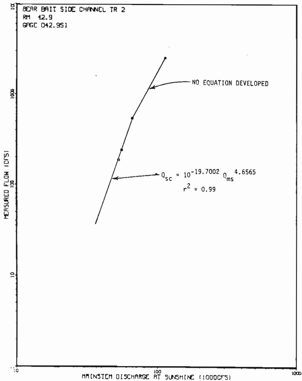
Figure 18. Bear Bait Side Channel streamflow versus mainstem discharge at Sunshine Station (USGS 15292780) rating curve at transect 2 Q Site.
