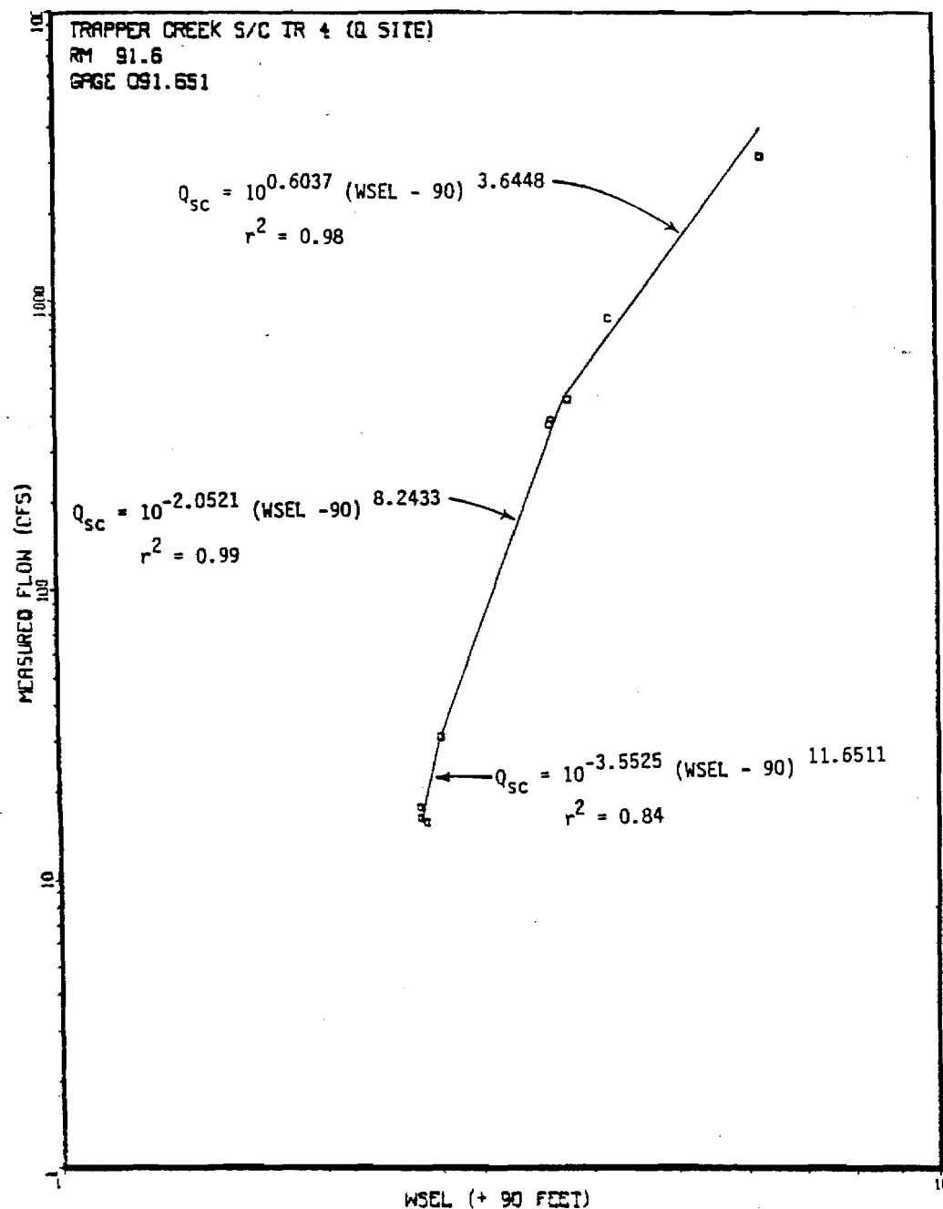
Figure 83. Trapper Creek Side Channel streamflow versus WSEL rating curve at transect 4 Q Site.
