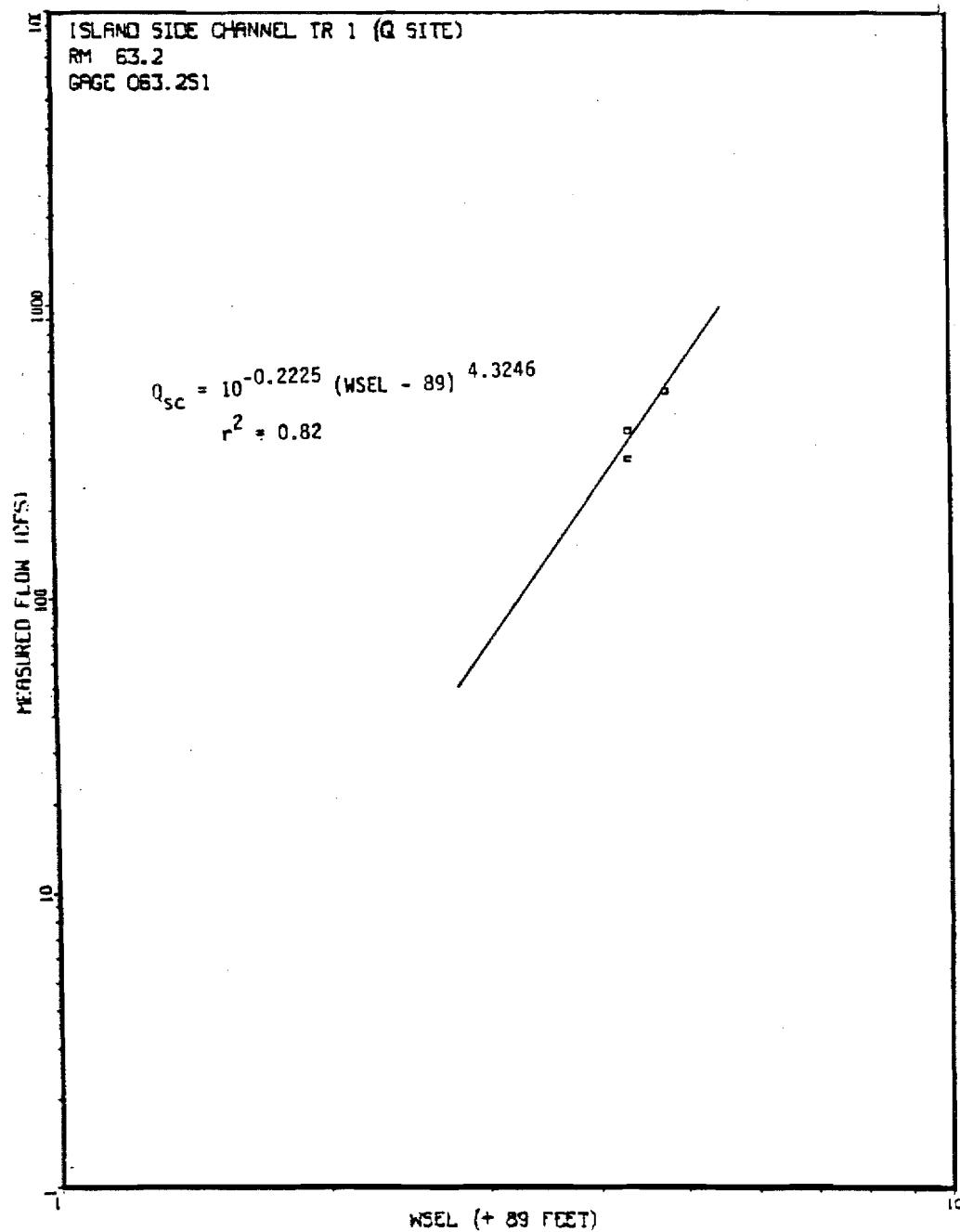
Figure 30. Island Side Channel streamflow versus WSEL rating curve at transect 1 Q Site.
