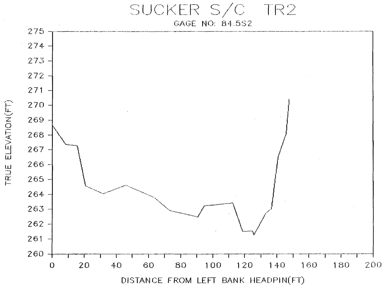
Attachment Figure D-35. Cross sectional profile obtained at transect 2 of Sucker Side Channel.
