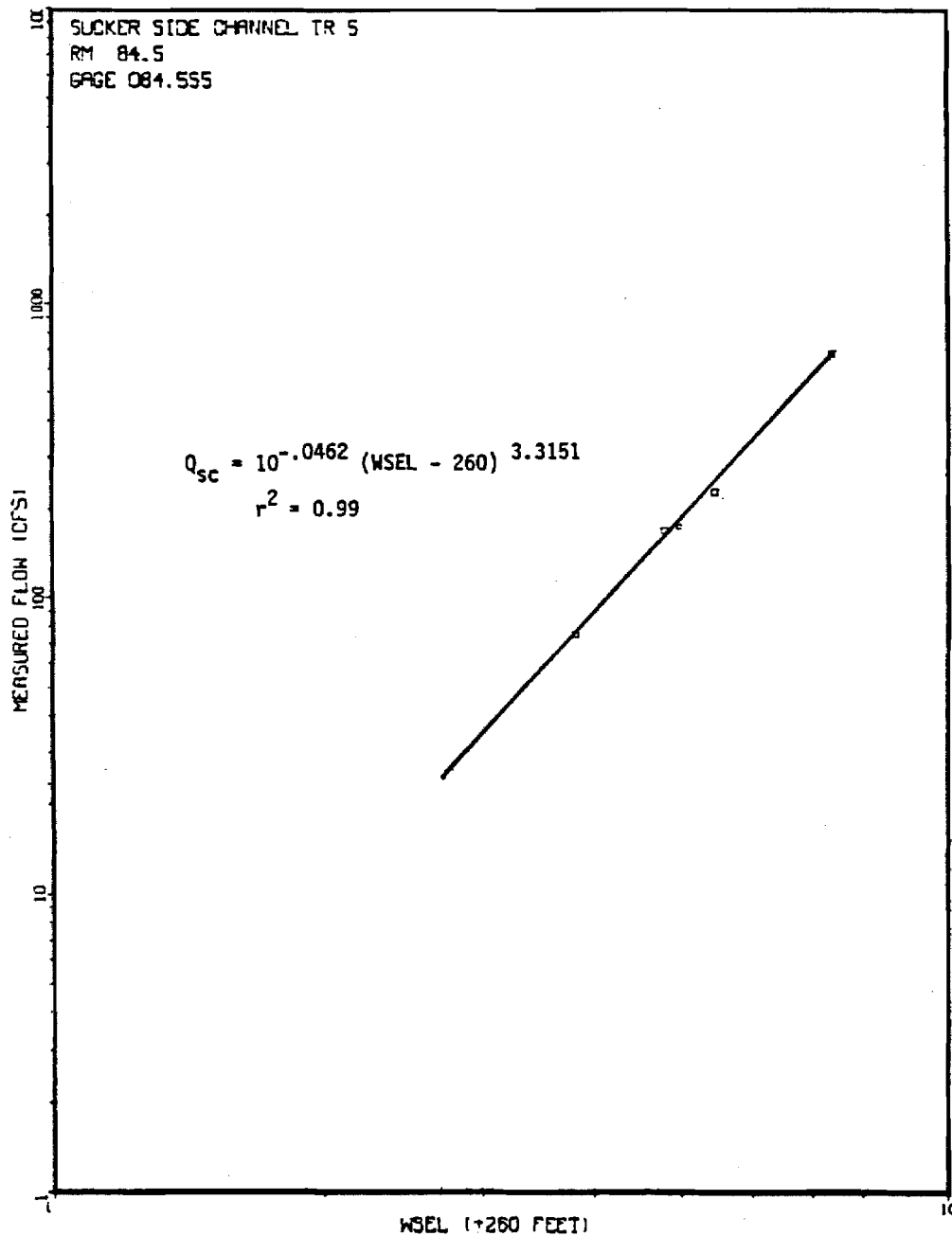
Figure 59. Sucker Side Channel streamflow versus WSEL rating curve at transect 5 Q Site.
