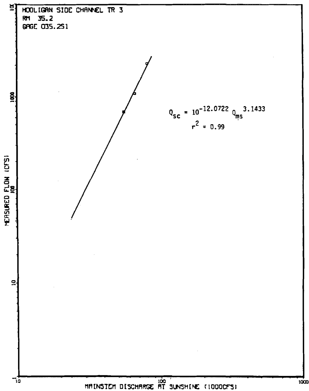
Figure 5. Hooligan Side Channel streamflow versus mainstem discharge at Sunshine Station (USGS 15292780) rating curve from Q site located 50 feet upstream from transect 3.
