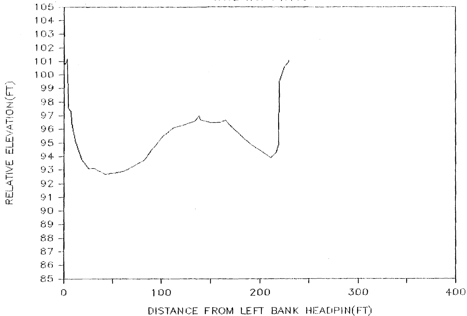
Attachment Figure D- 20. Cross sectional profile obtained at transect 3 of Mainstem West Bank Side Channel.
