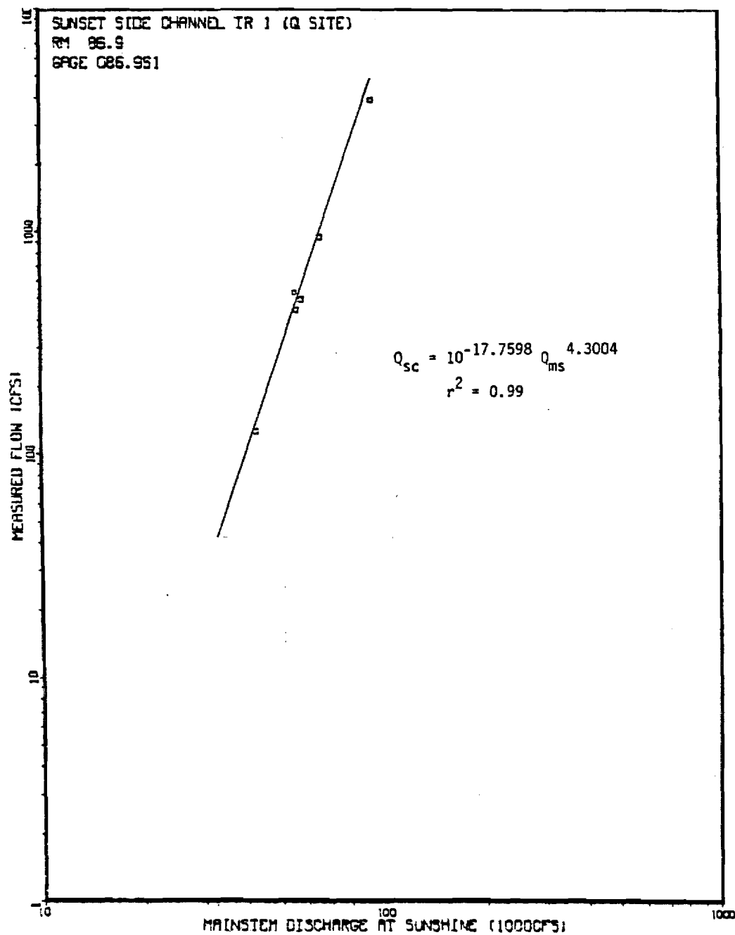
Figure 72. Sunset Side Channel streamflow versus mainstem discharge at Sunshine (USGS 15292780) rating curve at transect 1 Q Site.
