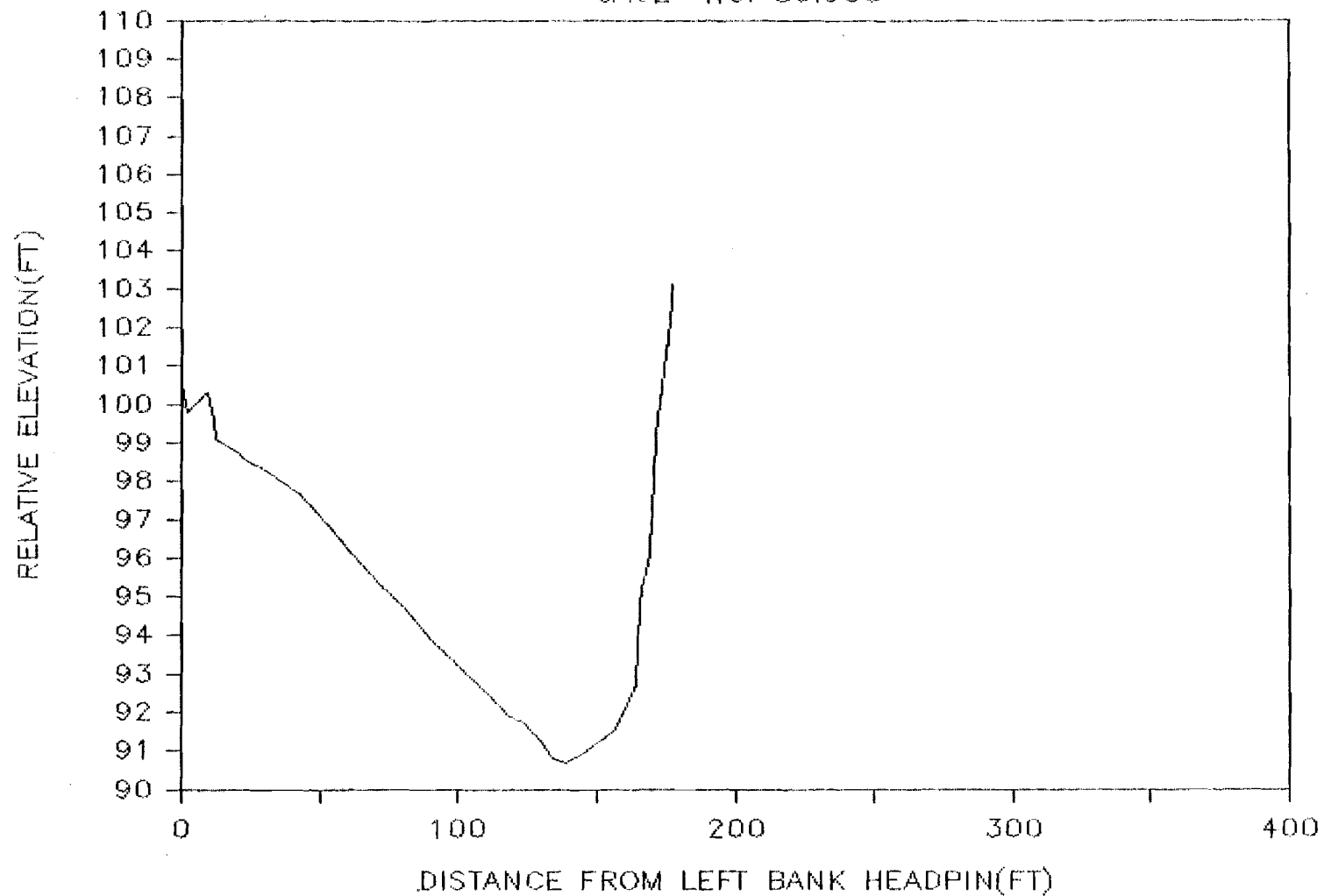
Attachment Figure D-45. Cross sectional profile obtained at transect 6 of Sunset Side Channel.
