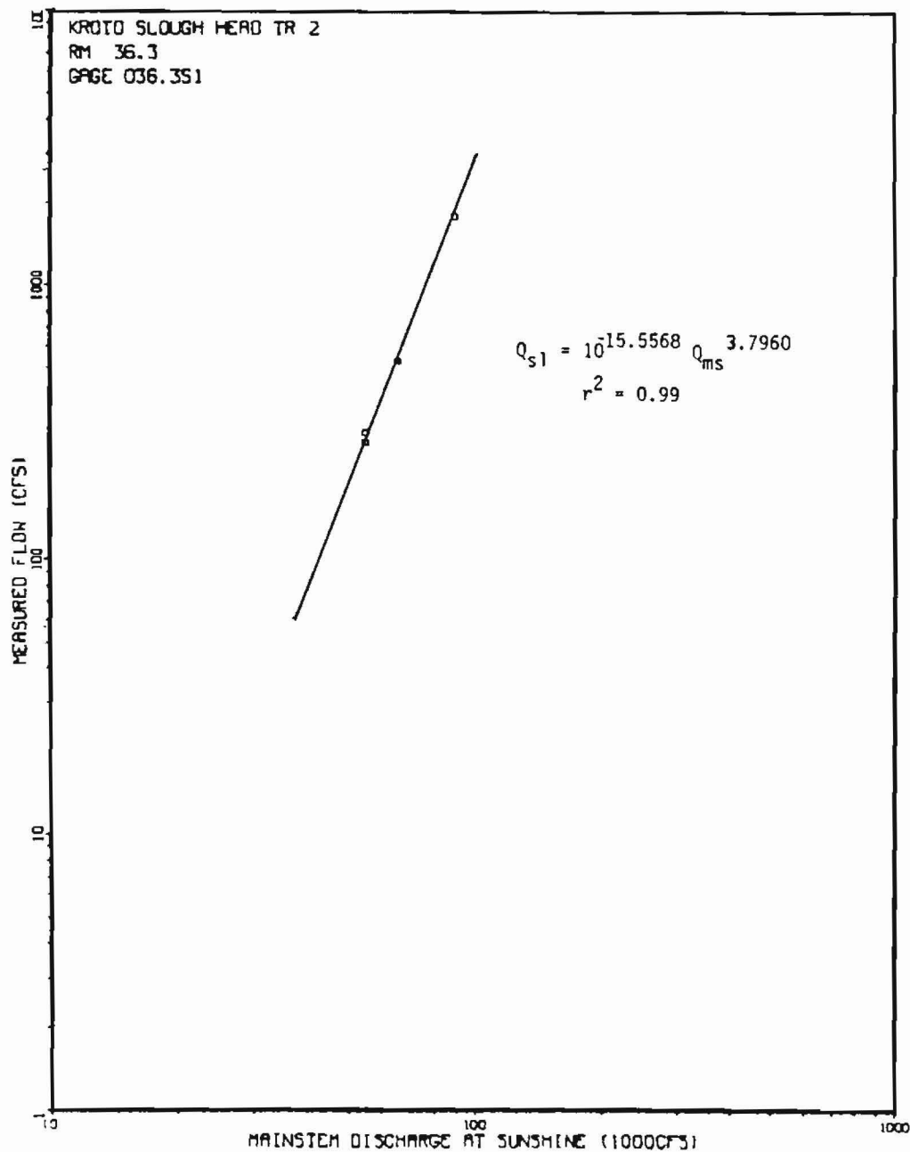
Figure 11. Kroto Slough Head streamflow versus mainstem discharge (cfs) at Sunshine Station (USGS 15292780) rating curve at transect 2 Q site.
