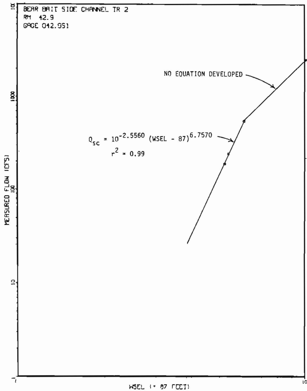
Figure 17. Bear Bait Side Channel streamflow versus WSEL rating curve at transect 2 Q Site.
